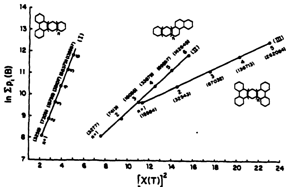
Fig. 4. Correlation between total number of self-avoiding paths, 19 \Sigma p(B) , (numbers of parentheses) of families of benzenoid hydrocarbons and [\chi(T)]^2 , the squares of connectivity indices of the equivalent trees.
