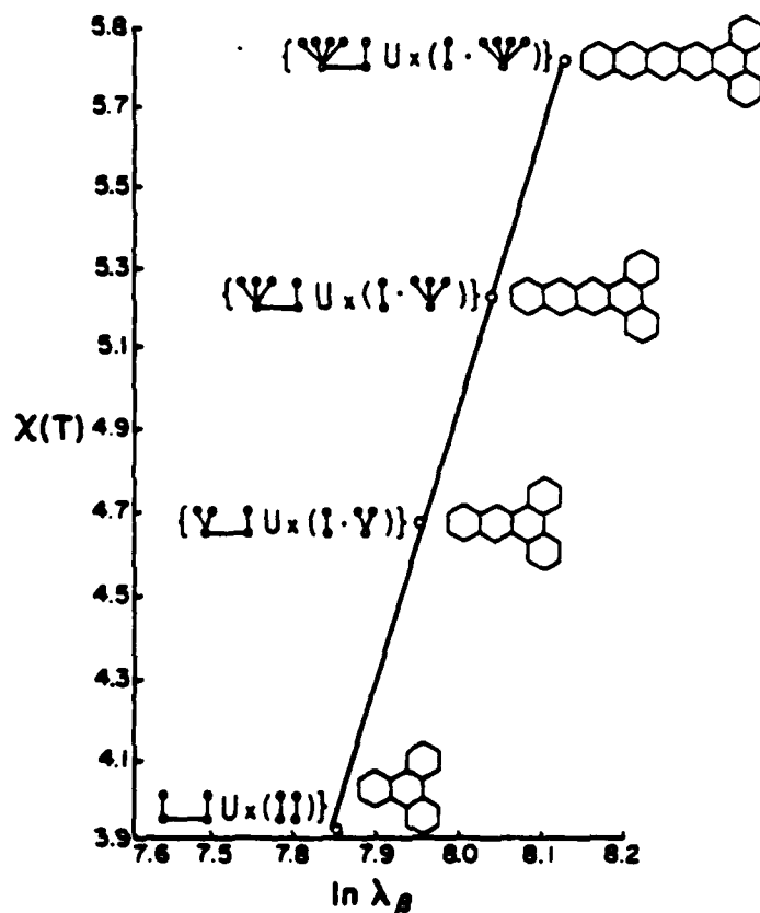
Fig. 3. A plot of electronic absorption \lambda_B , for a series of branched benzenoids 18 and the connectivity indices of a series of disconnected trees, (T) .
