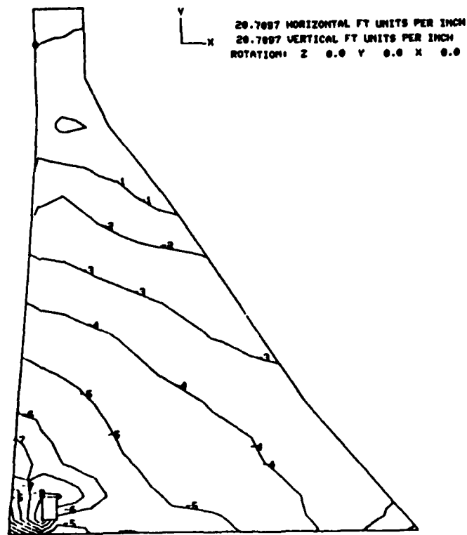
Figure 13. S_{xx} stresses
