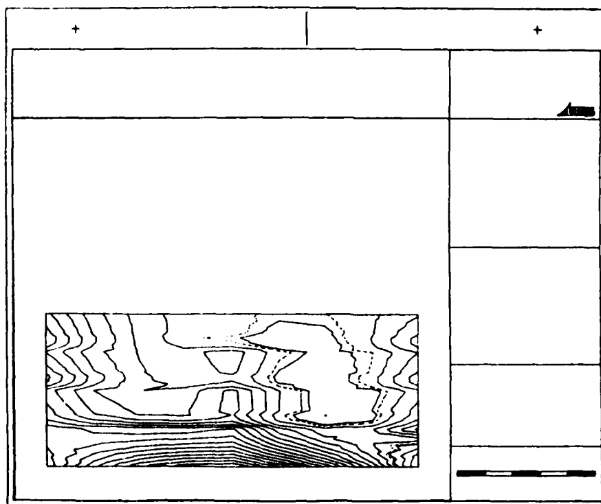
Figure G24. Nonannotated, Y-direction principal stress contours grid I, N = 4, P-level 2
