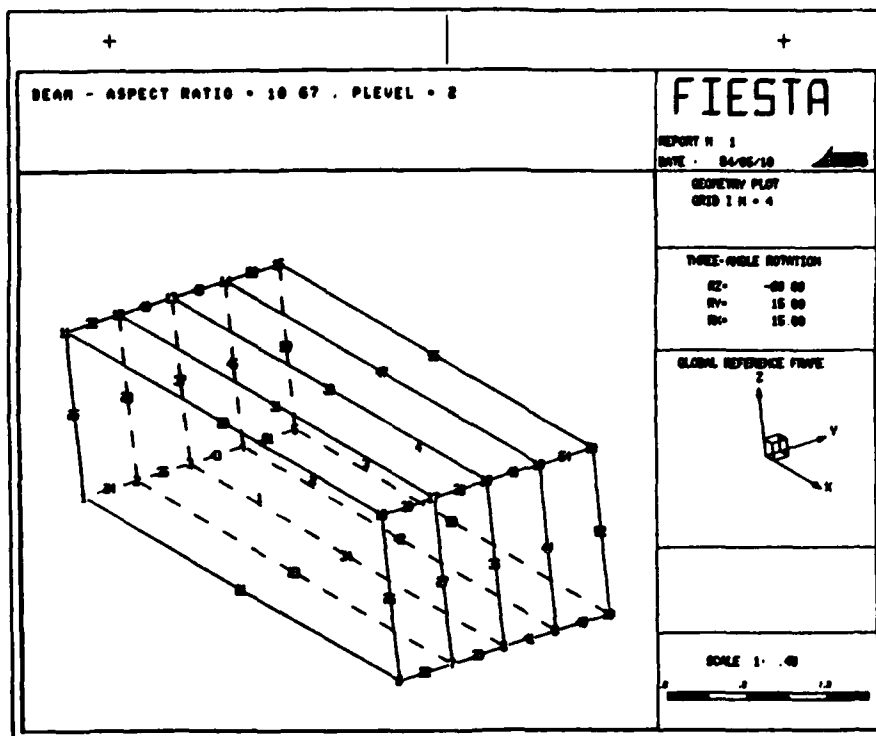
Figure G19. Annotated geometry plot grid I, N = 4 , P-level 2
