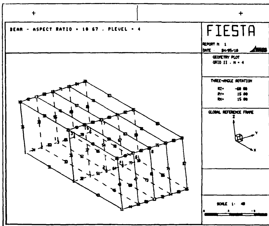
Figure G36. Annotated geometry plot grid II, N = 4 , P-level 4
