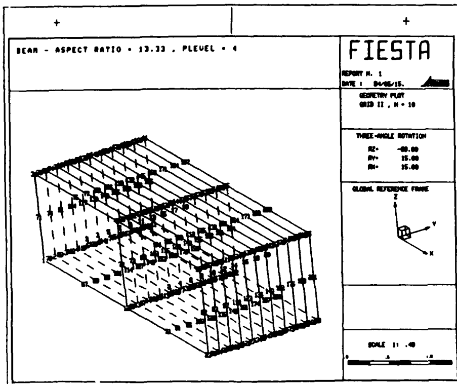
Figure G54. Annotated geometry plot grid II, N = 10 , P-level 4
