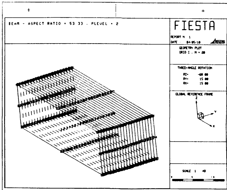
Figure G58. Annotated geometry plot grid I, N = 20 , P-level 2
