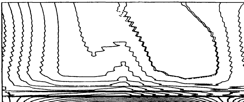
Figure G63. Nonannotated window of Y-direction principal stress contours grid I, N = 20 , P-level 2
