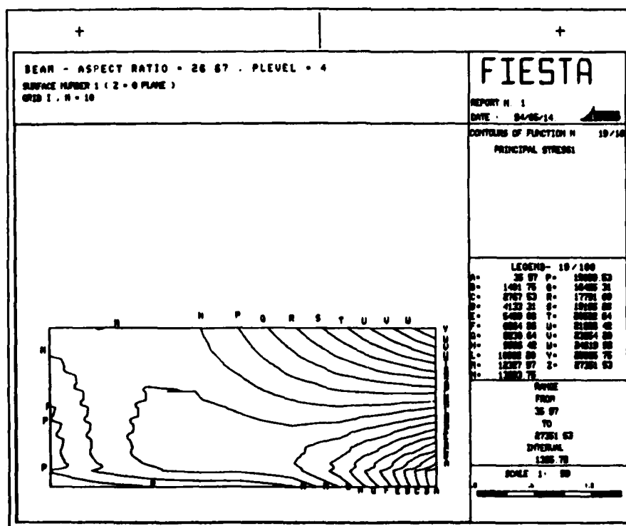
Figure G48. Annotated, X-direction principal stress contours grid I, N = 10 , P-level 4
