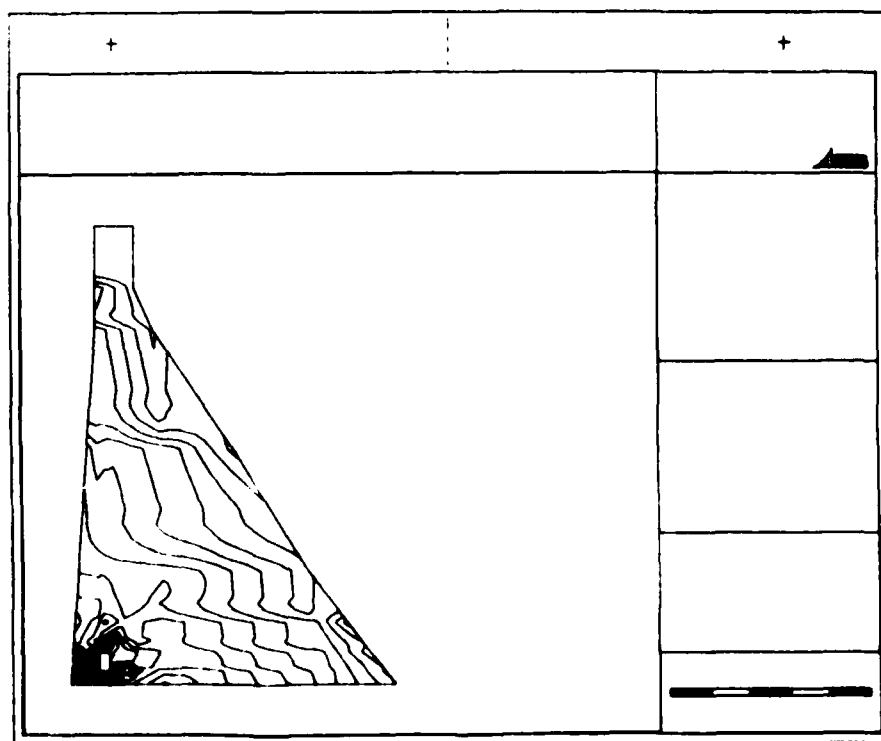
Figure 89. Nonannotated plot of Y-direction principal stress contours, fine grid, P-level 1
