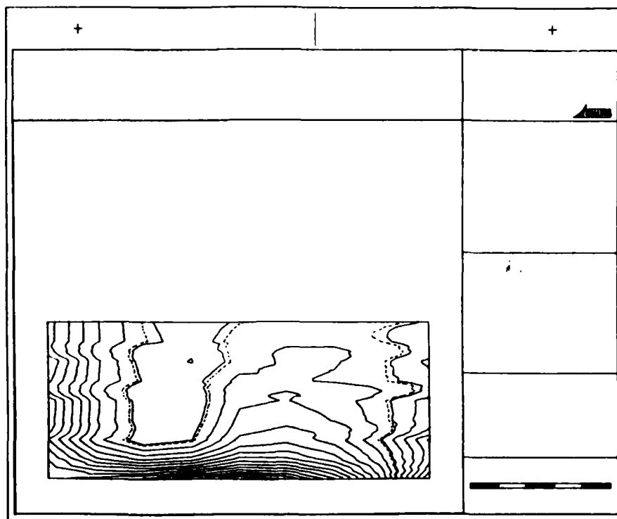
Figure G29. Nonannotated, Y-direction principal stress contours grid I, N = 4 , P-level 4
