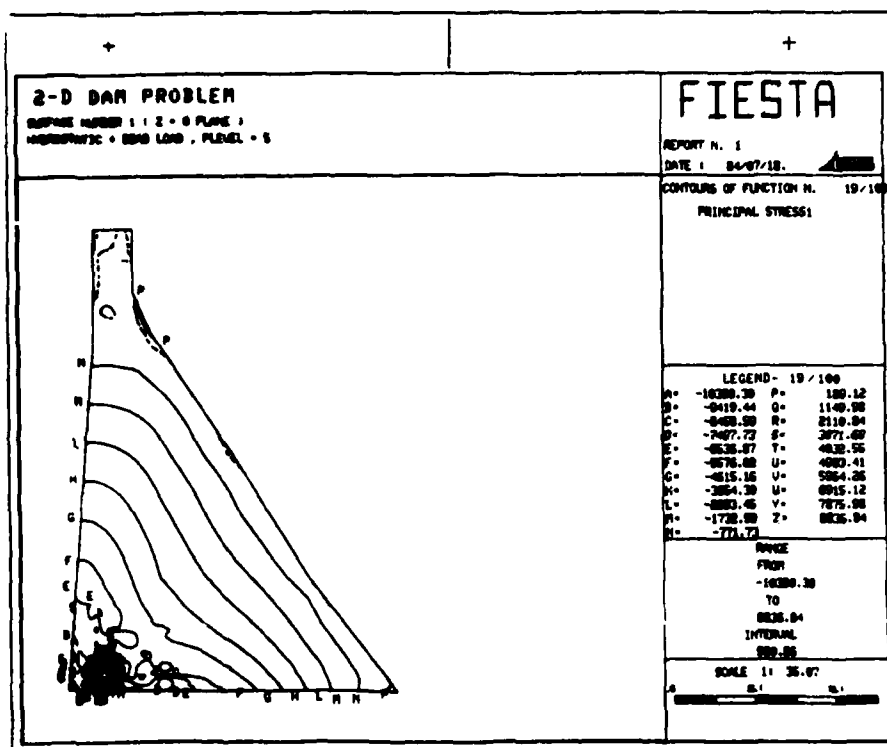
Figure B26. Window plot of annotated, X-direction principal stress contours, fine grid, P-level 5
