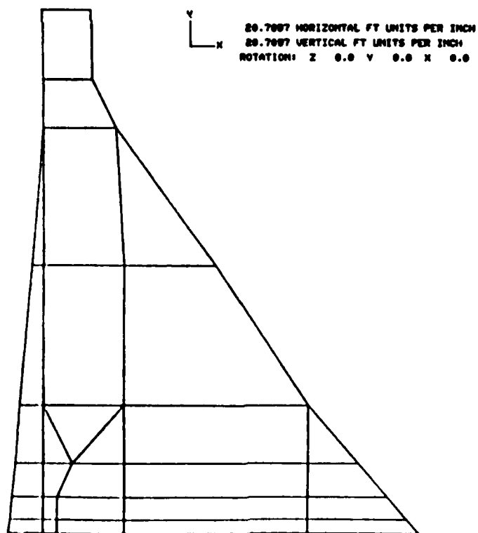
Figure 11. GTSTRU DL Model 2
