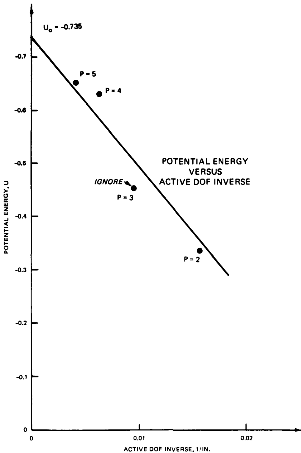
Figure 21. Thin plate, 100-psf uniform load
