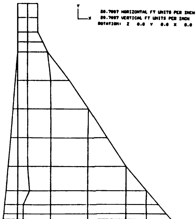
Figure 10. GTSTRU DL Model 1
