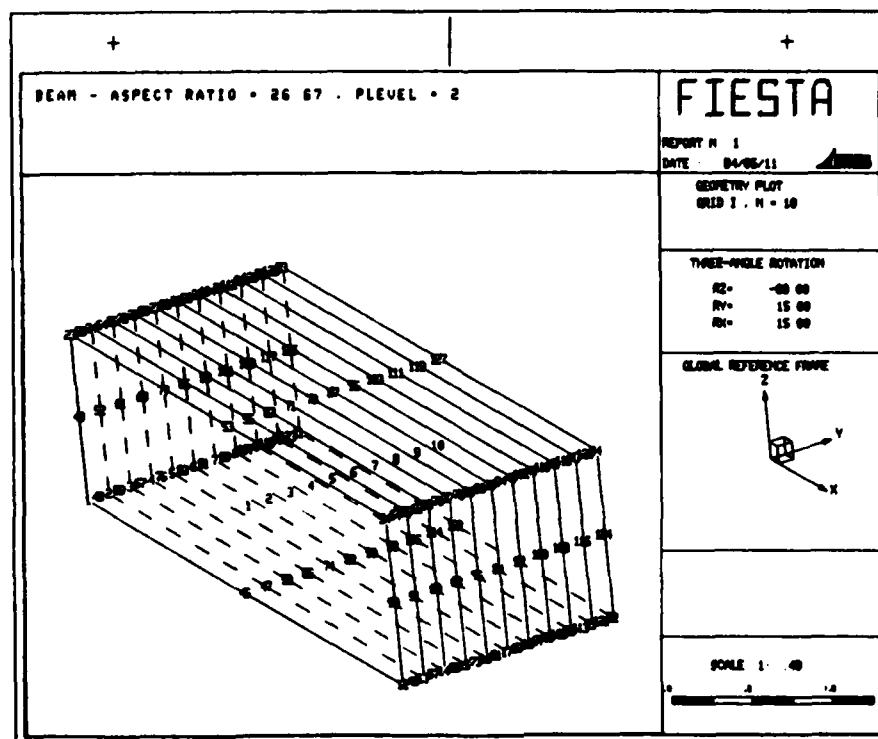
Figure G42. Annotated geometry plot grid I, N = 10 , P-level 2
