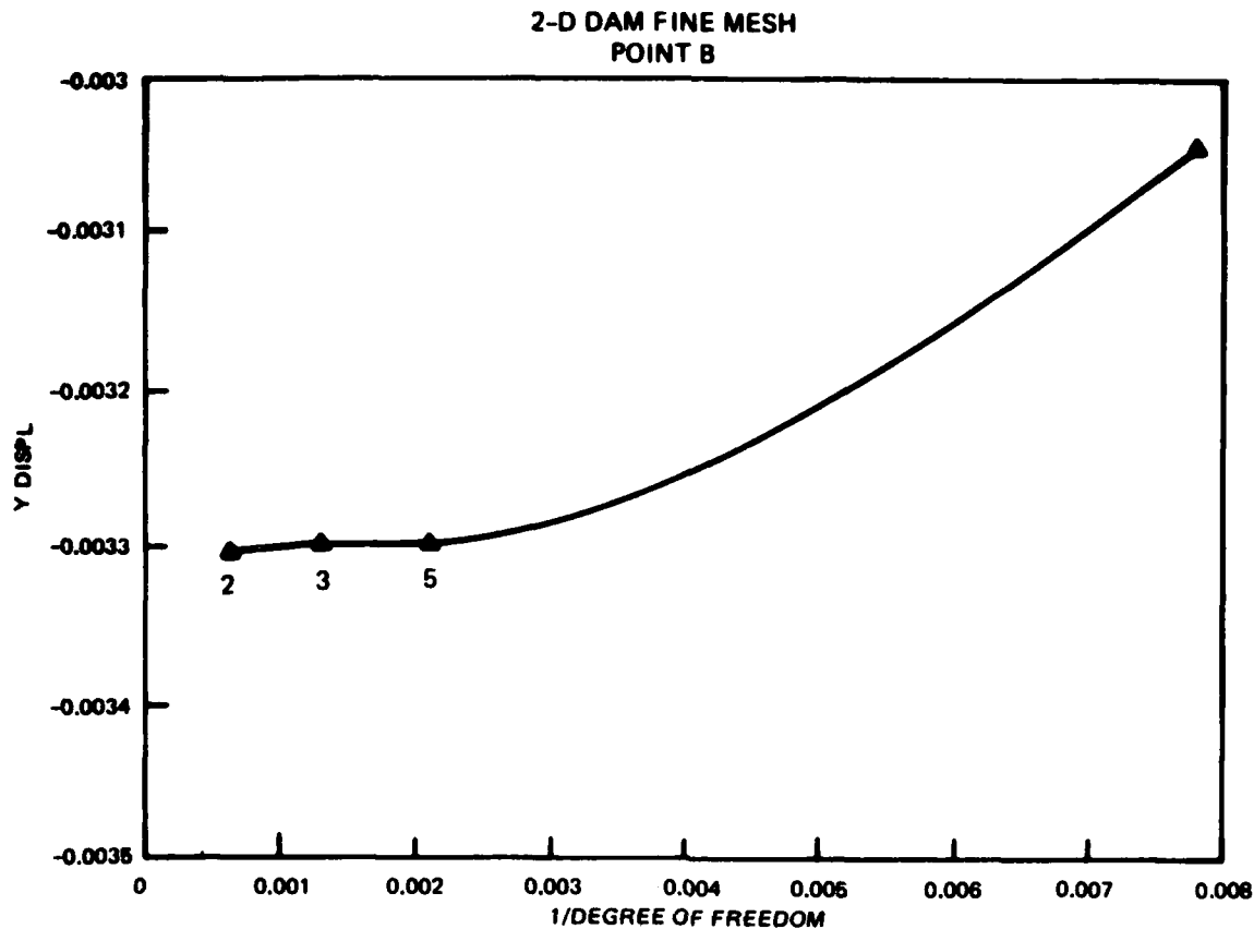
Figure 9. Vertical displacement at point B
