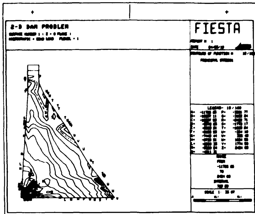
Figure B4. Annotated plot of X-direction principal stress contours, fine grid, P-level 1
