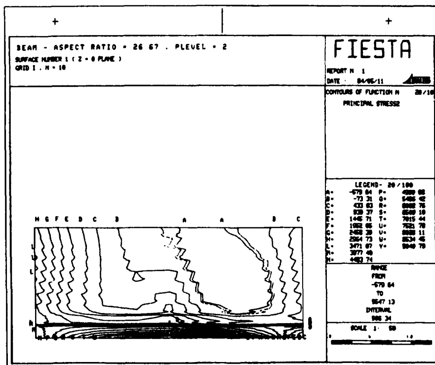
Figure G46. Annotated, Y-direction principal stress contours grid I, N = 10, P-level 2
