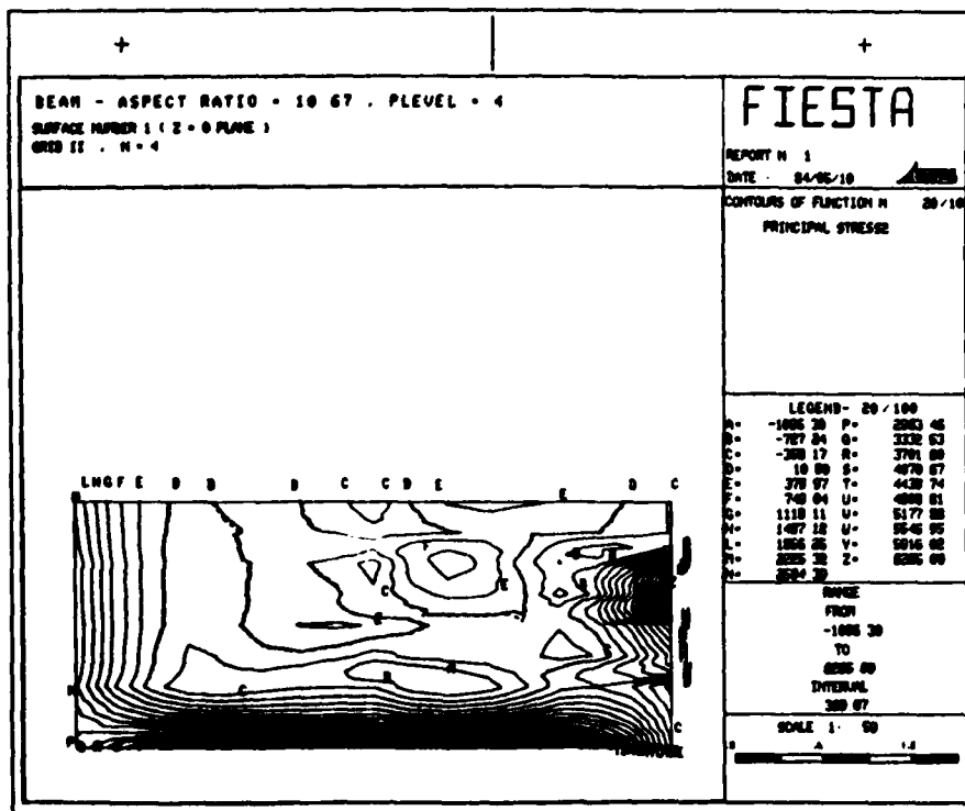
Figure G39. Annotated, Y-direction principal stress contours grid II, N = 4, P-level 4
