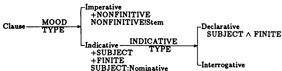
Figure 11: MoodType and IndicativeType Realizations
