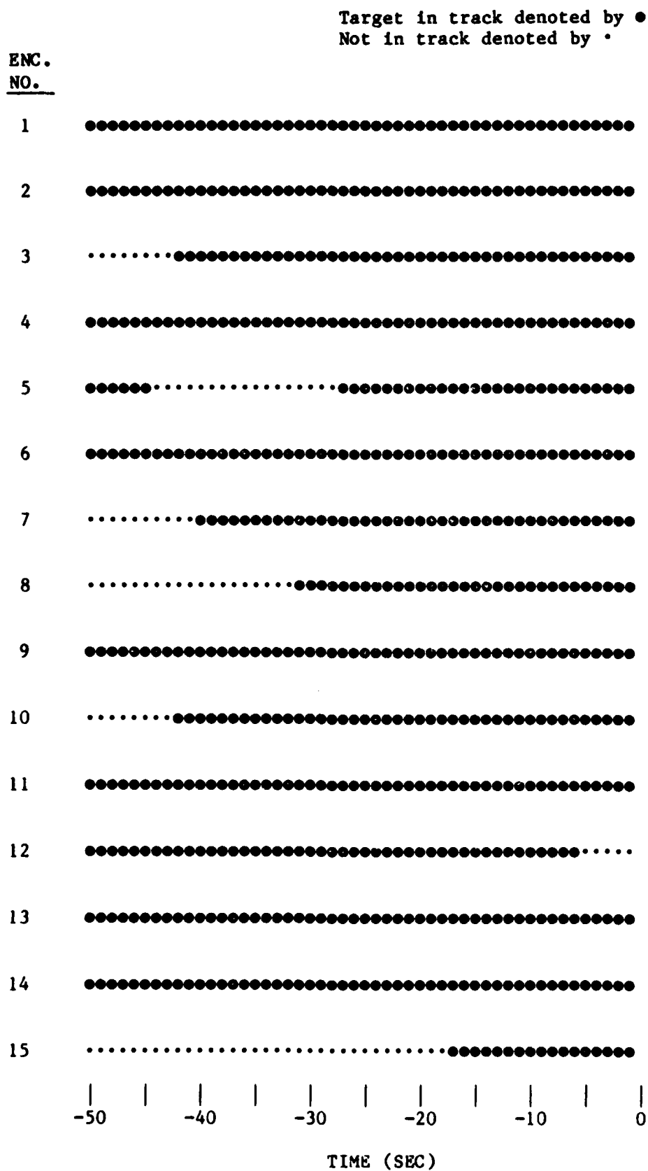
Fig. 3-10. TCAS air-air surveillance during 15 close encounters in New York.
