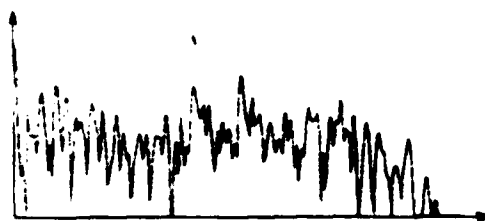
Fig. 2.3(g) - Synthetic Spectrum
