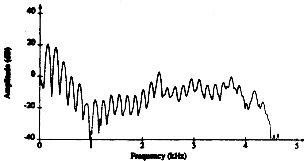
Figure 1.2: Spectrum of a /l/ Phoneme
