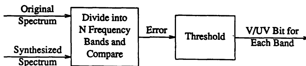
Figure 5.13: Coding of V/UV Information
