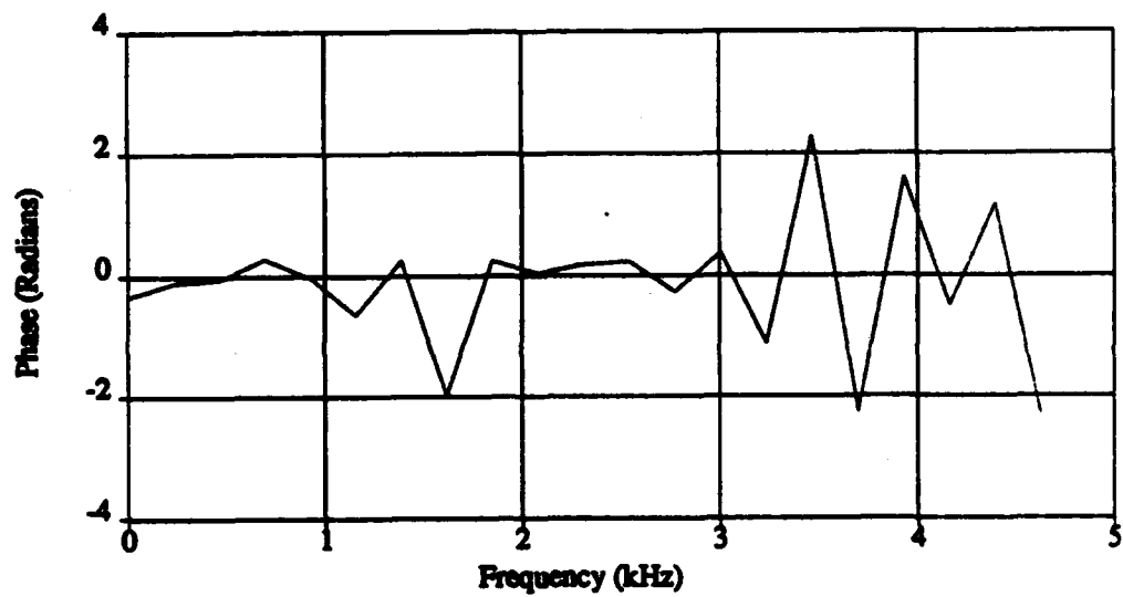
Figure 5.5: Difference Between Estimated and Predicted Phases
