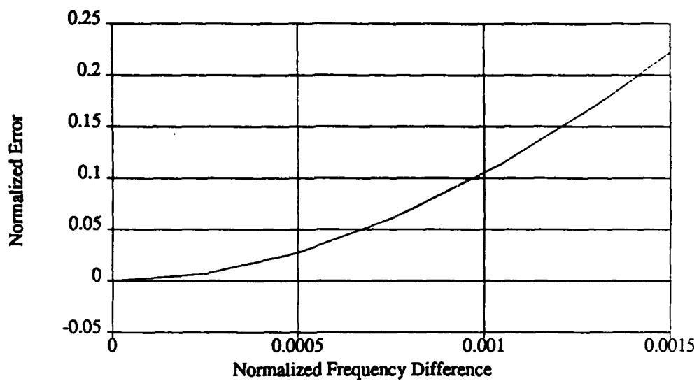
Figure 3.6: Normalized Error Versus Normalized Frequency Difference
