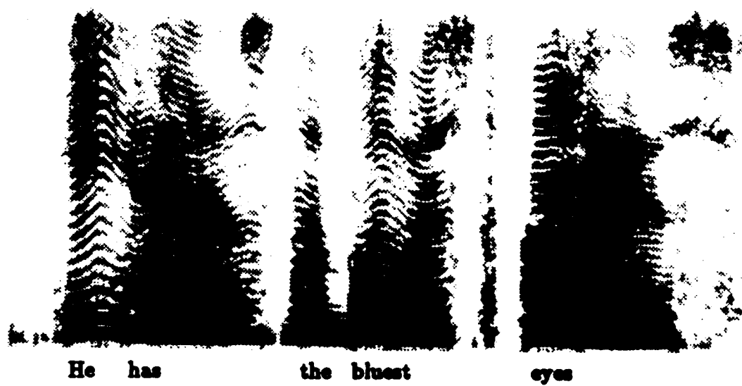
Figure 5.16: SBE Vocoder - Clean Speech Spectrogram
