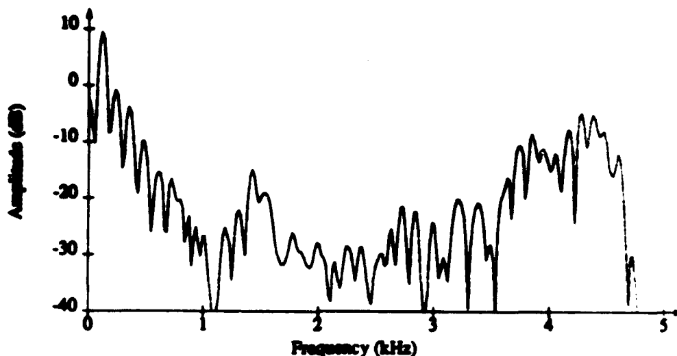
Figure 1.1: Spectrum of a /s/ Phoneme
