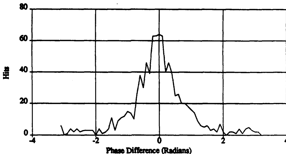
Figure 5.9: Phase Difference Histogram (1.0 - 1.5kHz)
