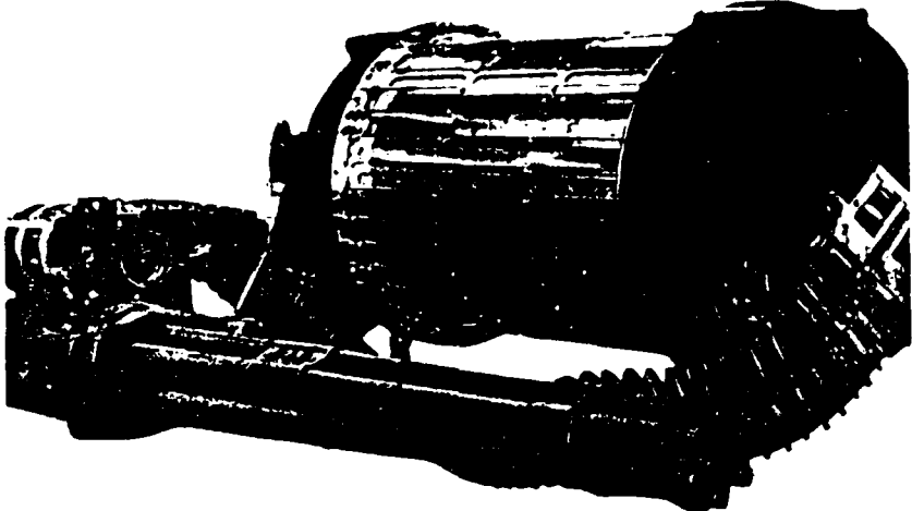
FIGURE 6. M-61A1 Vulcan With Rotary Drum Linkless Feed System (Air Force Photo)
