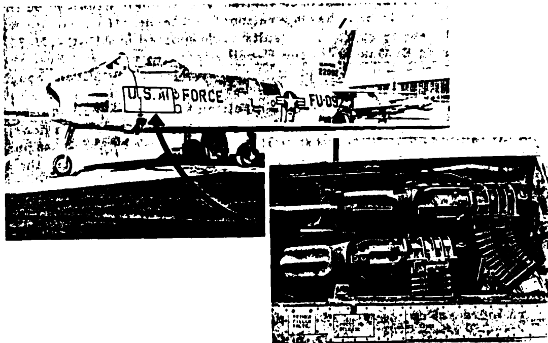
FIGURE 2. F-86 Aircraft With M-39 Installed. (Air Force Photo)
