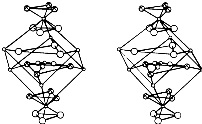
Figure 2. ORTEP stereoview of the structure of \text{OD}_3\text{SbF}_6 . The bridging \text{F}_2 atoms are differentiated from the nonbridging \text{F}_1 atoms by smaller circles marked by traces.
