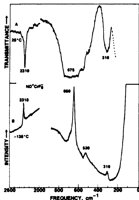
Figure 2. Vibrational spectra of solid NOCrF 6 : trace A, infrared spectrum of the powder pressed between AgBr disks; trace B, low-temperature Raman spectrum.
