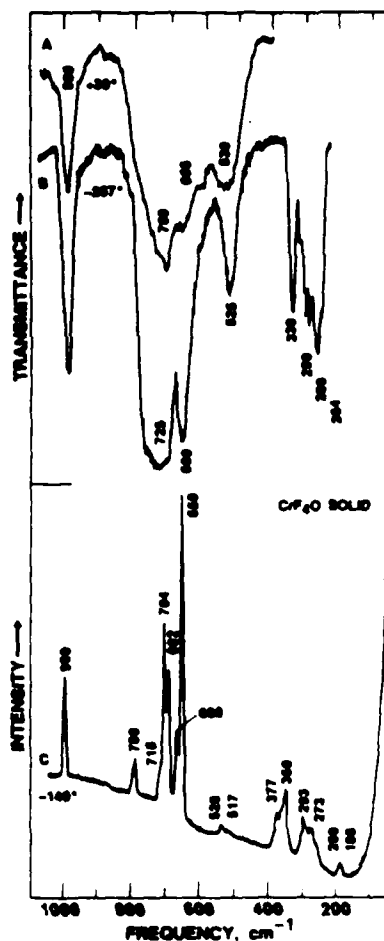
Figure 3. Vibrational spectra of solid \text{CrF}_5\text{O} : (A) infrared spectrum of the solid between \text{AgCl} disks at room temperature; (B) infrared spectrum of the solid at 6\text{ K} on a \text{CsI} window; (C) Raman spectrum of the solid in a quartz tube recorded at -140^\circ\text{C} with 647.1\text{-nm} excitation
