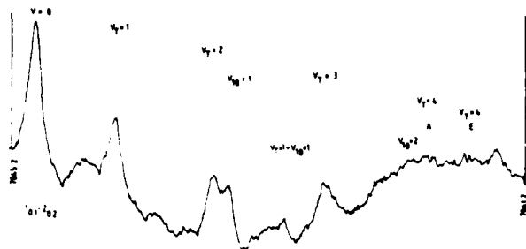
Figure 5. The J = 1_{01} \rightarrow 2_{02} transitions at a Stark field of 800 V/cm. Marker spacing is 0.8 MHz. The assignment of v_{15} = 4 is speculative, although other J candidates for the A components have been located.
