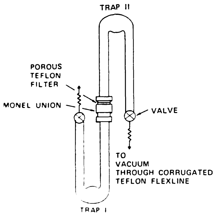
Fig. 2. Metathesis apparatus for [\text{NF}_4][\text{HF}] , [\text{NF}_4][\text{MnF}_6] , [\text{NF}_4][\text{SiF}_6] , and
