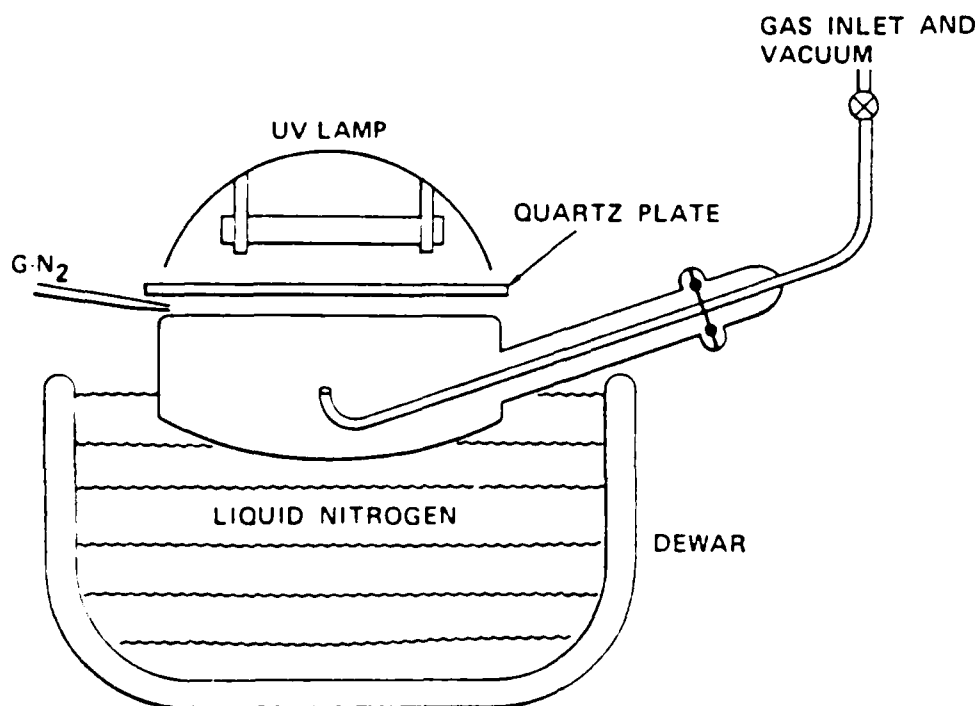
Fig. 1 Apparatus for synthesis of [\text{NF}_4][\text{BF}_4] .
