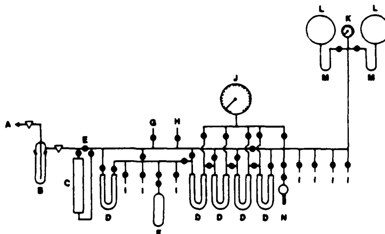
Fig. 1. Typical metal-Teflon vacuum system used for handling strongly oxidizing or corrosive fluorine compounds. As the vacuum source A, a good mechanical pump ( 10^{-4} torr or better) is normally sufficient. The use of a fluorocarbon oil, such as Halocarbon [Halocarbon Products] as a pump oil is strongly recommended for safety reasons. B, glass waste trap with glass or Teflon stopcocks and a detachable bottom; only fluorocarbon grease [Halocarbon Products] should be used for the stopcocks and joint; the trap is kept cold by a Dewar flask with liquid nitrogen; great care must be taken, and a face shield and heavy leather gloves must be worn when pulling off the cold lower half of the waste trap for disposal of the trapped material by evaporation in a fume hood. The glass waste trap can be connected to the metal line by a glass-metal joint, a graded glass-metal seal, or most conveniently by a quick-coupling compression fitting with Viton O-ring seals. C, scrubber for removal of fluorine; the scrubber consists of a glass tower packed with alternating layers of NaCl and soda lime that are held in place by plugs of glass wool at either end. The valves E are arranged in such a manner that the scrubber can be bypassed during routine operation. D, Teflon-FEP (fluoro-ethylene-propylene copolymer [Zeus]) or PFA (polyperfluoroether) U-traps made from \frac{1}{2} - or \frac{3}{8} -in o.d. commercially available heavy wall tubing; all metal lines are made from either 316 or 321 \frac{1}{2} -in o.d. stainless steel or Monel tubing, except for the lines from the U-traps to the Heise gage [Dresser] J, for which \frac{1}{8} -in o.d. tubing is preferred, stainless steel bellows valves E such as Hoke Model 4200 series, are used throughout the entire line, metal-metal or metal-Teflon connections are all made with either flare or compression (Swagelok [Crawford Fitting] or Gyrolok) fittings. F, lecture bottle of ClF 3 , [Ozark-Mahoning] used for passivation of the vacuum line. G, He gas inlet. H, F, gas inlet. I, connectors for attaching reaction vessels, reagent containers, etc. J, Heise Bourdon tube pressure gage (0-1000 mm \pm 0.1%). K, crude pressure gage (0-5 atm). L, 2-L steel bulbs used for either measuring or storing larger amounts of gases. M, \frac{1}{8} -in o.d. metal U-tubes to permit condensation of gases into the storage bulbs. N, infrared cell for gases, Teflon body with condensing tip, 5 cm path length, AgCl windows. The four U-traps D, connected in series, constitute the fractionation train used routinely for the separation of volatile materials by fractional condensation employing slush baths of different temperatures. The volumes of each section of the vacuum line are carefully calibrated by PVT measurements using a known standard volume.
