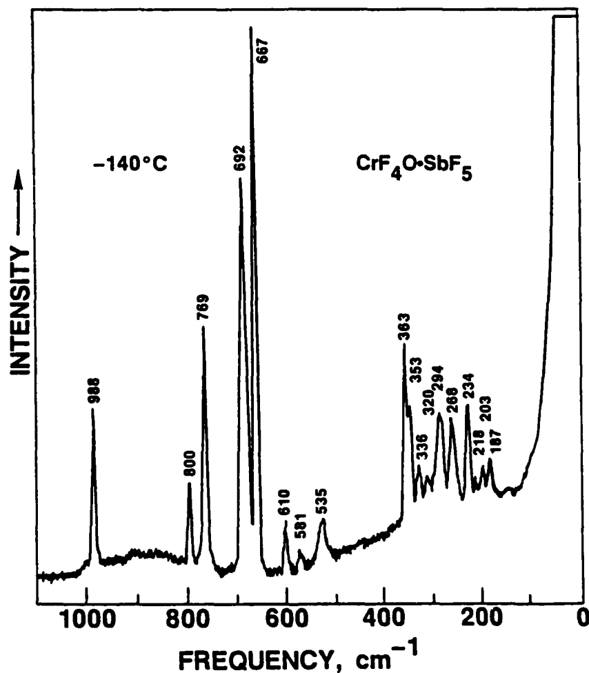
Figure 1. The Raman Spectrum of \text{CrF}_4\text{O}\cdot\text{SbF}_5 at -140^\circ
