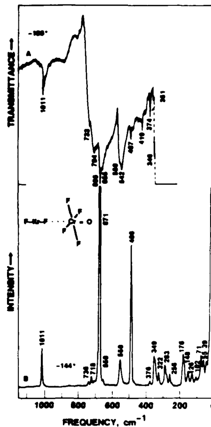
Figure 5. Vibrational spectra of solid KrF 2 -CrF 3 O - : (A) infrared spectrum of the solid between AgCl disks at -196 °C (broken line indicates absorption due to the AgCl window material); (B) Raman spectrum of the solid in a quartz capillary recorded at -144 °C with 647.1-nm excitation.
