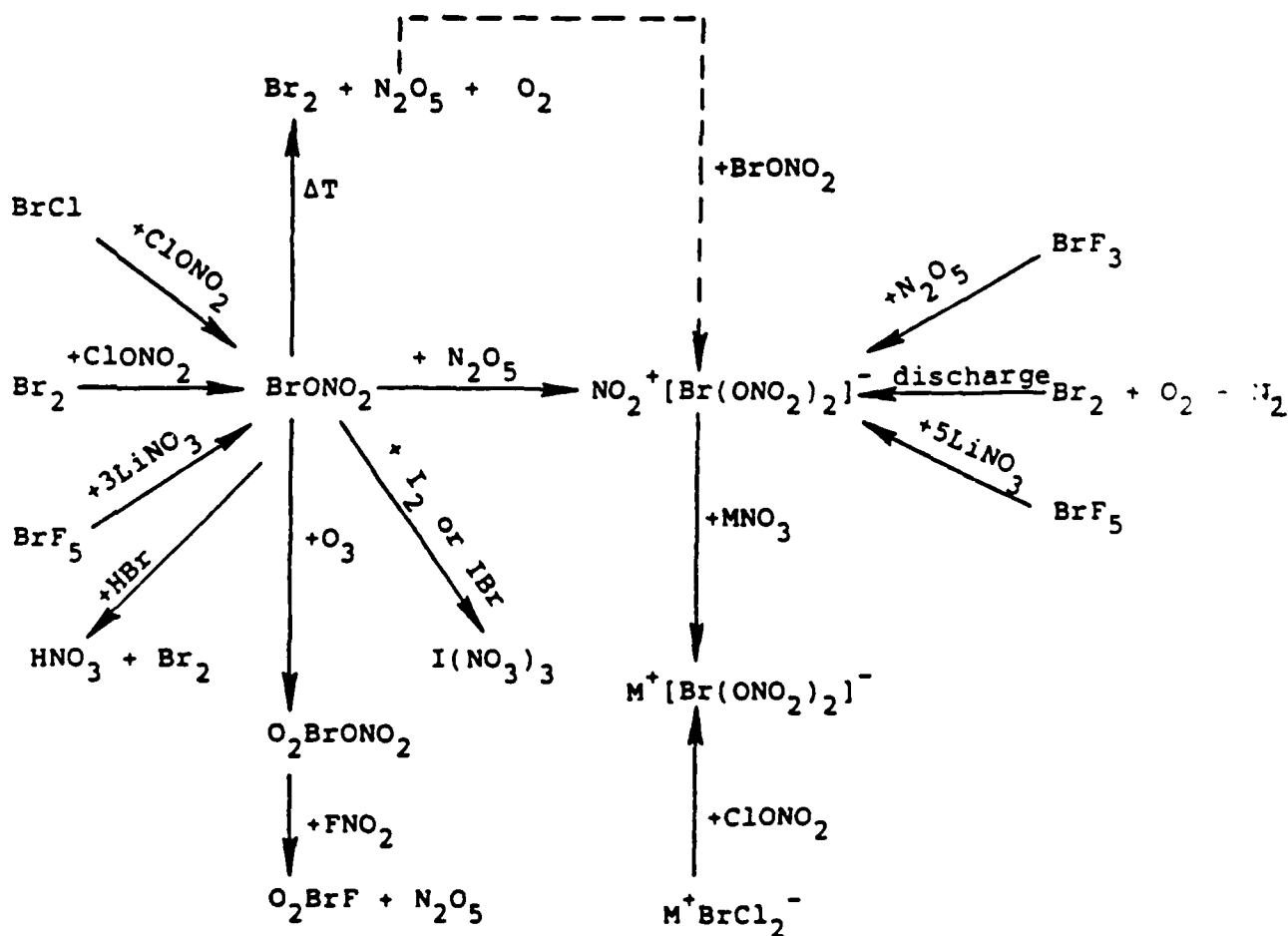
Scheme 1. Reaction Chemistry of Bromine Nitrates
