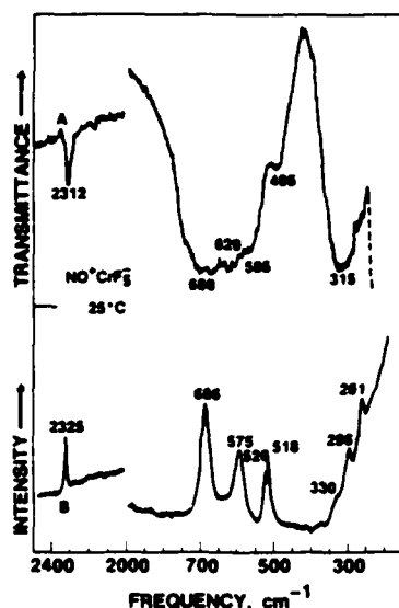
Figure 4. Vibrational spectra of solid \text{NOCrF}_5 : trace A, infrared spectrum; trace B, Raman spectrum.
