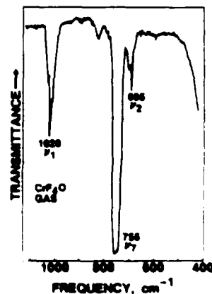
Figure 1. Infrared spectrum of gaseous CrF 5 O at 13 torr in a 5-cm Teflon cell with AgCl windows.
