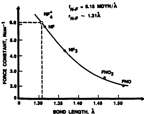
Fig. 1. Extrapolation of the N-F bond length of \text{NF}_4^+ from its stretching force constant.
