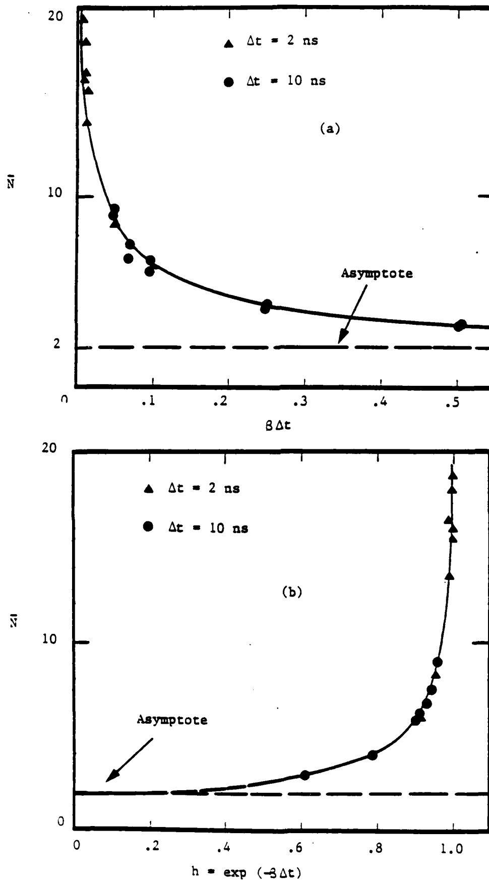
Figure 4.5. Monte Carlo Simulation Result of the Mean Time Step ( \bar{N} ) Between Zero-Crossings of the Velocity, (a) as a Function of \beta\Delta t ; (b) as a Function of h = \exp(-\beta\Delta t) .
