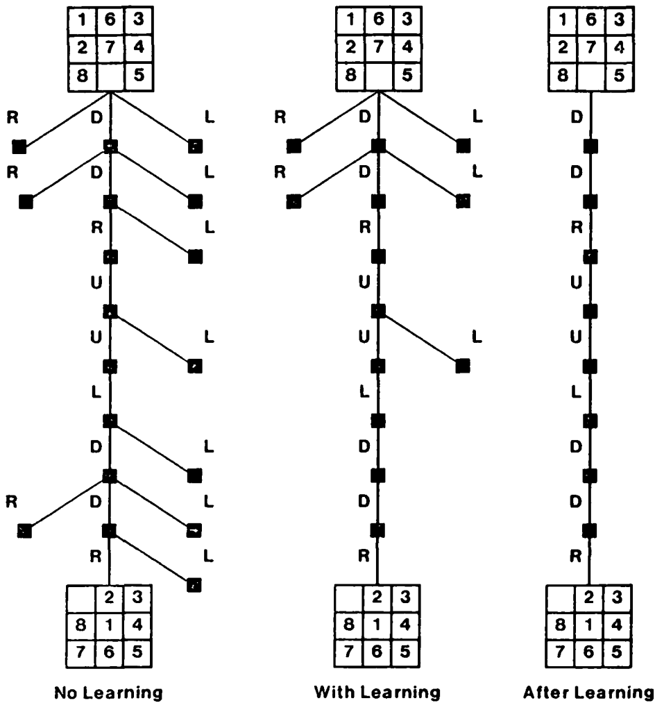
Figure 3-6: Learning in the eight puzzle [33].
