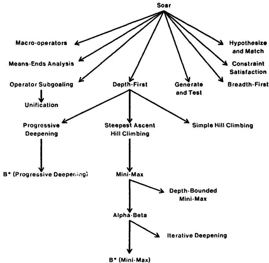
Figure 3-5: Structure of weak methods realized in Soar [29].
