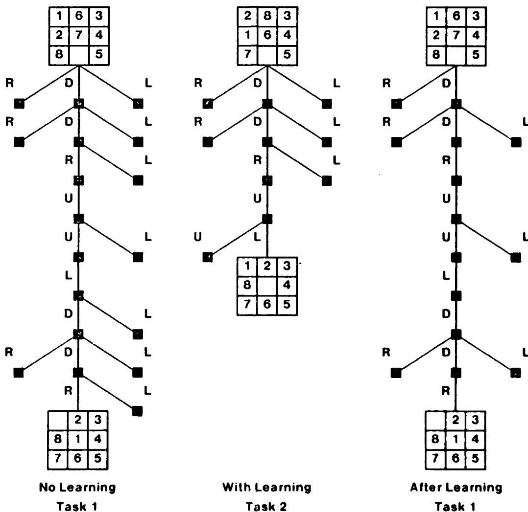
Figure 3-7: Across-task transfer in the eight puzzle [33].
