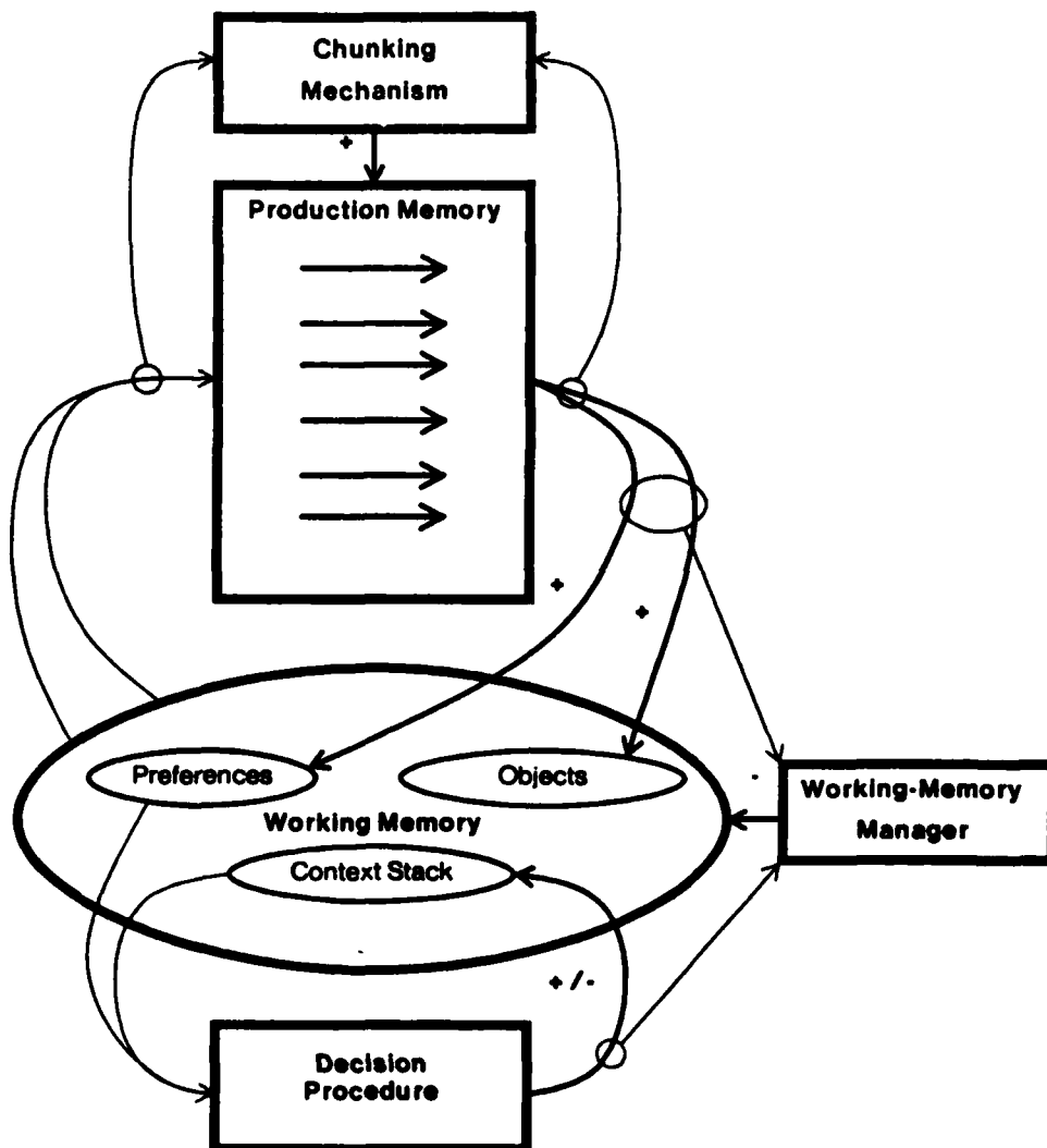
Figure 2-2: Architectural structure of Soar.
