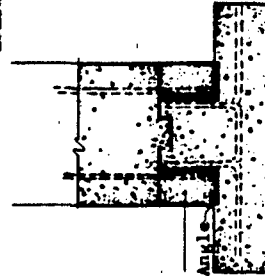
FIGURE D-16. WALL-TO-ROOF FOUNDATION JOINTS.
