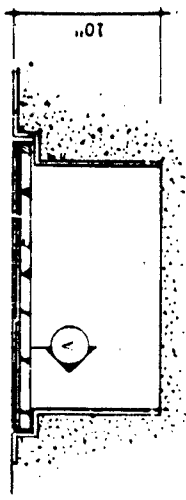
FIGURE B1-4. FLOOR TRACK DETAIL.
