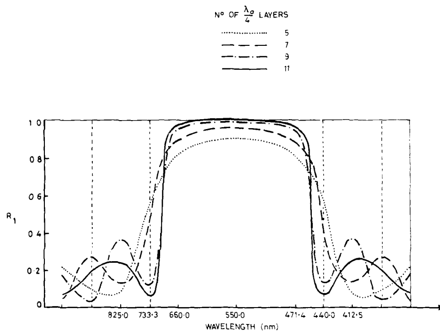
Figure 25. Reflectance versus wavelength for \frac{\lambda_0}{4} multilayers of zinc sulphide and cryolite ( \lambda_0 = 550 nm)
