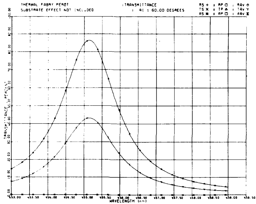
(h) Angle of incidence 60° (enlarged detail of figure 34(g))
