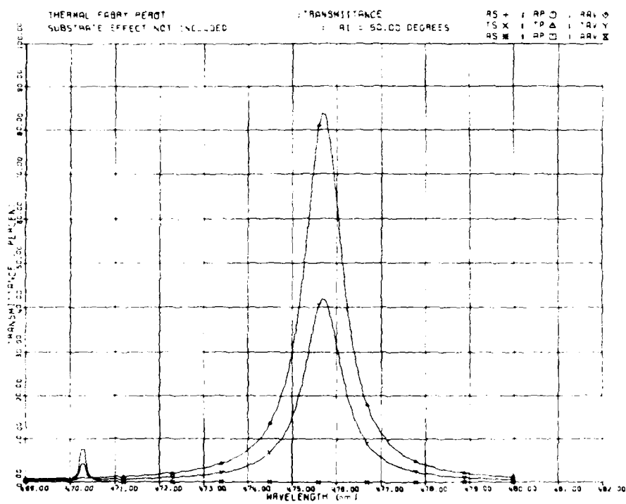
(e) Angle of incidence 50°
