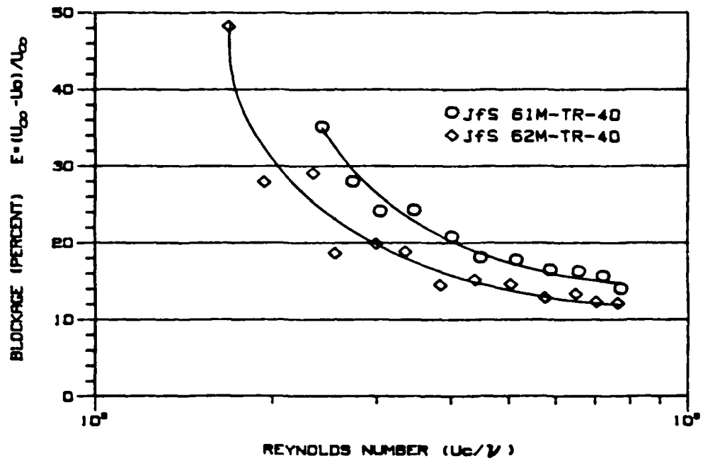
Fig. 7.13 Measured blockages of the Jfs 40 section
