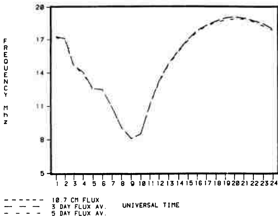
Figure 29. Effect of 10.7-cm solar flux index for Solid Shield, Hurlbert-Norfolk, 7 May 1981.
