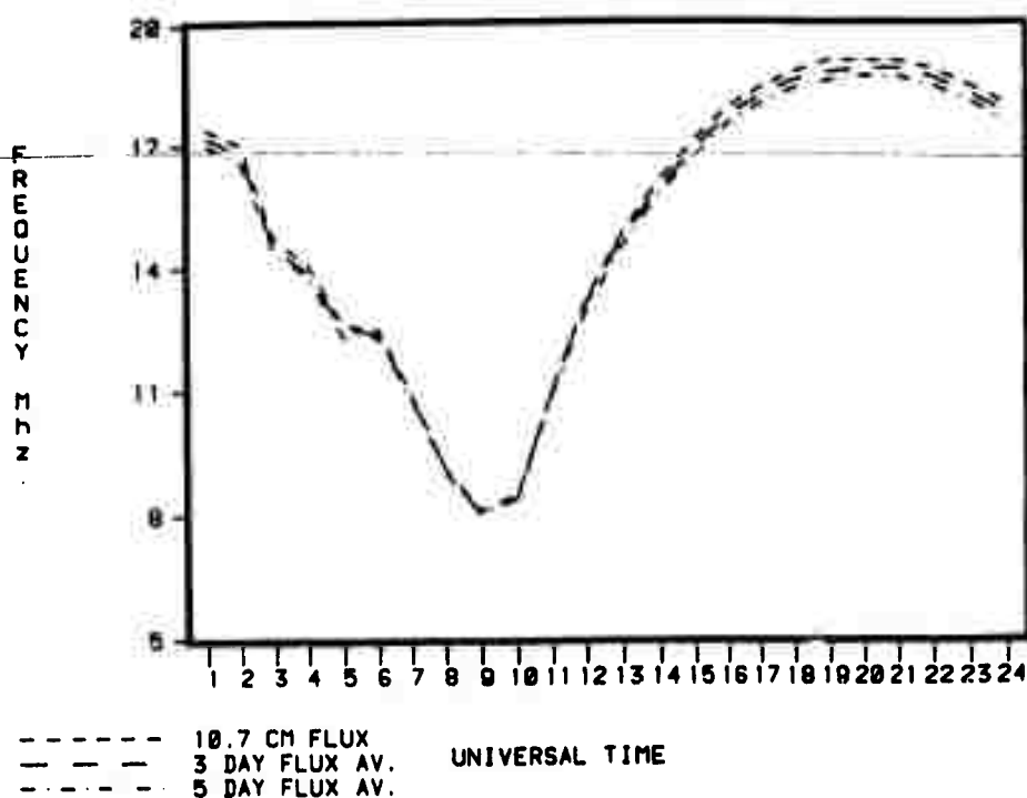
Figure 28. Effect of 10.7-cm solar flux index for Solid Shield, Hurlbert-Norfolk, 5 May 1978.
