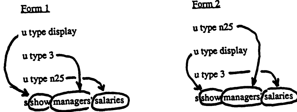
Figure 6e: Result of eliminating obligatory previous action heuristic.
