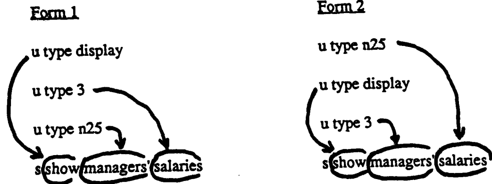
Figure 6d: After applying loose-ends heuristic.
