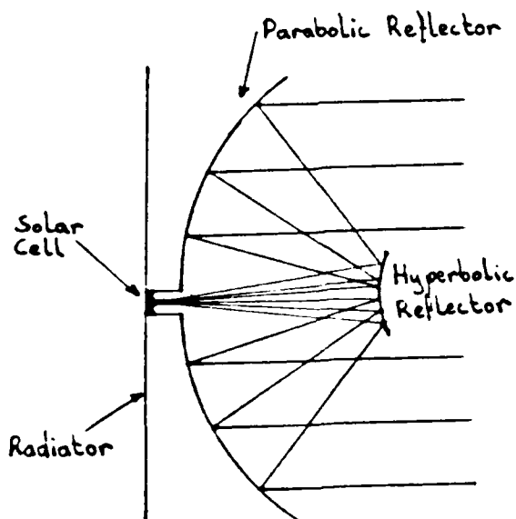
Figure 6. Cassegrain Type Modular Concentrator
