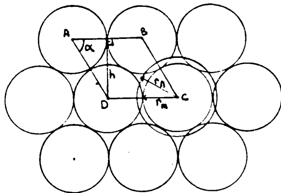
Figure 31. Orthogonal Packing of Mirrors
