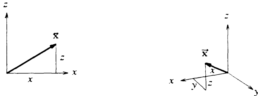
Fig.3.1. Cartesian Coordinates in 2-D and 3-D.
