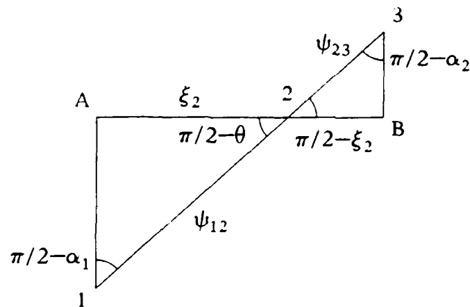
Fig.8.20. Two spherical triangles of interest for deriving the matching constraints.
