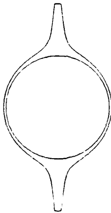
Profile of r_{11} -component of 3-D VST
