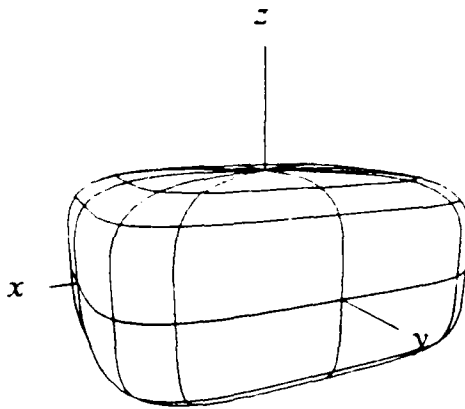
n=4.5
