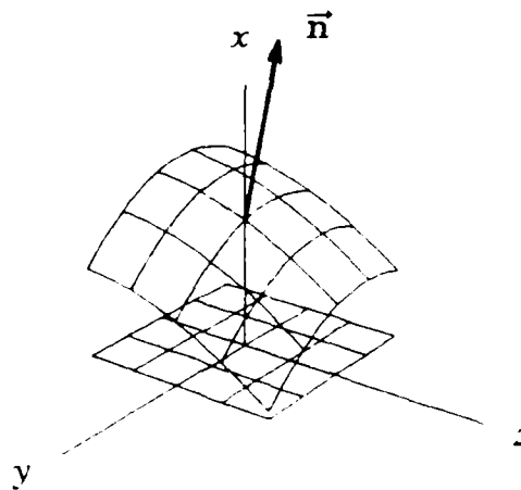
Fig.3.8. Monge parameterization for a Surface.
