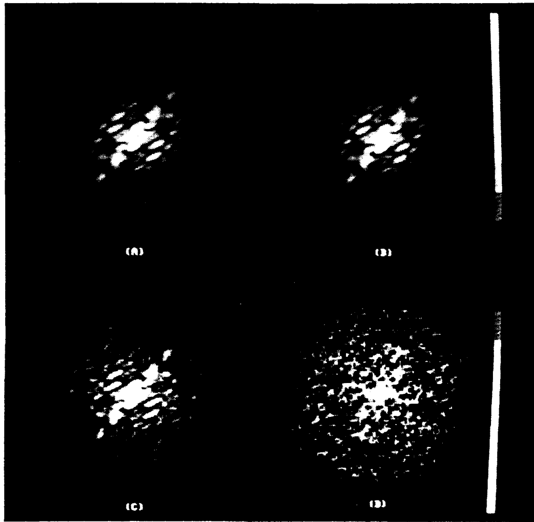
Figure 3. Fourier modulus estimates computed from 156 noisy, blurred images each. Number of photons per degraded image: (a) infinity (noise-free), (b) 305,000, (c) 6143, (d) 643.
