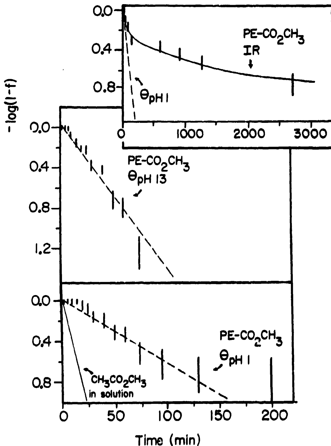
Figure 10. Kinetic plots for f_{\theta, pH 1} , f_{\theta, pH 13} and f_{IR} from the data on Figure 8. For comparison, the plot includes data for homogeneous hydrolysis of CH 3 CO 2 CH 3 under the same conditions. 26
