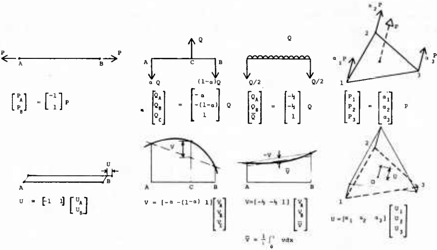
Fig. 3 Examples of Generalised Forces and Corresponding Displacements
