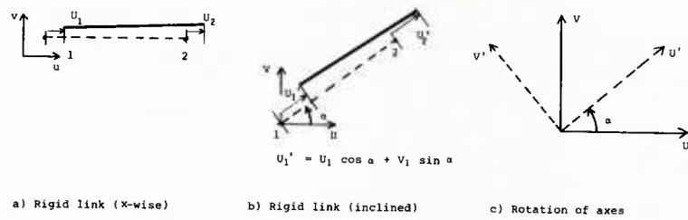
Fig. 4 Some Simple Displacement Transformations
