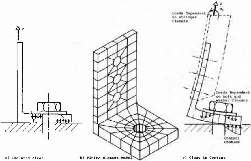
Fig 1 Analysis of a Tension Cleat
