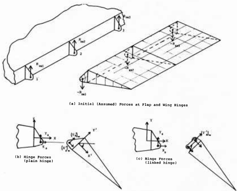
Fig. 6 Interaction Forces Between Wing and Flap
