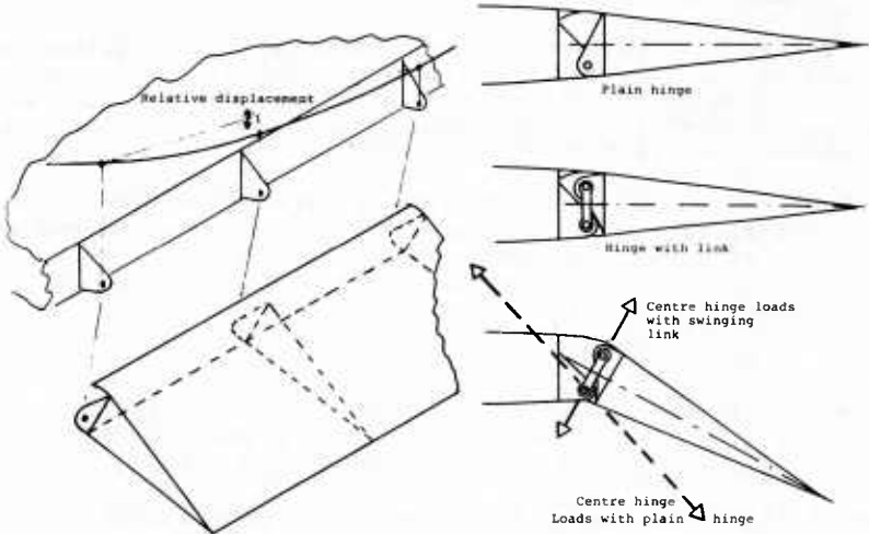
Fig. 2 Flap-Wing Interaction-Effect of Wing Displacements
