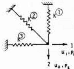
FIG. 7a. Two Degree of Freedom System
