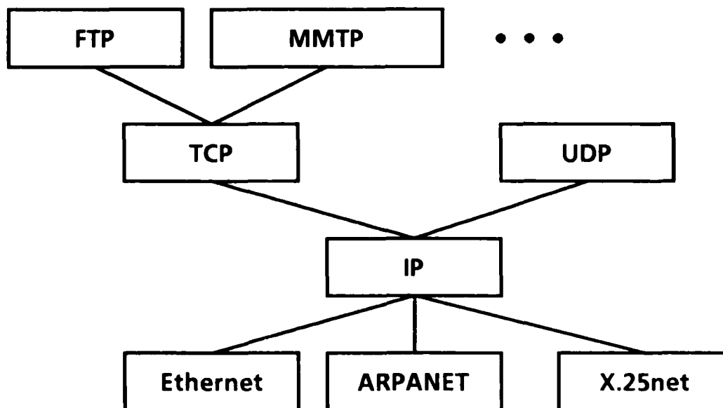
Figure 1: Protocol Architecture
