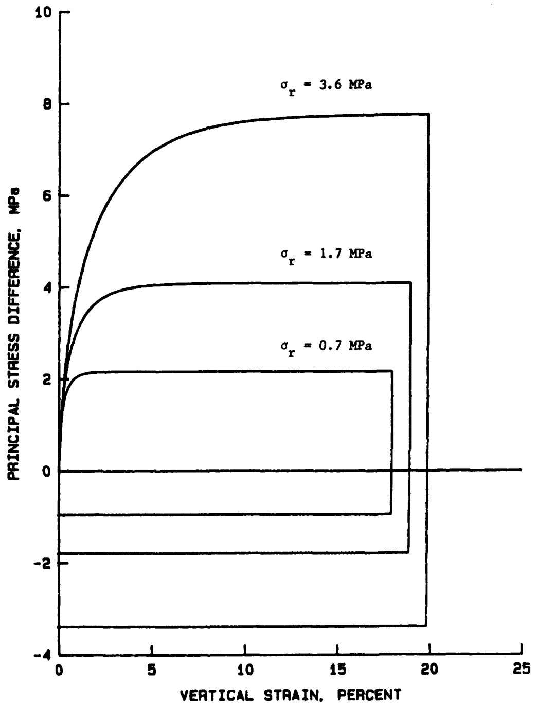
Figure 20. Strain-dependent cap model fit for ISST Layer 2: triaxial compression principal stress difference - vertical strain relations for low confining pressures.
