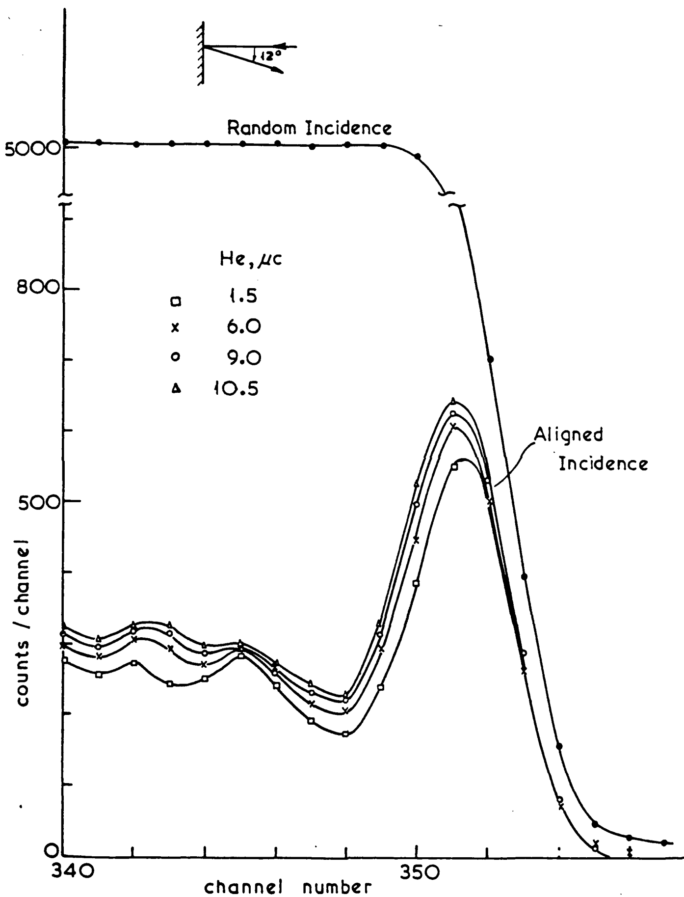
Fig 1 Rutherford backscattering/channelling spectra of random and \langle 100 \rangle aligned incidence 2 MeV \text{He}^+ ions from In atoms in an unimplanted InP substrate as a function of He ion fluence
