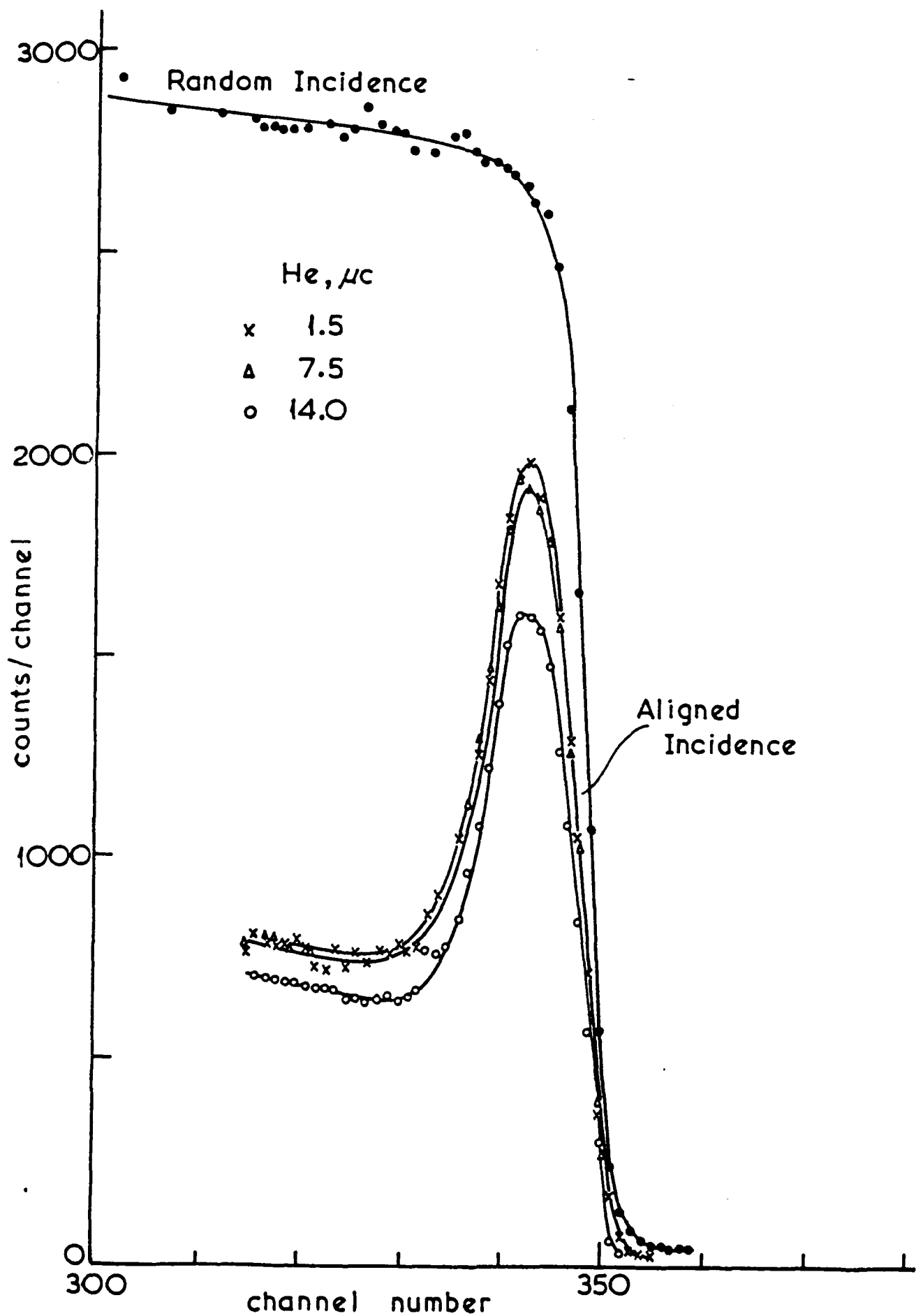
Fig. 2 Rutherford backscattering/channelling spectra of random and \langle 100 \rangle aligned incidence 2 MeV \text{He}^+ ions from In atoms in an InP substrate implanted with 40 keV 10^{14} \text{ N}^+ ions \text{cm}^{-2} as a function
