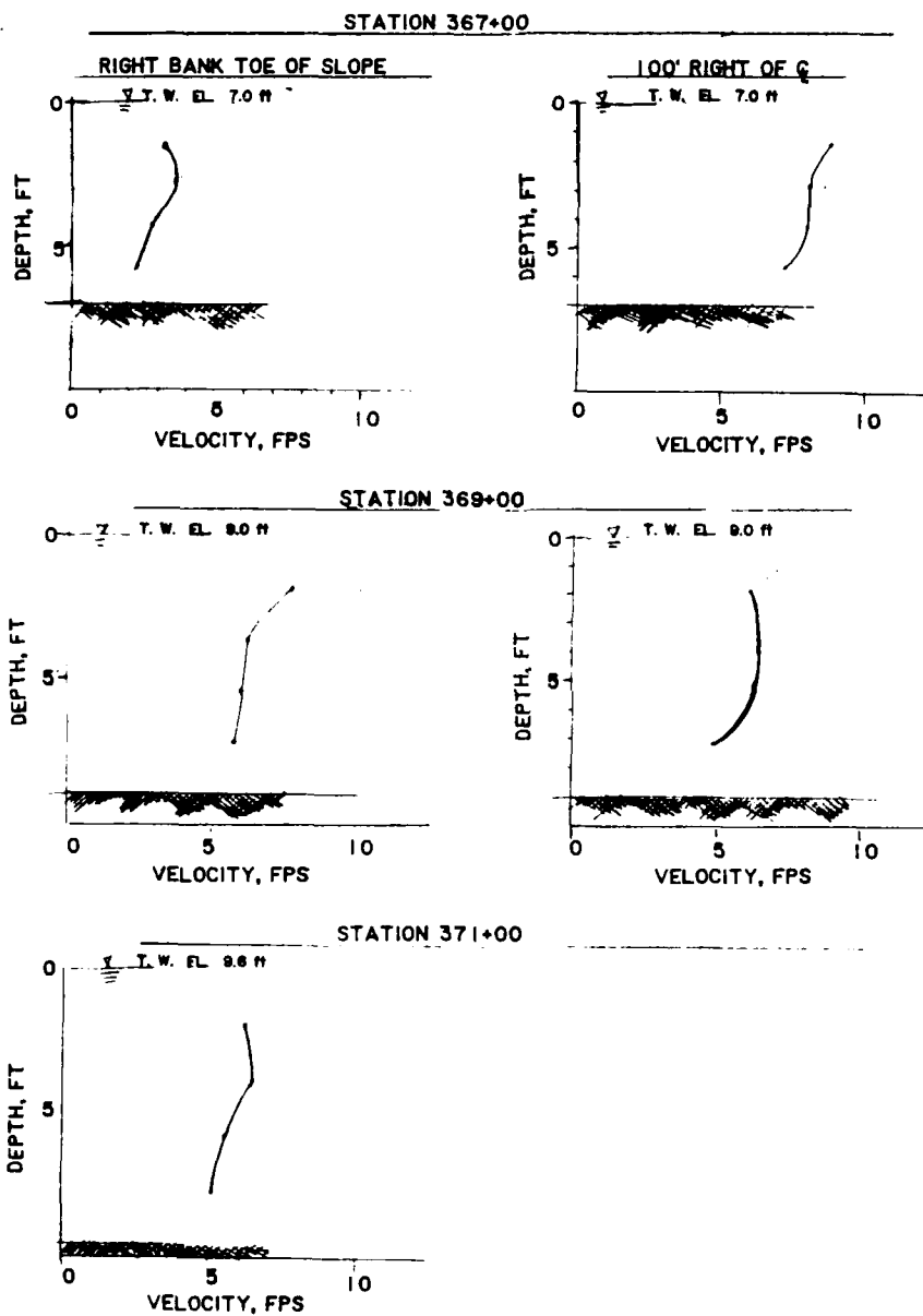
VELOCITY PROFILES TEST 7, UNIT 3 LOW TAILWATER
