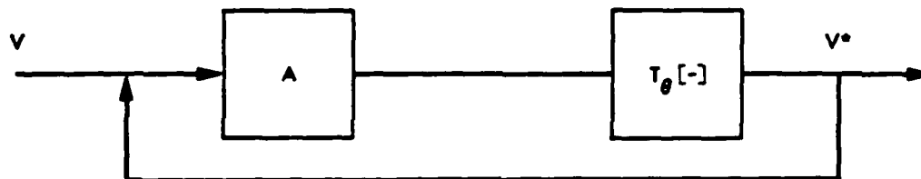
Figure 1. An iterative computing model for associative retrieval.
