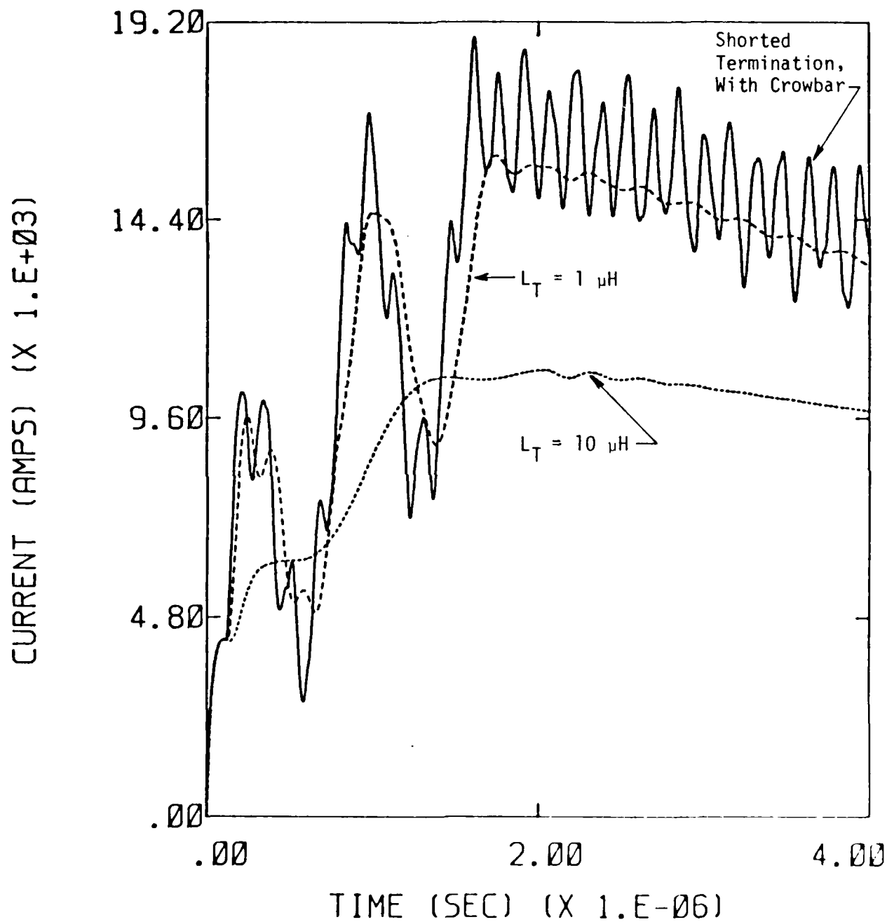
Figure 2.3 Current I with R_T = 71.4 and L_T = 1 \mu\text{H} and L_T = 10 \mu\text{H} , Both With a Crowbar. Results for Shorted Termination With Crowbar Also Shown for Comparison.
