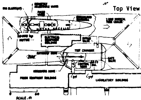
Fig. 1 Langley Transonic Dynamics Tunnel.
