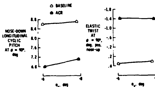
Fig. 10 Advancing side tip elastic twist and total pitch versus configuration performance ( r/R = .78 M_T = .65 ).
