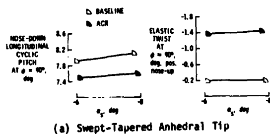
Fig. 10 Advancing side tip elastic twist and total pitch versus configuration performance ( r/R = .78 M_T = .65 ).
