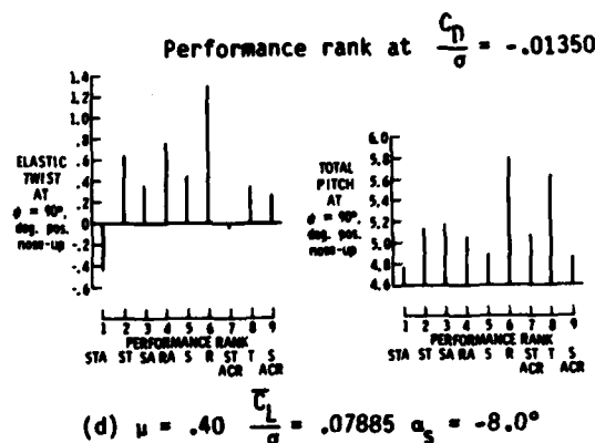
Fig. 10 Advancing side tip elastic twist and total pitch versus configuration performance ( r/R = .78 M_T = .65 ).
