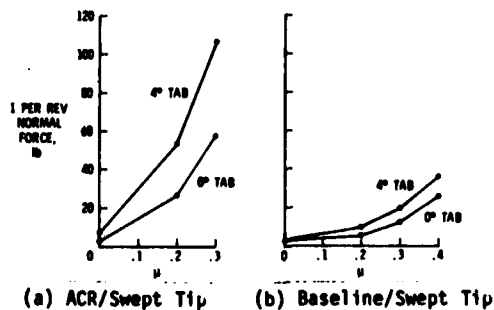
Fig. 15 Effect of Tab Deflection on Fixed System Normal Loads ( M_T = .65, \frac{\tau_L}{\sigma} = 0.075 ).
