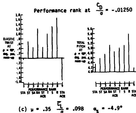
Fig. 10 Advancing side tip elastic twist and total pitch versus configuration performance ( r/R = .78 M_T = .65 ).
