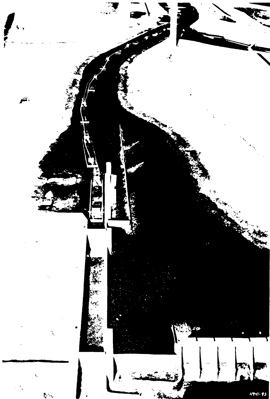
Photo 18. Plan B-35, upbound tow approaching the lock; discharge 31,000 cfs, tailwater el 21.0 (normal)
