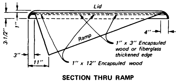
Figure 3. Construction details for commercially fabricated cistern lid and ramp for a gallinaceous guzzler (after USACE 1979)
