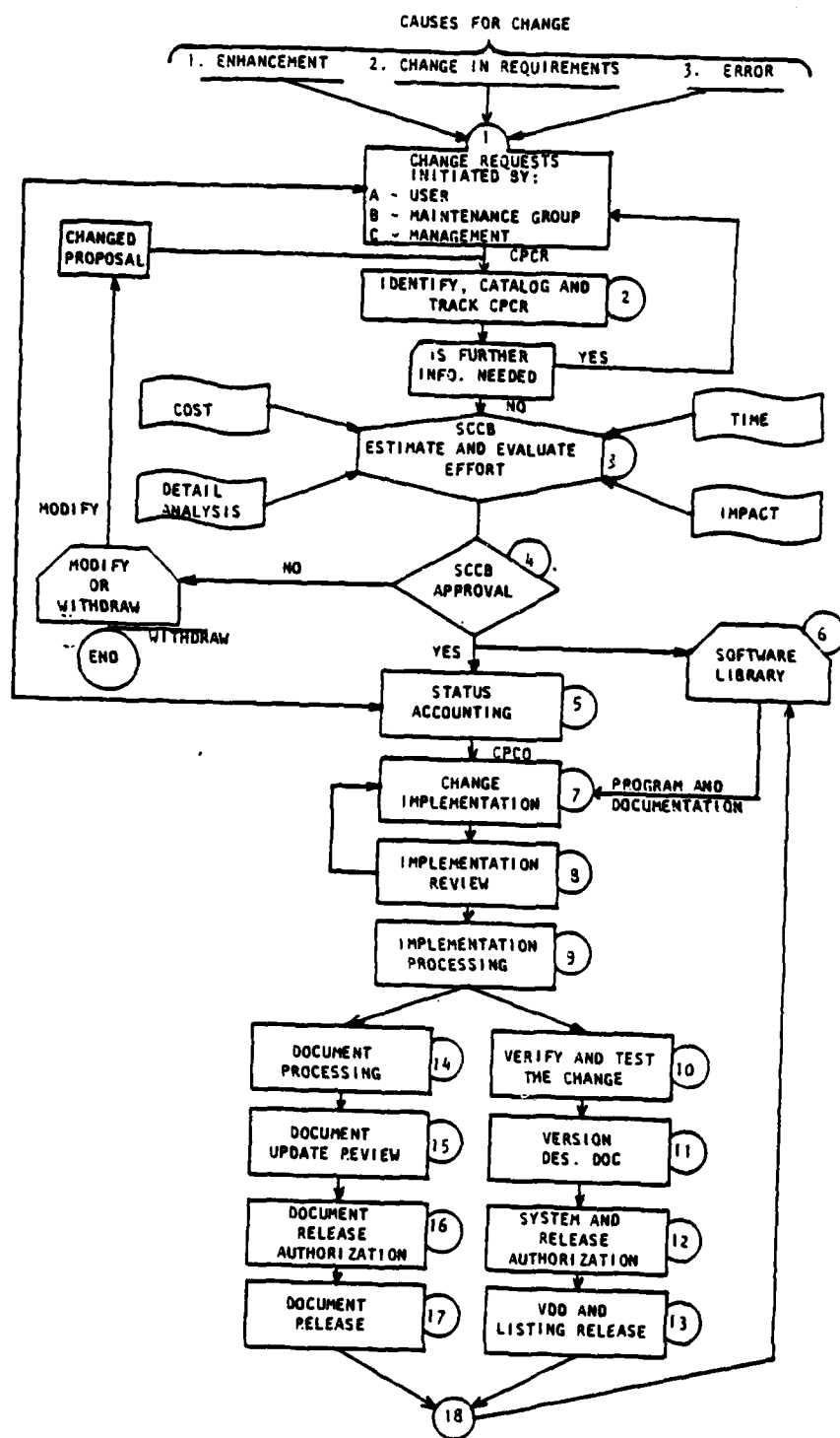
Figure 6.1 Improved Change Control Model
