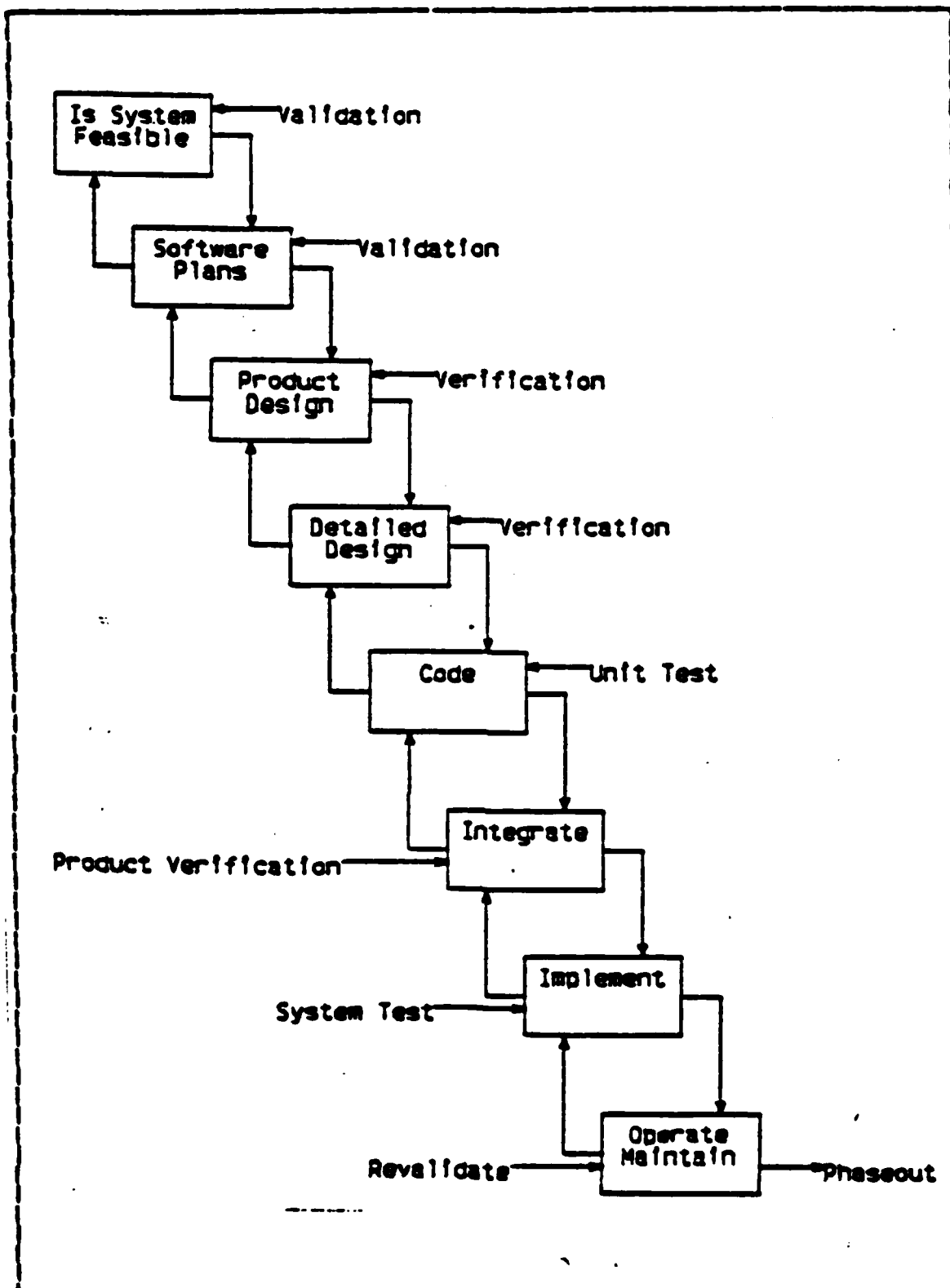
Figure 2.3 The Waterfall Model of the Software Life Cycle
