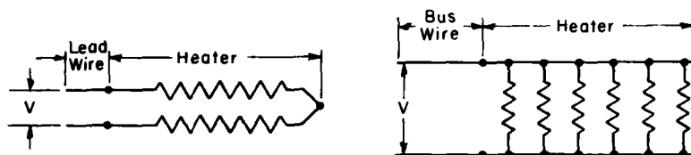
b. Parallel resistance, continuous type.
