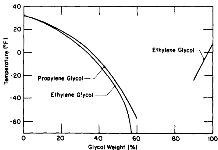
2. Freezing points of aqueous glycol solutions (redrawn from Dow Chemical Company literature).
