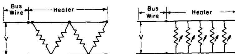
c. Parallel resistance, zonal type.
