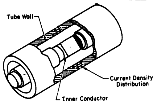
5. Current density distribution due to skin effect (after Burpee and Carson 1977).
