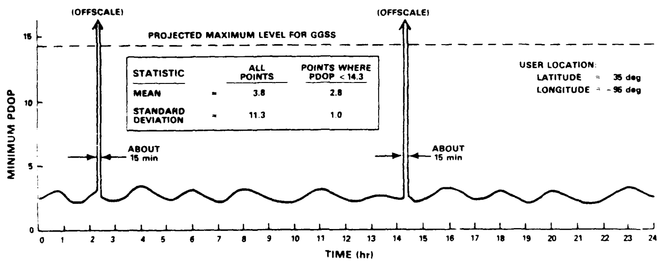
Figure A.3-5 Typical PDOP Characteristics at an Outage Location
