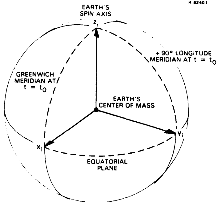
Figure A.2-3 Inertial Coordinates
