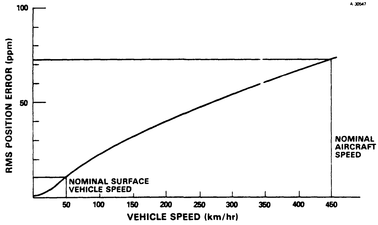
Figure 3.4-1 Sensitivity of Position Measurement Accuracy to Vehicle Speed
