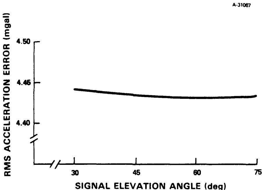
Figure 3.4-6 Sensitivity of Acceleration Measurement Accuracy to Signal Elevation Angle
