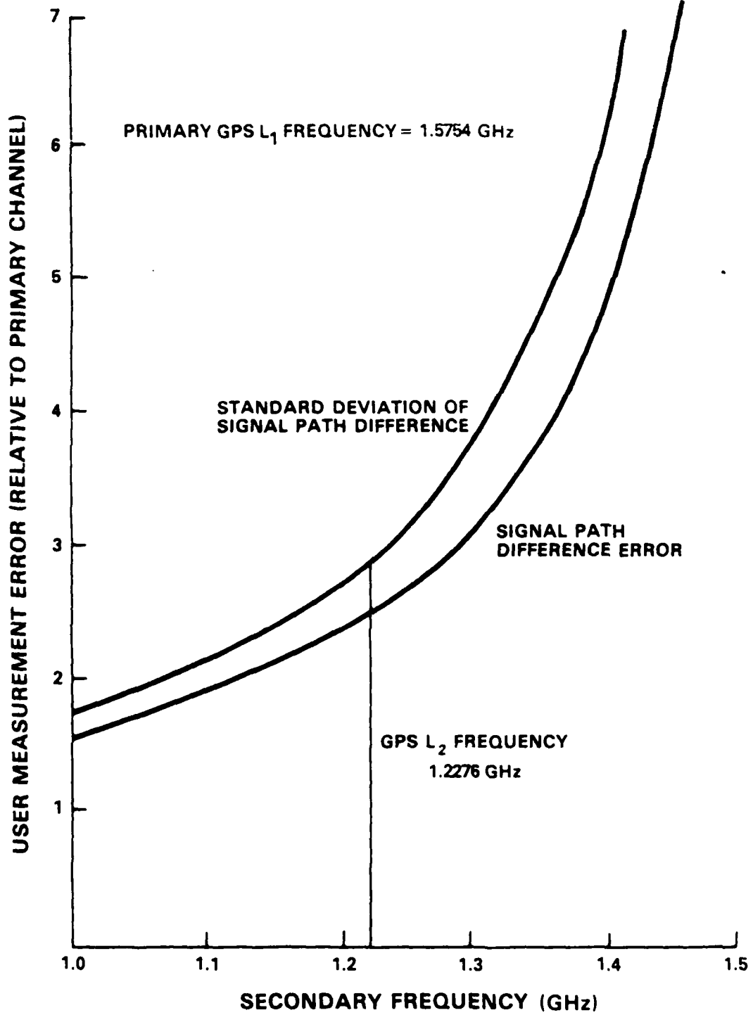
Figure C.4-2 Frequency Dependence of Receiver Measurement Error
