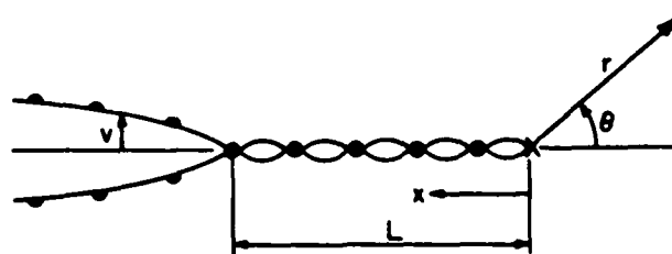
Fig. 1 Partially bridged crack
