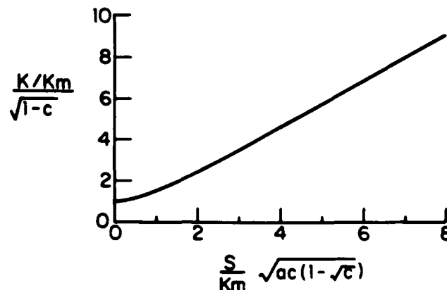
Fig. 3 Particulate toughening
