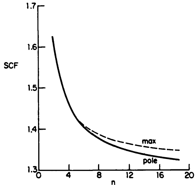
Fig. 8 Asymptotic stress concentration factors, S/\sigma_1 \rightarrow \infty
