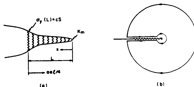
Fig. 2 (a) Spring model, (b) J-integral path
