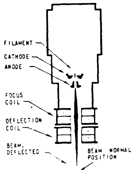
Fig. 2.3, Illustration, Beam Deflection
