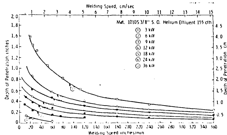
FIGURE 30 NVEB DEPTH OF PENETRATION VS. WELDING SPEED AT SELECTED POWER LEVELS. MATERIAL 1010 CARBON STEEL, 3/8" STANDOFF, HELIUM GAS EFFLUENT. (WESTINGHOUSE DATA)
