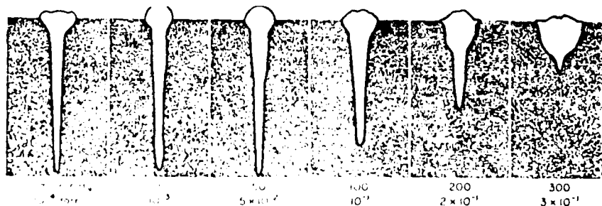
FIGURE 3 EFFECT OF WELDING CHAMBER PRESSURE ON PENETRATION AND WELD SHAPE
