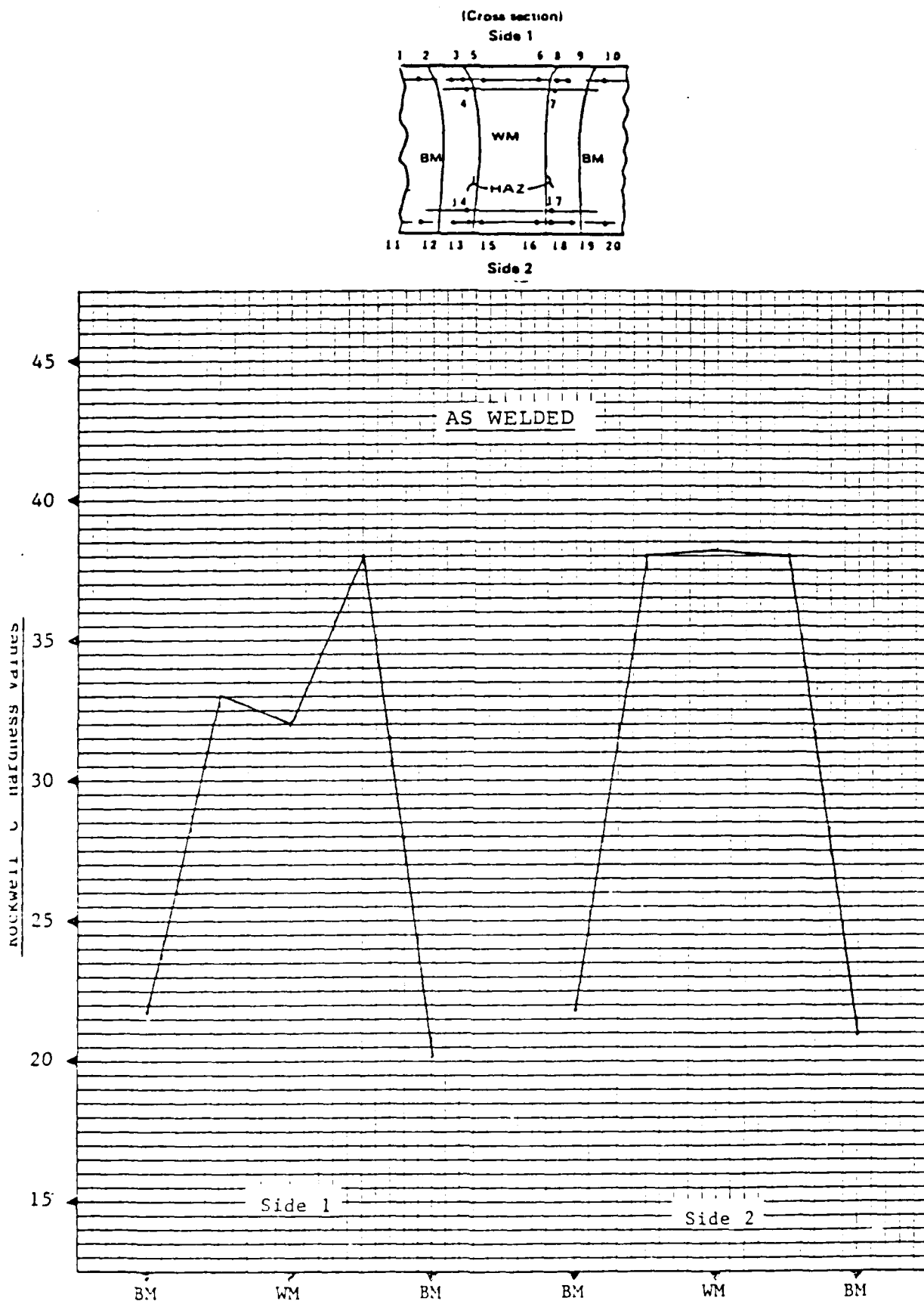
FIGURE 67 ROCKWELL "C" TRAVERSE HARDNESS VALUES FOR ELECTRON BEAM WELDED HY-100 MATERIAL - AS-WELDED
