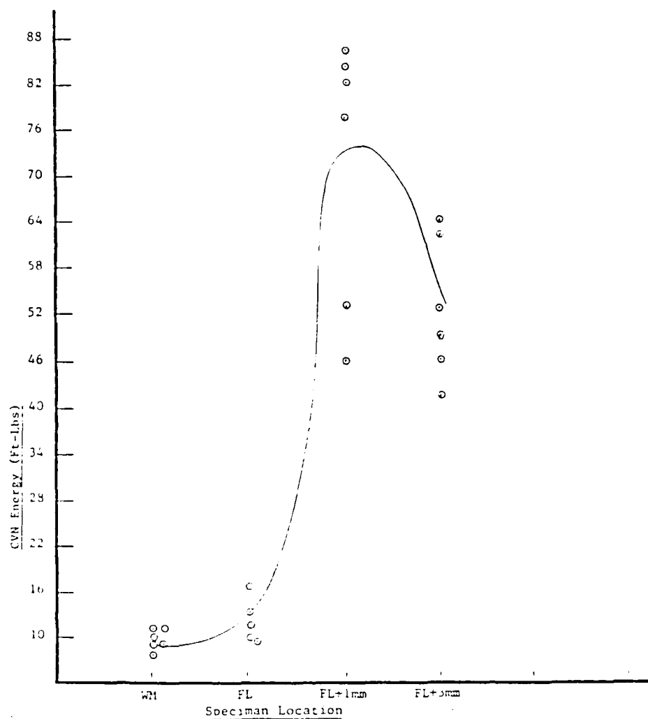
FIGURE 66 CHARPY V-NOTCH IMPACT RESULTS FOR ELECTRON BEAM WELDED HY-100 MATERIAL - AS-WELDED (TEST TEMP. -120^{\circ}\text{F} )
