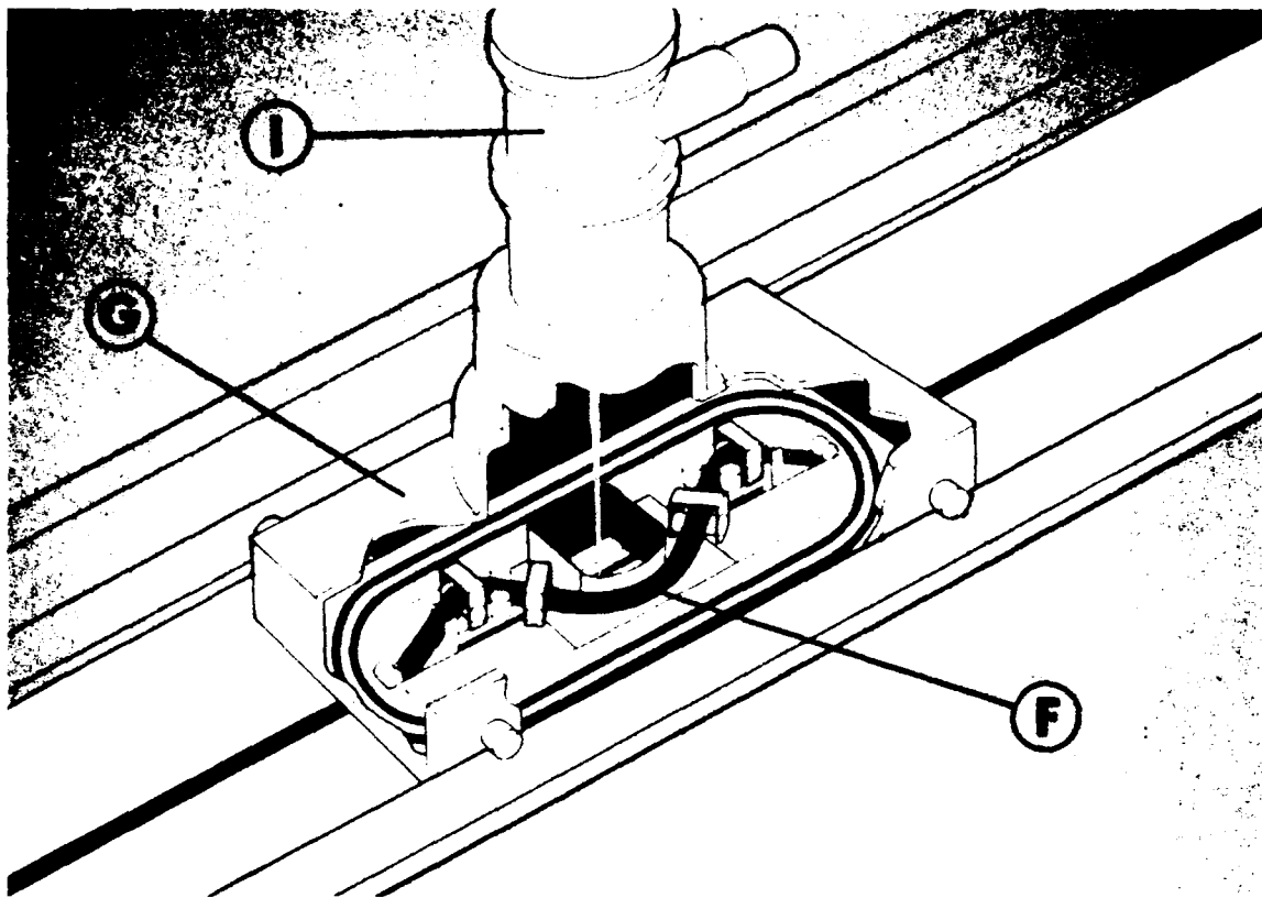
FIGURE 21 SKETCH OF SCI AKY CARRIAGE AND ELECTRON GUN
