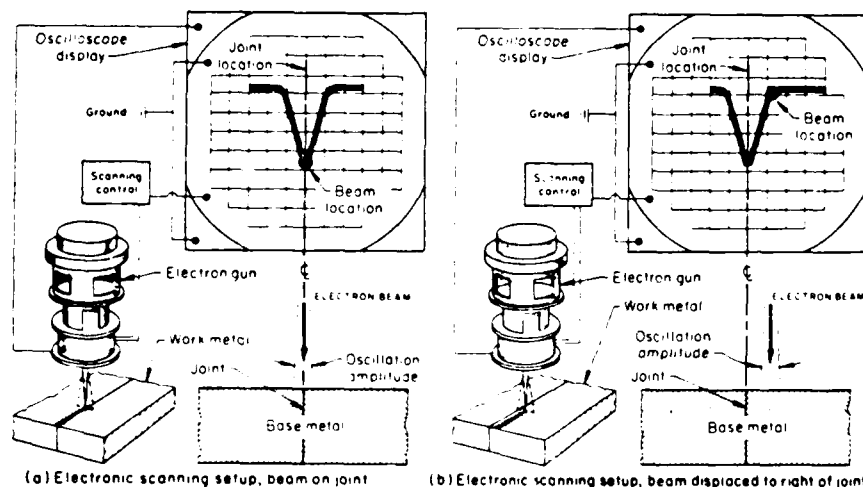
FIGURE 8 ILLUSTRATION OF RECORD AND PLAYBACK ELECTRONIC SCANNING
