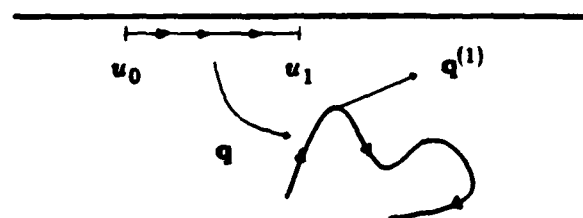
Figure 1. The univariate parametrization q generates an oriented curve by deformation of the oriented line segment [u_0, u_1] .
