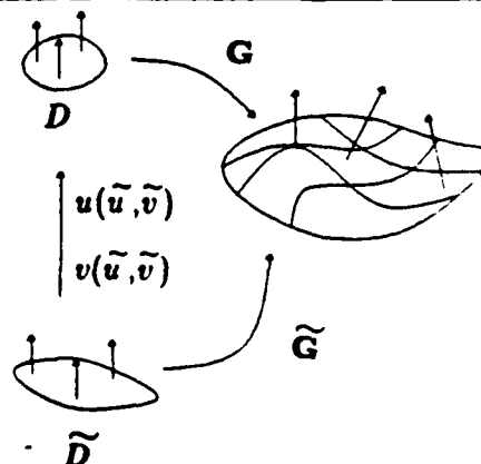
Figure 8. G and \tilde{G} are GO-equivalent parametrisations related by the change of parametrisation determined by u(\tilde{u}, \tilde{v}) and v(\tilde{u}, \tilde{v}) .
