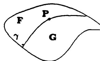
Figure 7. The surface patches generated by the parametrisations F and G meet at the boundary curve \gamma .
