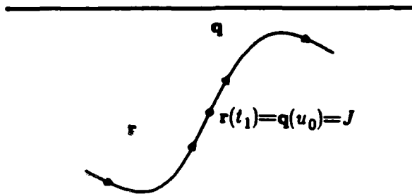
Figure 4. The parametrisations r(t) and q(u) meet at the common point J .
