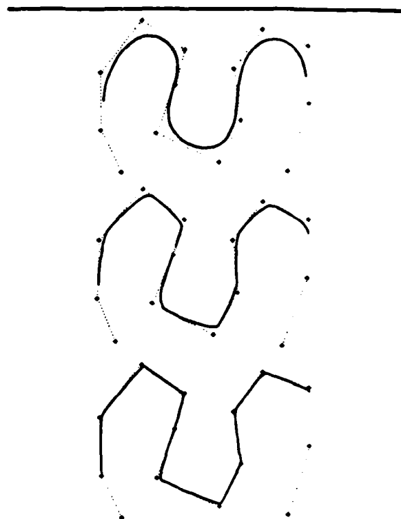
Figure 5. The curves above share the same control polygon, and all have \beta_1 = 1 and \beta_3 = 0 ; they differ only in the value of \beta_2 . The top curve has \beta_2 = 0 , the middle curve has \beta_2 = 20 , and the bottom curve has \beta_2 = 100 .
