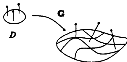
Figure 6. The bivariate parametrisation G deforms the oriented domain D to generate an oriented surface patch.
