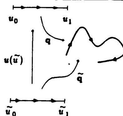
Figure 3. The equivalent parametrisations q and \tilde{q} are related by the change of parameter u(\tilde{u}) .
