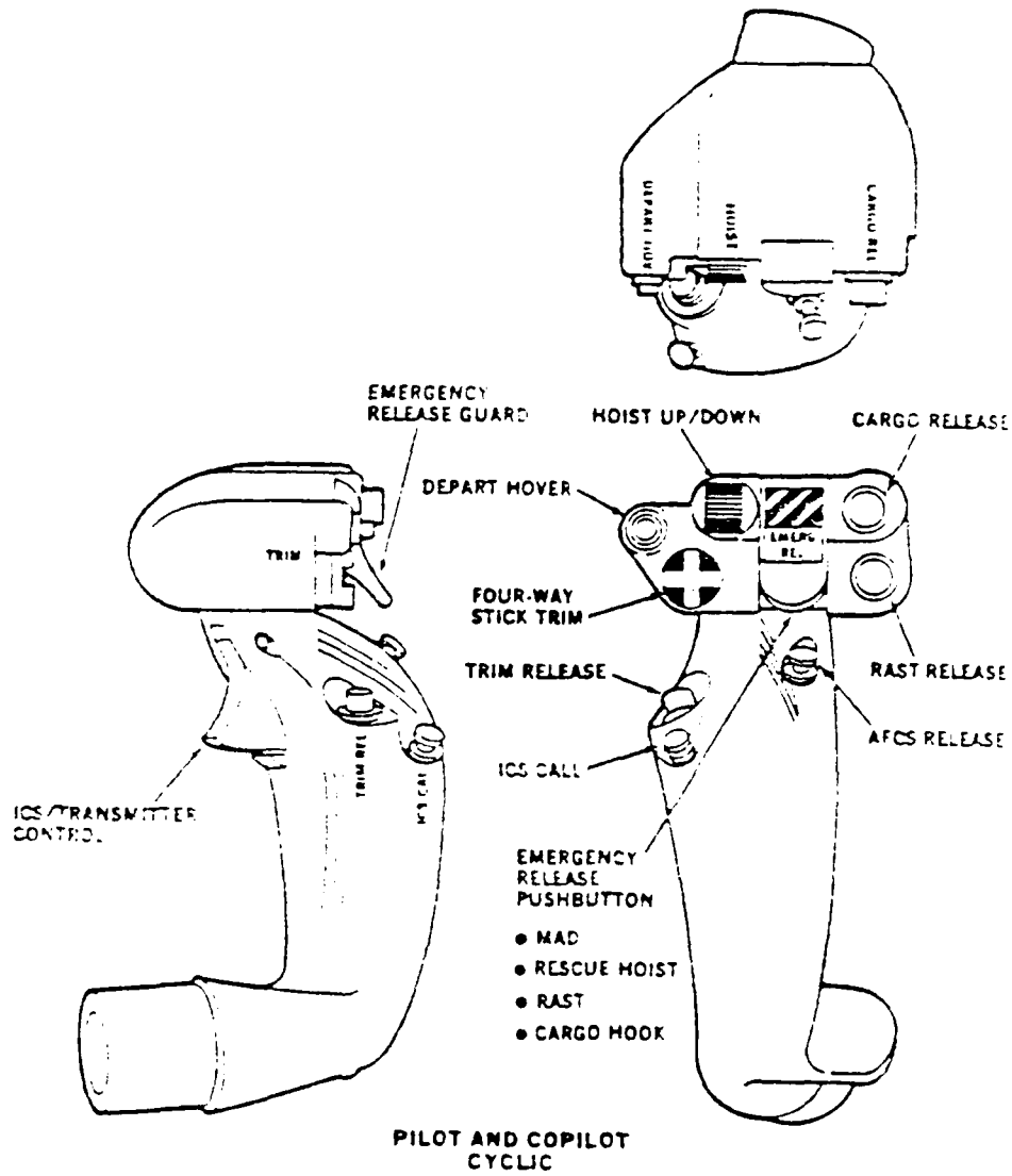
PILOT AND COPILOT CYCLIC Figure A-2. Cyclic
