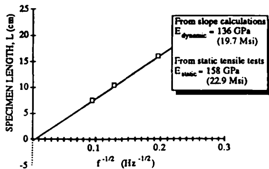
Figure 1 An Indication of Parametric Losses at the Grips in a Clamped-Free Flexure Apparatus.
