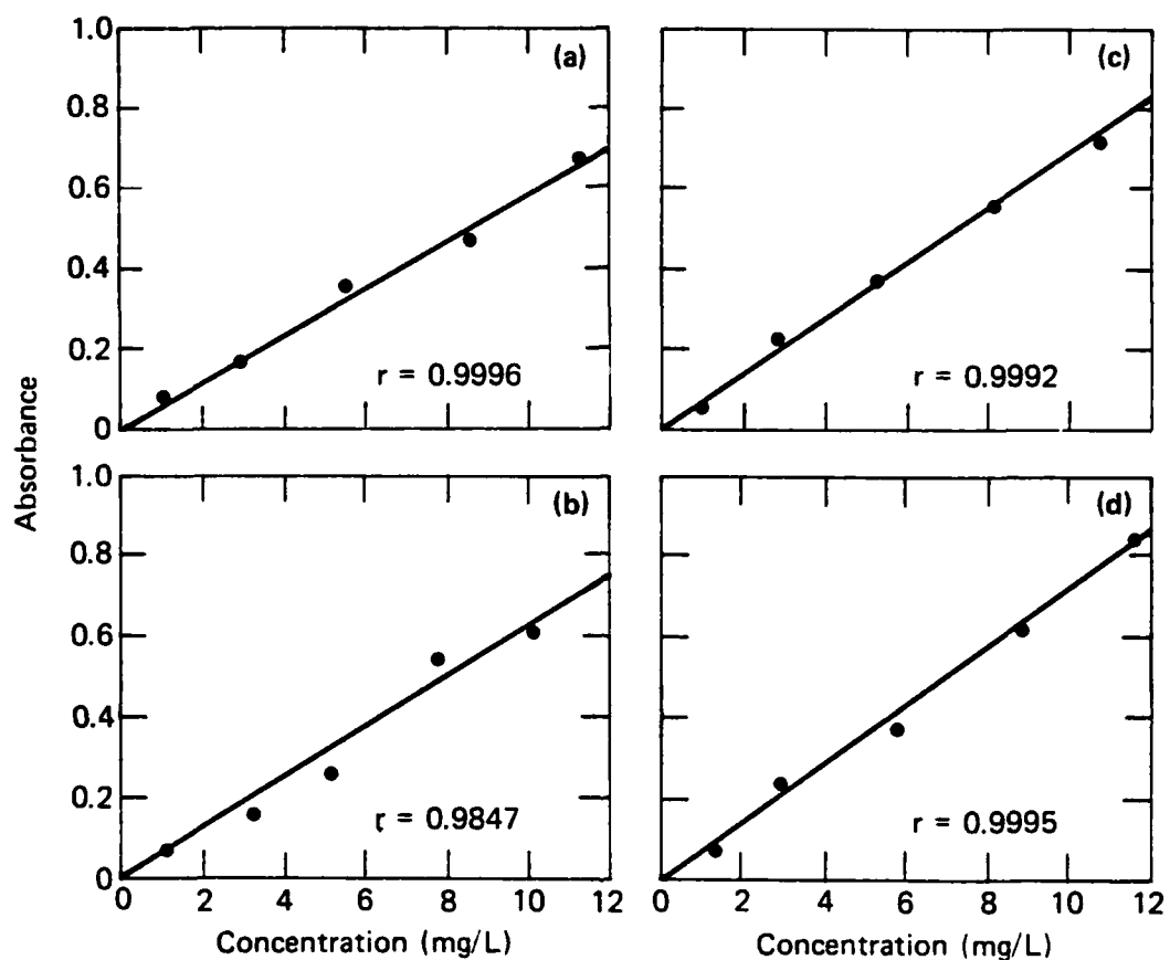
Fig. 1 The linear correlation between absorbance (254 nm) and concentration of the solvent yellow 33 and solvent green 3 using the Varion spectrophotometer; (a) Lovelace purified solvent yellow 33, (b) Technical solvent yellow 33, (c) Lovelace purified solvent green 3, (d) Technical solvent green 3.
