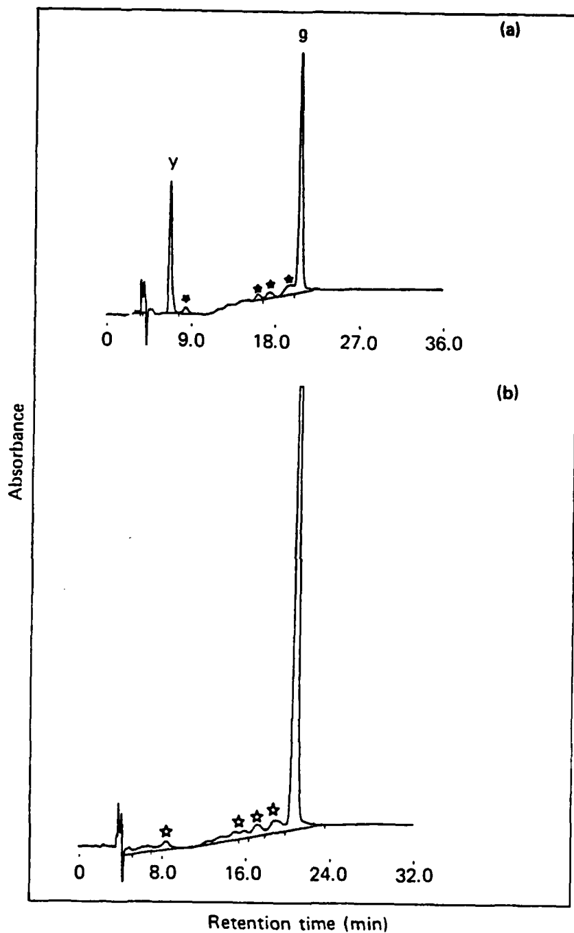
Fig. 6 Comparison of HPLC chromatograms of Technical solvent green 3 with the Lovelace purified solvent green 3; (a) 5.0 mg/L Technical solvent green 3 with yellow 33 component (y) and green 3 component (g) indicated, (b) 5.7 mg/L Lovelace purified solvent green 3. Note the absence of the yellow component in the purified dye. The stars indicate minor contaminants shared by the two formulations.
