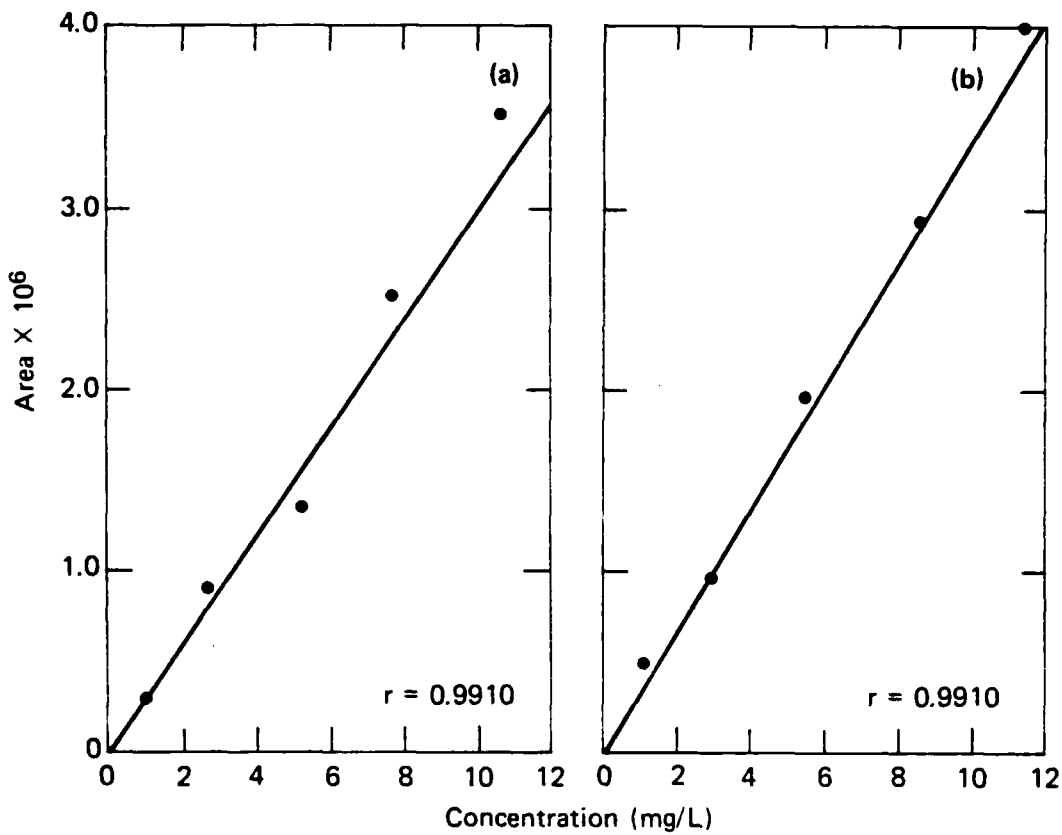
Fig. 4 The linear correlation between area of absorbance (254 nm) and concentration using the Waters HPLC; (a) Technical solvent yellow 33, (b) Lovelace purified solvent yellow 33.
