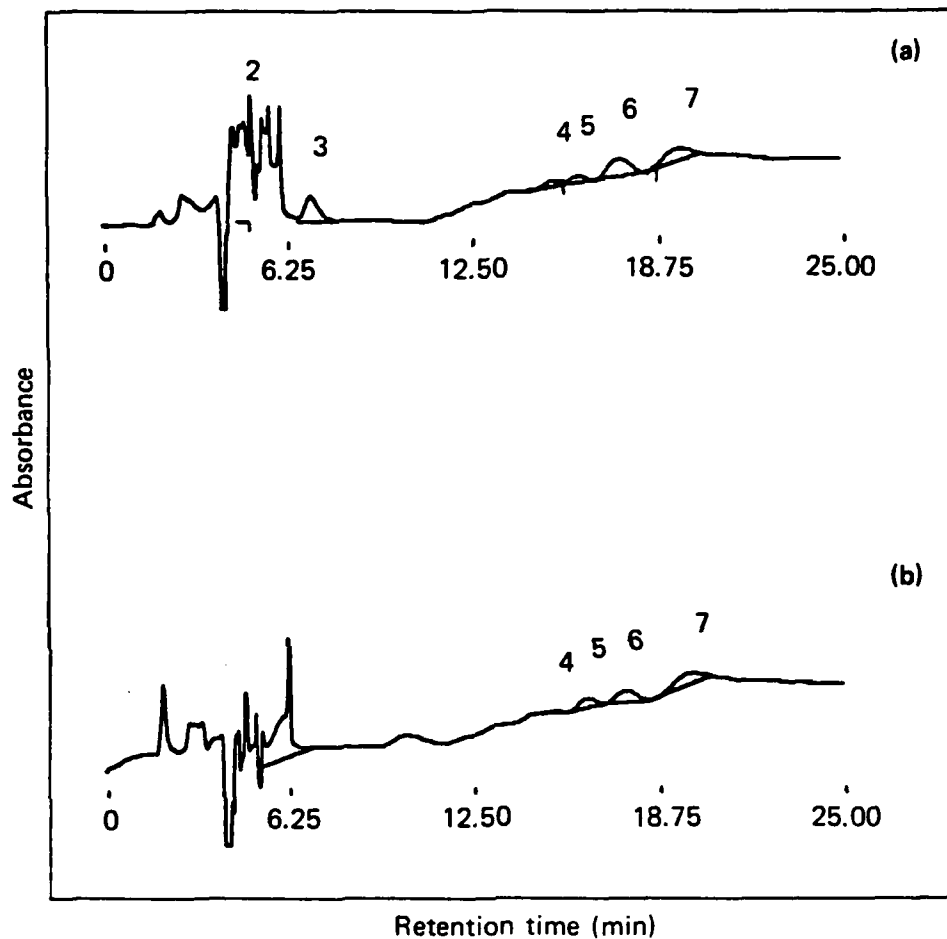
Fig. 8 Comparison of HPLC chromatograms of dissolved Technical solvent green 3 and control diluent water: (a) Technical solvent green 3 (solvent yellow 33 component present at a concentration of approximately 0.15 mg/L- peak 3; solvent green 3 component not detected at a retention time of 21 min), (b) diluent water only. Note the absence of the solvent yellow 33 component.
