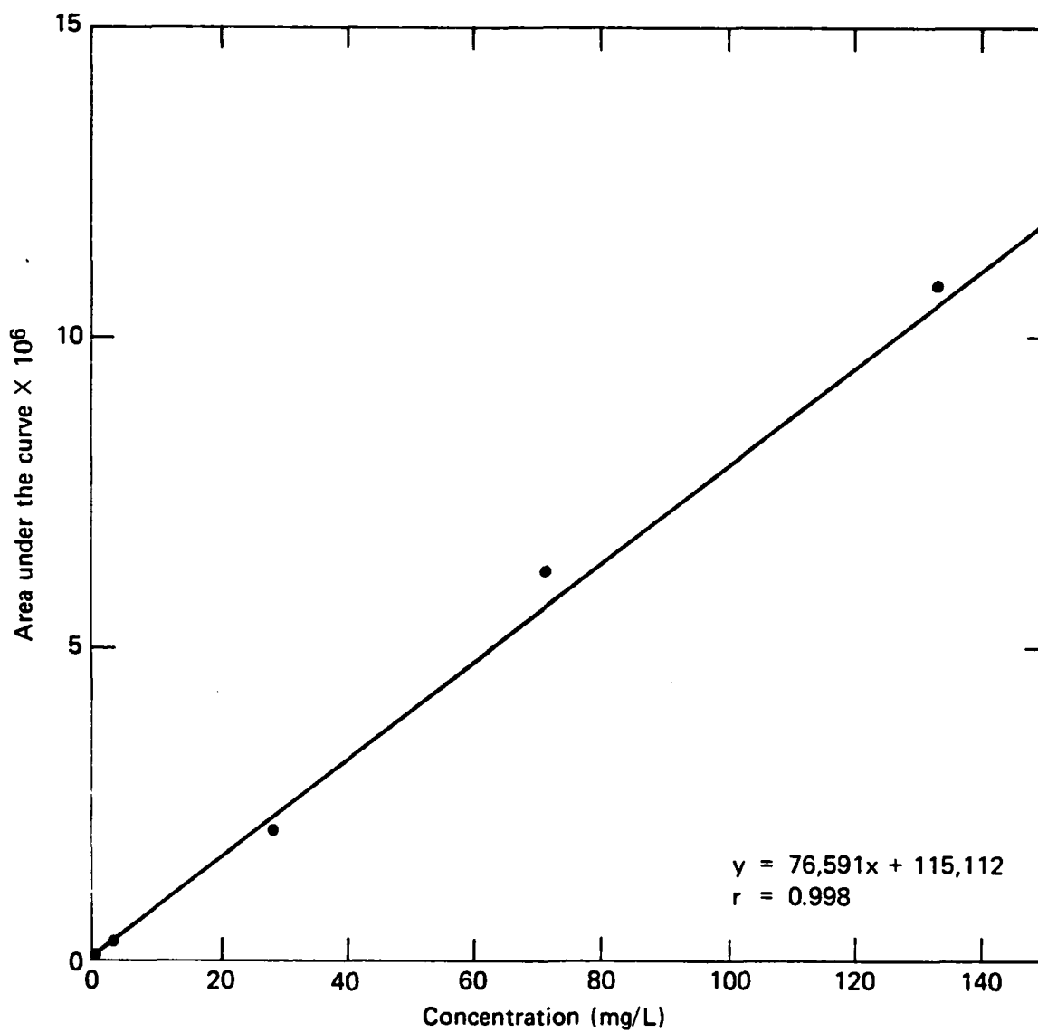
Fig. 16 The linear correlation between absorbance (215 nm) and concentration of DEGDN dissolved in diluent water using the HPLC. Injection volume was 100 \mu L.
