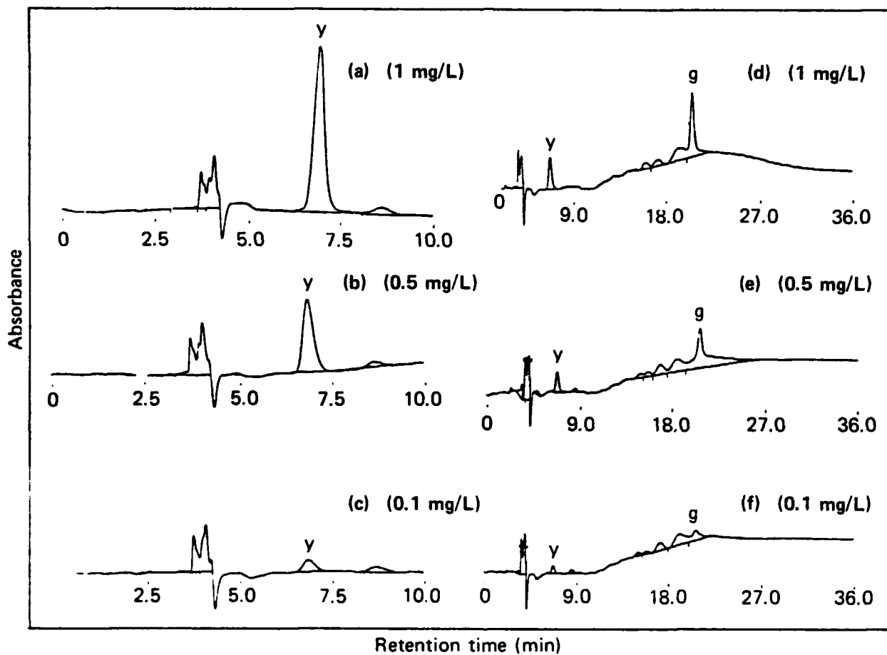
Fig. 2 HPLC chromatograms of technical grade solvent yellow 33 (a,b,c) and solvent green 3 (d,e,f). Note: The lower case (y) stands for solvent yellow 33 and the lower case (g) stands for solvent green 3.
