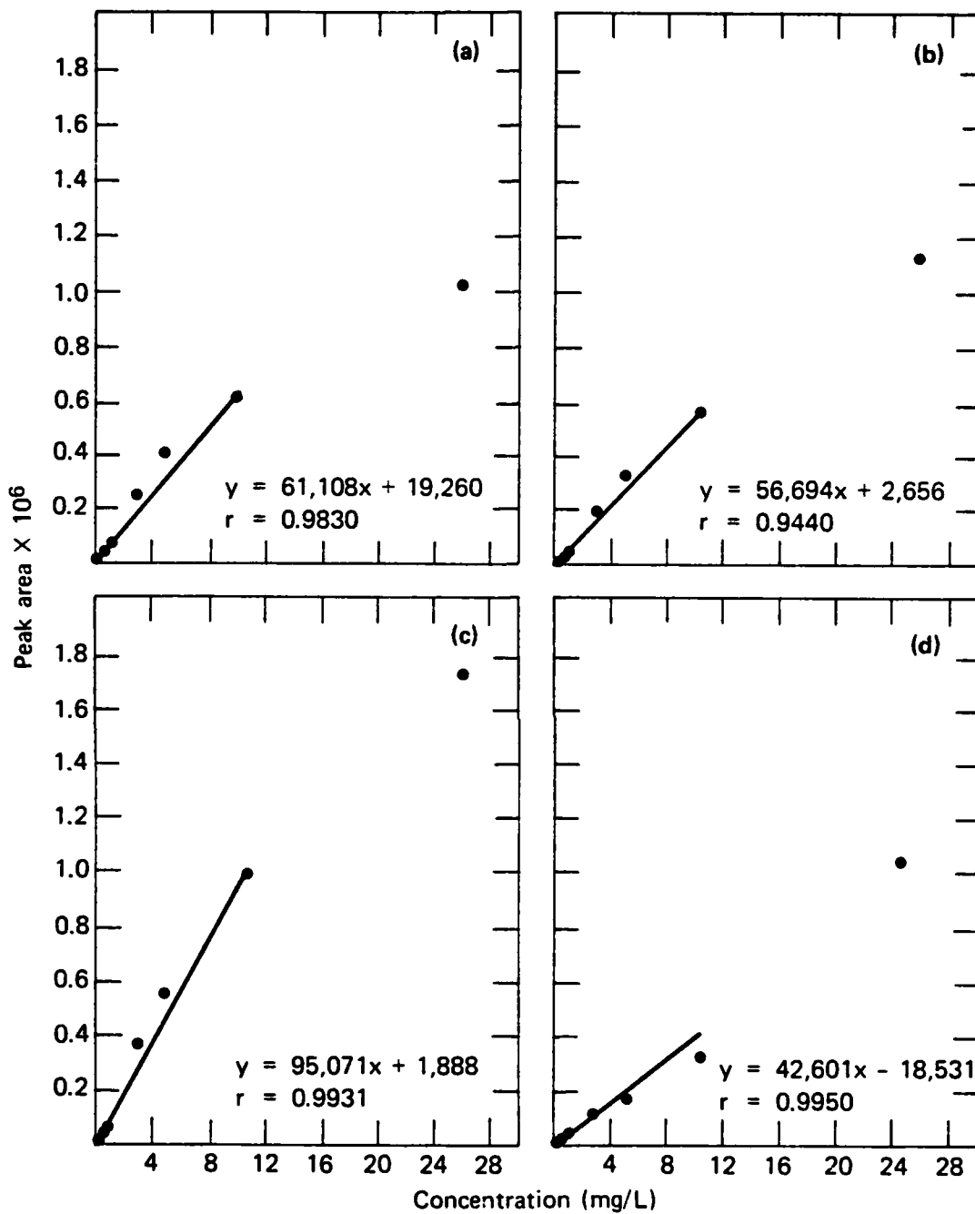
Fig. 9 The linear correlation between peak area and concentration for the chlorinated organics in the synthetic-HC smoke combustion products mixture using gas chromatography methods: (a) CCl 4 , (b) C 2 Cl 4 , (c) C 2 Cl 6 , (d) C 6 Cl 6 . (Regressions based on concentrations from 0.1 to 10.0 mg/L.)
