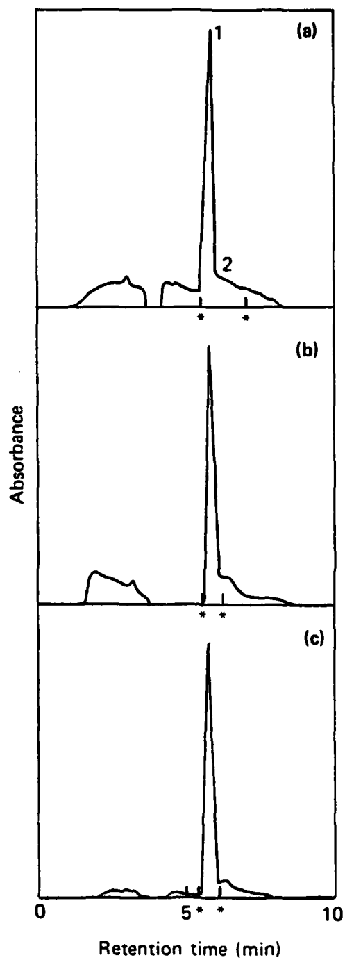
Fig. 17 HPLC chromatograms of DEGDN (28.6 mg/L) after 6(a), 24(b), and 48h (c) showing the stability of this compound in diluent water over time at 22°C. Note: The shoulder (peak 2) is due to a compound in the diluent water which absorbs at 215 nm. ** show where integrator began and ended integration of DEGDN peak.
