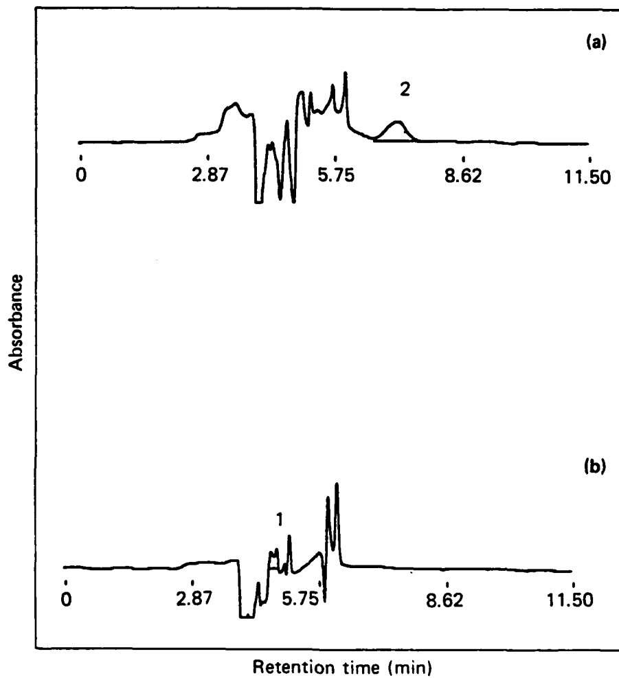
Fig. 7 Comparison of HPLC chromatograms of dissolved Technical solvent yellow 33 and control diluent water: (a) Technical solvent yellow 33 (yellow 33 component present at approximately 0.17 mg/L- peak 2), (b) diluent water only. Note the absence of peak 2.
