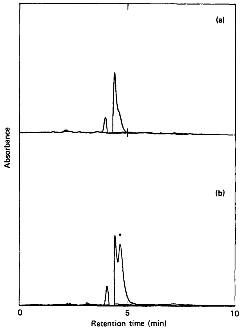
Fig. 15 Difference in absorbance of DEGDN at 254 nm (a) and 215 nm (b) for the same sample (28.6 mg DEGDN/L ethanol). The mobile phase was 15% DI H 2 O : 85% MEOH. Note: The retention time is 4.772 min and the DEGDN appears as a shoulder peak at 254 nm while a distinct peak (*) is visible at 215 nm. The injection volume was 5 \mu L.
