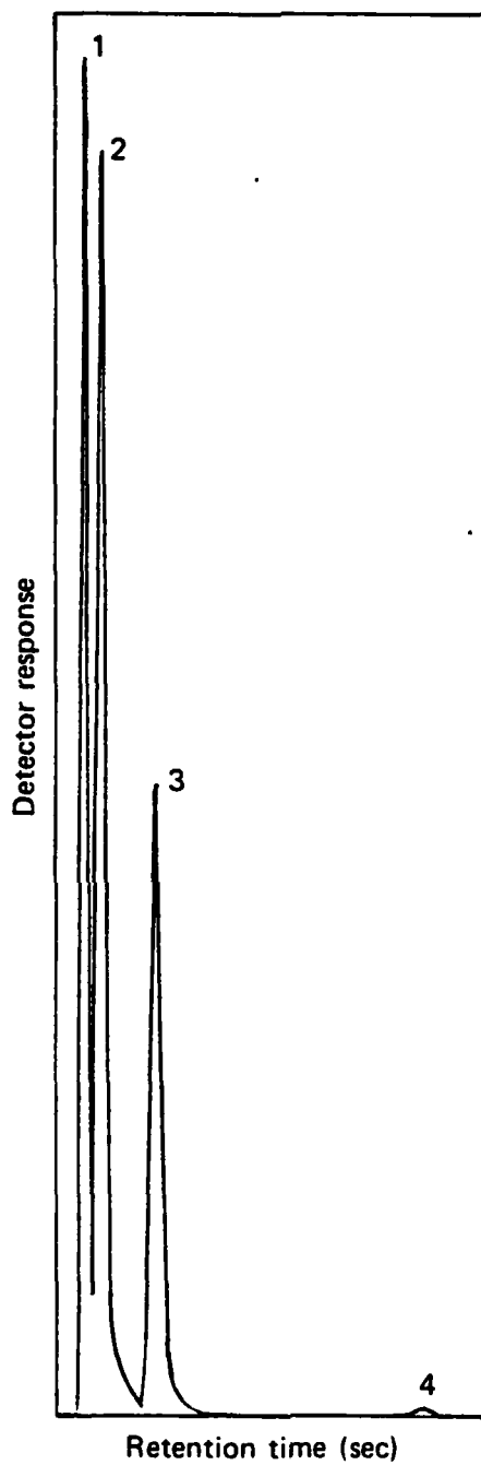
Fig. 13 Sample chromatogram of the four chlorinated organics in the synthetic-HC combustion products mixture following pentane extraction from diluent water (5 mL pentane : 50 mL water). This sample represents quantities of each compound after 24 h of mixing. Attenuation = 200: (1) \text{CCl}_4 ; (2) \text{C}_2\text{Cl}_4 ; (3) \text{C}_2\text{Cl}_6 ; (4) \text{C}_6\text{Cl}_6 (very close to detection limit).
