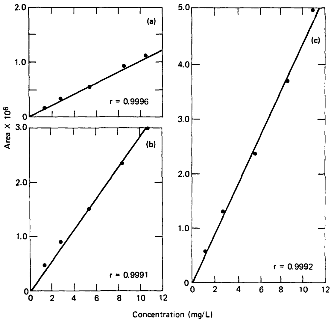
Fig. 3 The linear correlation between area of absorbance (254 nm) and concentration using the Waters HPLC; (a) Technical solvent green 3 - yellow component, (b) Technical solvent green 3 - green component, (c) Lovelace purified solvent green 3.
