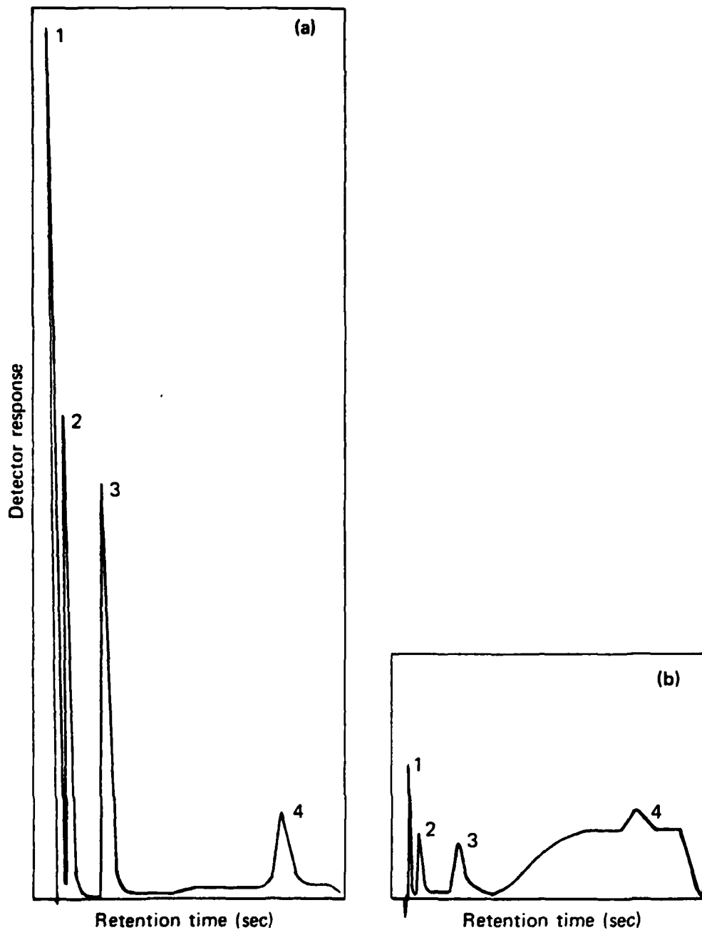
Fig. 10 Chromatograms from Tracor GC of 1 \mu L injection of GC standard for the organochlorine compounds in the synthetic-HC smoke combustion products mixture: (a) 3.0 mg/L, attenuation = 100; (b) 0.1 mg/L, attenuation = 10. Compounds (retention time, sec): (1) \text{CCl}_4 (57); (2) \text{C}_2\text{Cl}_4 (85); (3) \text{C}_2\text{Cl}_6 (190); (4) \text{C}_6\text{Cl}_6 (670).
