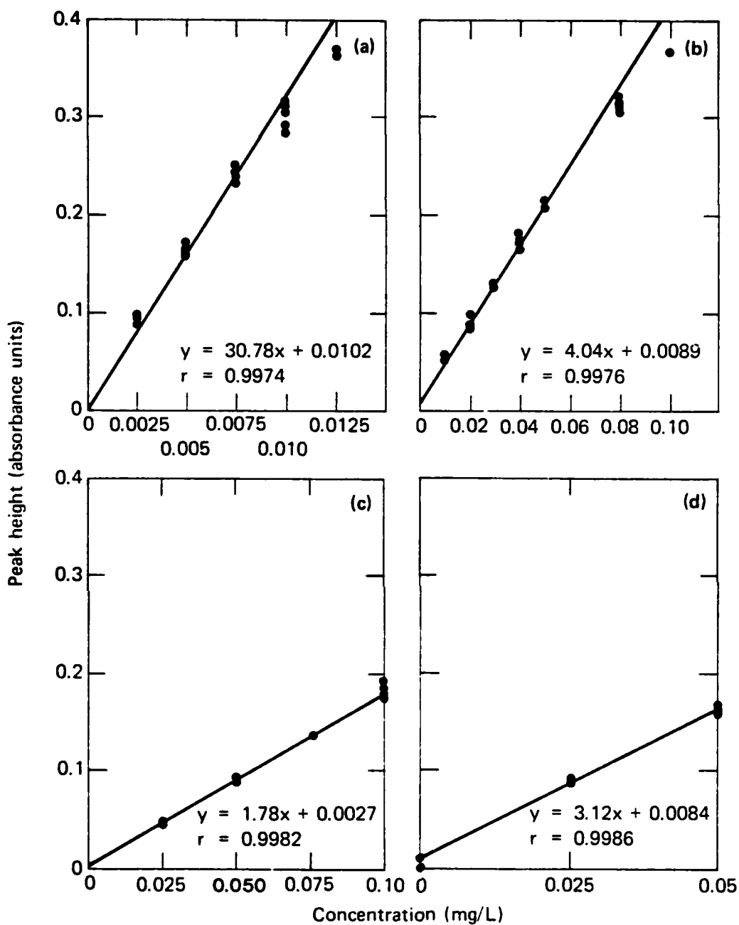
Fig. 11 The linear correlation between peak height (absorbance units) and concentration for the metals in the synthetic-HC smoke combustion products mixture using graphite furnace atomic absorption spectrophotometry: (a) cadmium; (b) aluminum; (c) lead; (d) arsenic.
