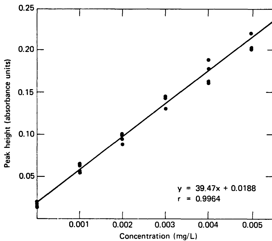
Fig. 12 The linear correlation between peak height (absorbance units) and concentration for arsenic analyzed by the gaseous hydride atomic absorption spectrophotometric method.
