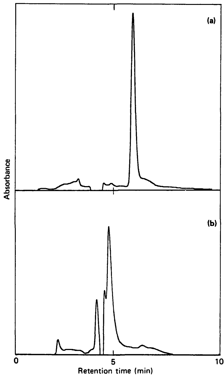
Fig. 14 Difference in retention time for DEGDN when using a 30% DI H 2 O: 70% MEOH mobile phase (a) (RT = 5.855 min) versus a 15% DI H 2 O: 85% MEOH mobile phase (b) (RT = 4.742 min). DEGDN concentration was 286 mg/L diluent water. Solvent front occurs from 4.123 - 4.502 min.
