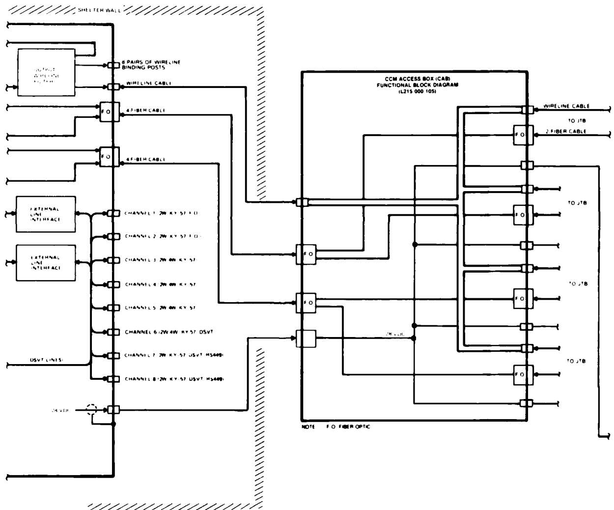
Figure 1. Communications Control System (CCS) Functional Block Diagram Final Design Model Rev. 3, Continued
