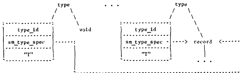
Figure 1: Incomplete Type
