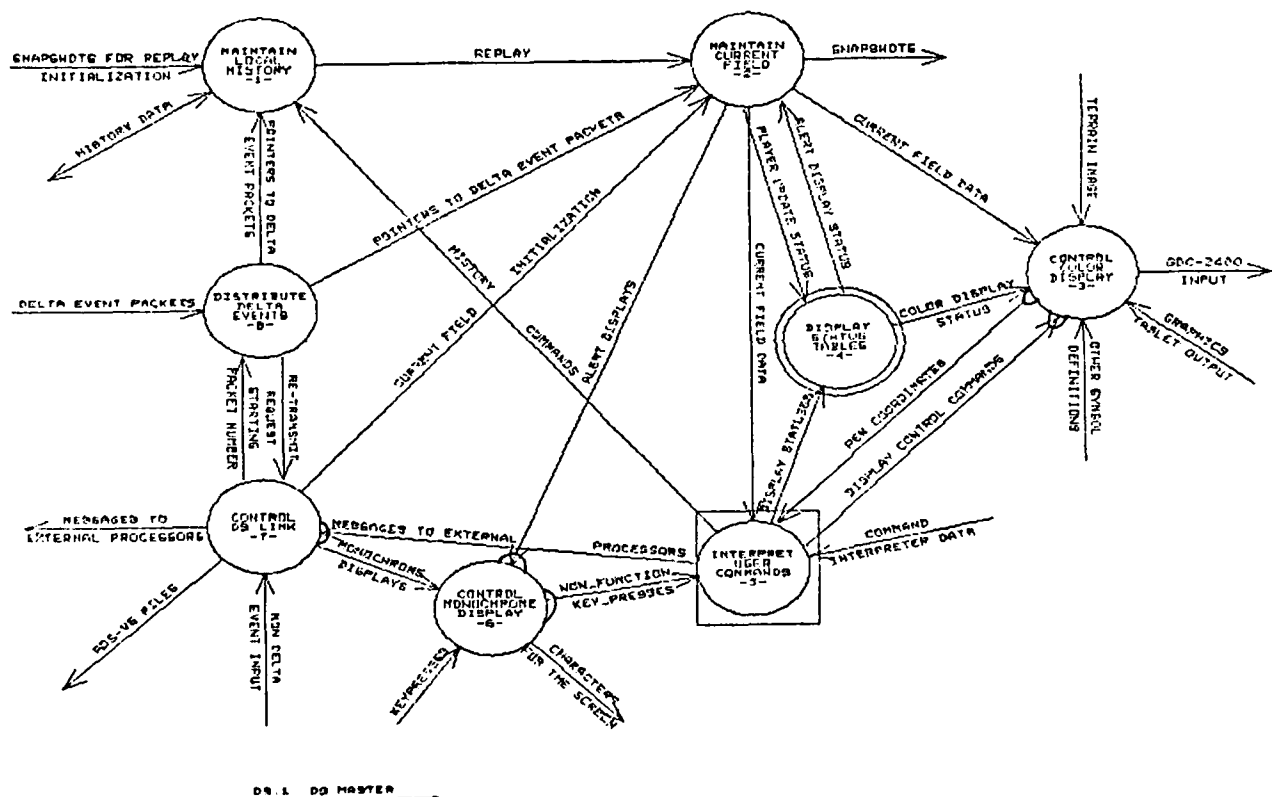
FIGURE 2: LEVEL 1 DATA FLOW DIAGRAMS FOR THE DISPLAY PROCESSOR
