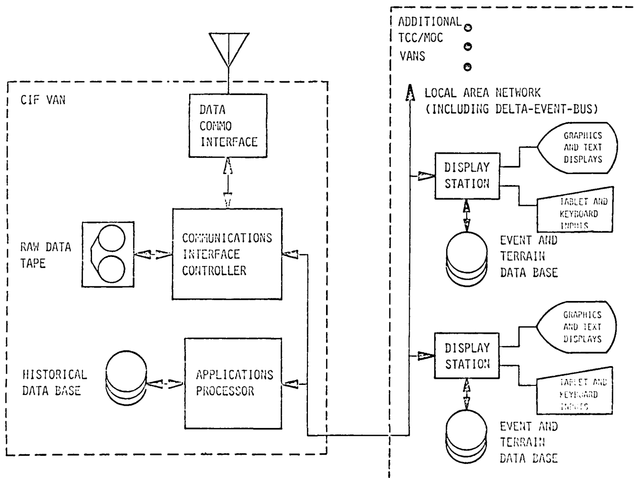
FIGURE 1: COMMAND AND CONTROL HARDWARE ARCHITECTURE
