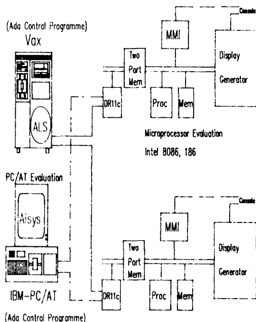
Figure 3 - Platform 2 Sonar Demonstrator
