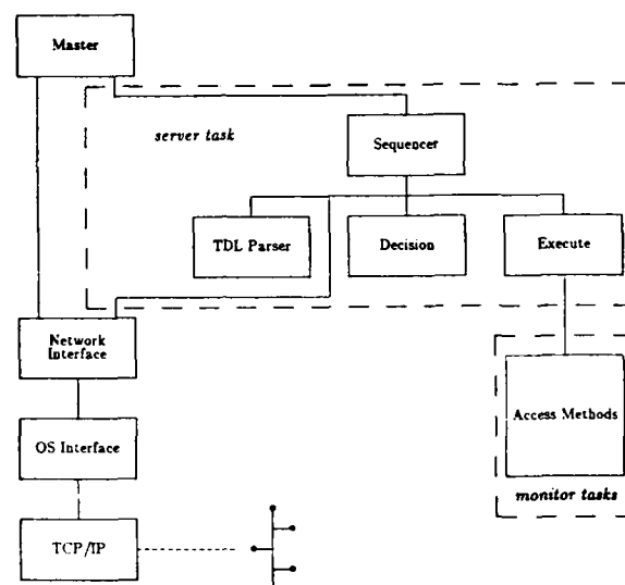
Figure 4. General Back End Design.
