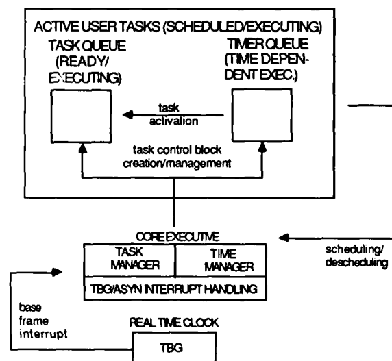
FIGURE 2. FORTRAN/ASSEMBLY EXECUTIVE FUNCTIONAL SCHEMATIC
