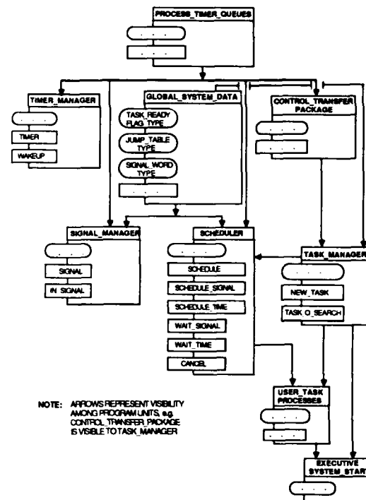
FIGURE 5. HIGH LEVEL RTOD SCHEMATIC "BARE MACHINE APPROACH"
