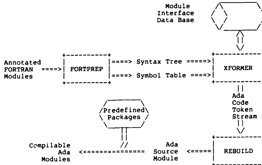
Figure 1. A Translation System based on the Present Approach
