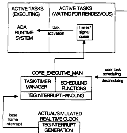
FIGURE 6. Ada PRIORITY DRIVEN EXECUTIVE FUNCTIONAL SCHEMATIC
