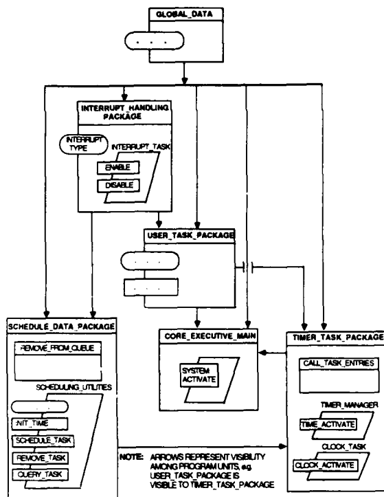
FIGURE 4. HIGH LEVEL RTOD SCHEMATIC EXECUTIVE WITH UNDERLYING RTS
