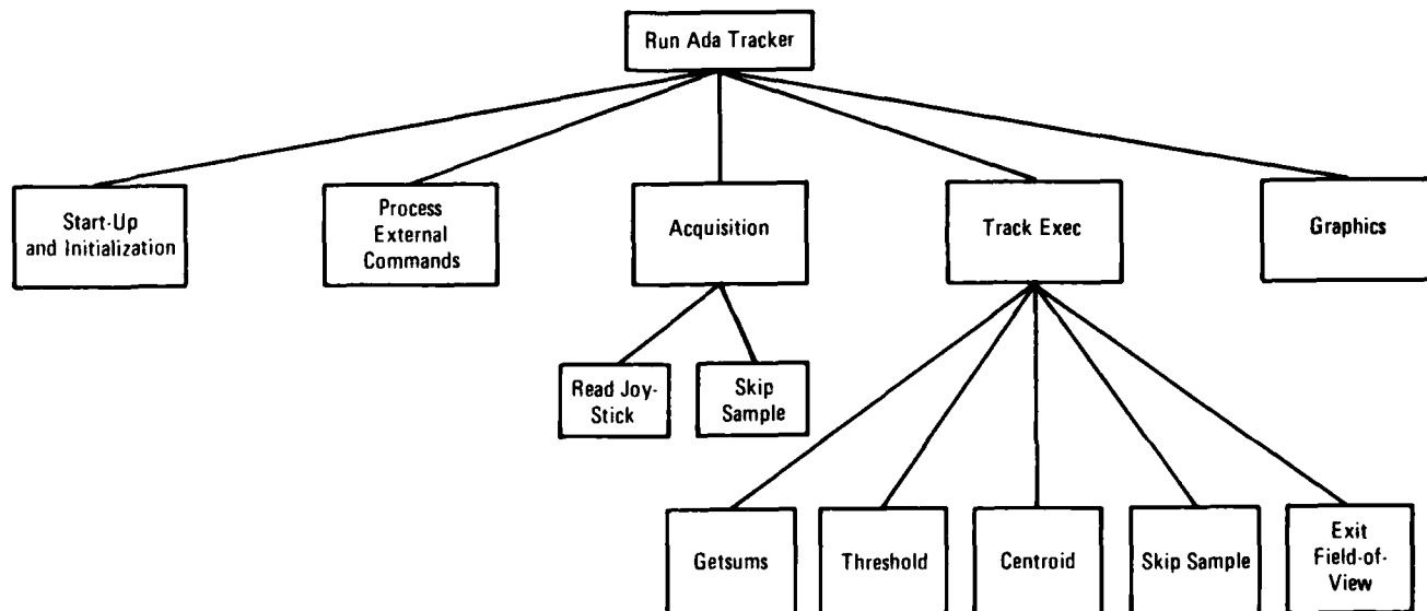
Figure 5. High Level Design
