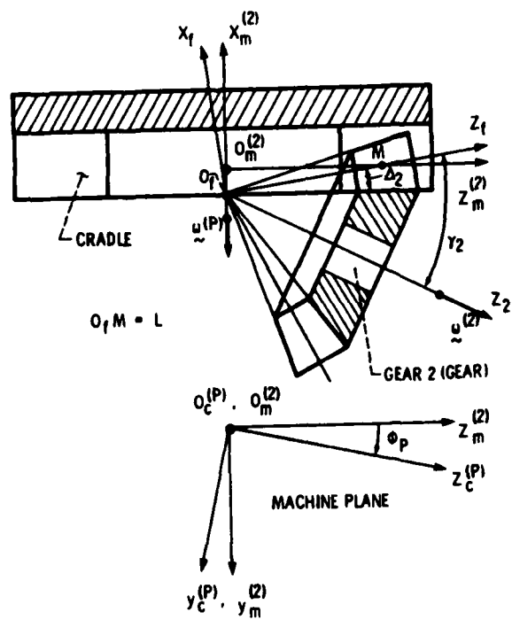
Figure 3. - Gear generation.
