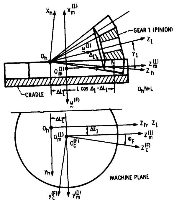
Figure 4. - Pinion generation.
