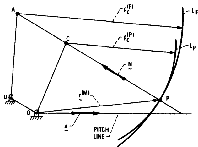
Figure 6. - Meshing in plane \pi .
