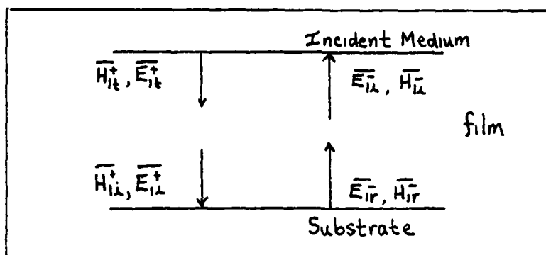
Fig. 24 \vec{H} and \vec{E} waves within the Film Thickness
