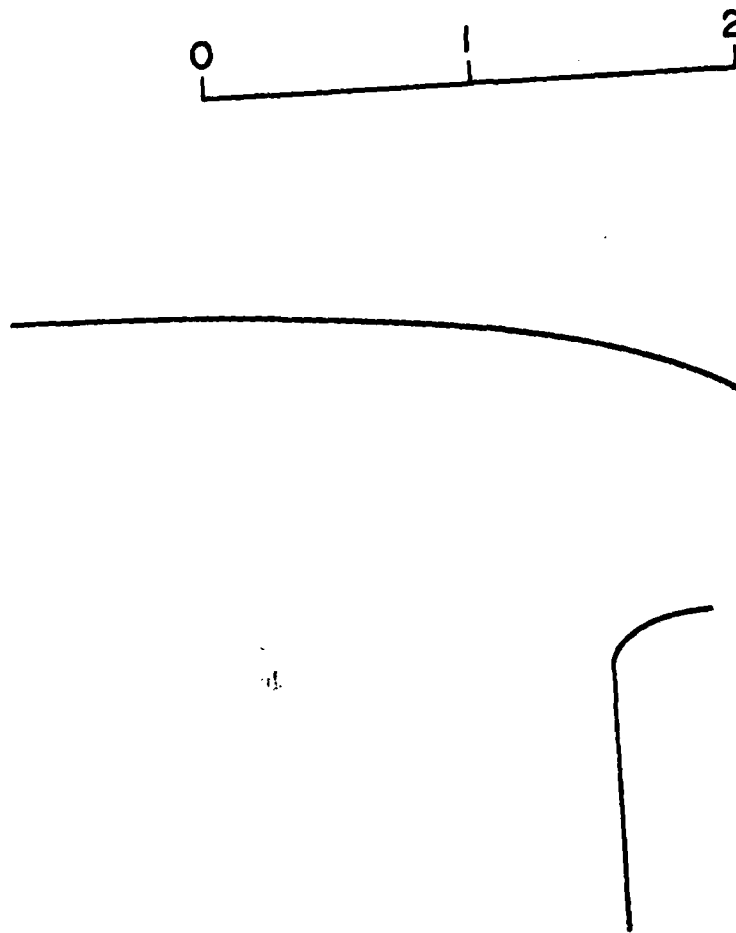
Figure 4: Computed free surface profile for the flow past a thin weir in an infinitely deep channel. The vertical scale is the same as the horizontal scale.
