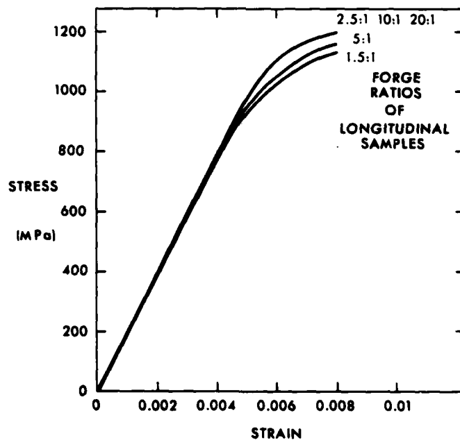
FIGURE 6. Stress-strain relationship for each forge ratio showing the different behaviour for two deformation ratios (1.5:1 and 5:1) which also displayed lower tensile and notch impact properties.
