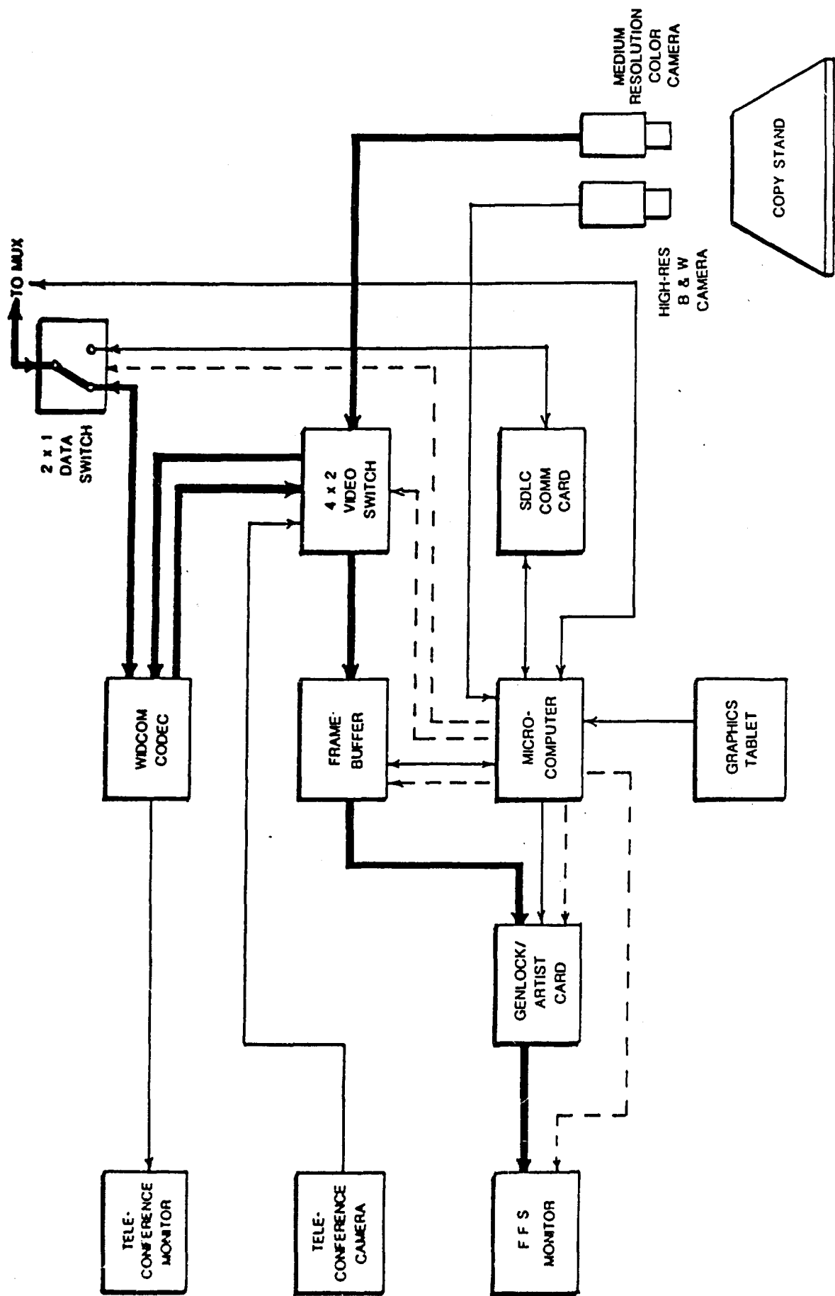
FIGURE 8 COLOR TRANSMISSION
