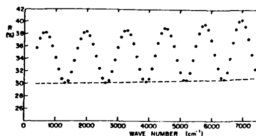
Fig. 2. Points are calculated reflection vs. frequency ( \text{cm}^{-1} ) for a single layer on a Si substrate as given in Fig. 1 with \sigma_D = 0 and k(\nu) = 0 . The R_D = 1.0 \mu\text{m} and the dispersion parameters are as follows: for amorphous Si, A_D = 7.03 , B_D = 2.64 \times 10^9 \text{ cm}^{-2} and \Omega_D = 18,860 \text{ cm}^{-1} ; for crystalline Si, A_S = 4.1476 ; B_S = 5.8875 \times 10^9 \text{ cm}^{-2} and \Omega_S = 27,973 \text{ cm}^{-1} . The smooth dashed curve is the reflectivity for crystalline Si.
