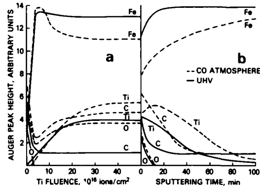
Fig. 7. (a) Auger peak height as a function of 150 keV \text{Ti}^+ fluence for implantation into a polished M50 substrate in ultra-high-vacuum conditions ( 1 \times 10^{-8} Torr) and with the target chamber backfilled to 7 \times 10^{-7} Torr with CO. (b) Auger depth profile of the implanted layers obtained by sputtering with 4.0 keV argon ions.
