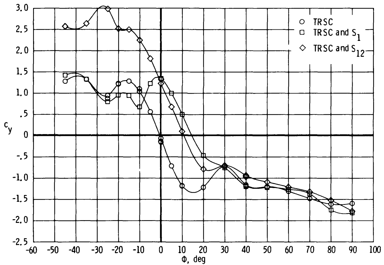
Figure 22. Comparison of drag and side-force variation with flow incidence of UH-60 shape with TRSC and spoilers S_1 and S_{12} .
