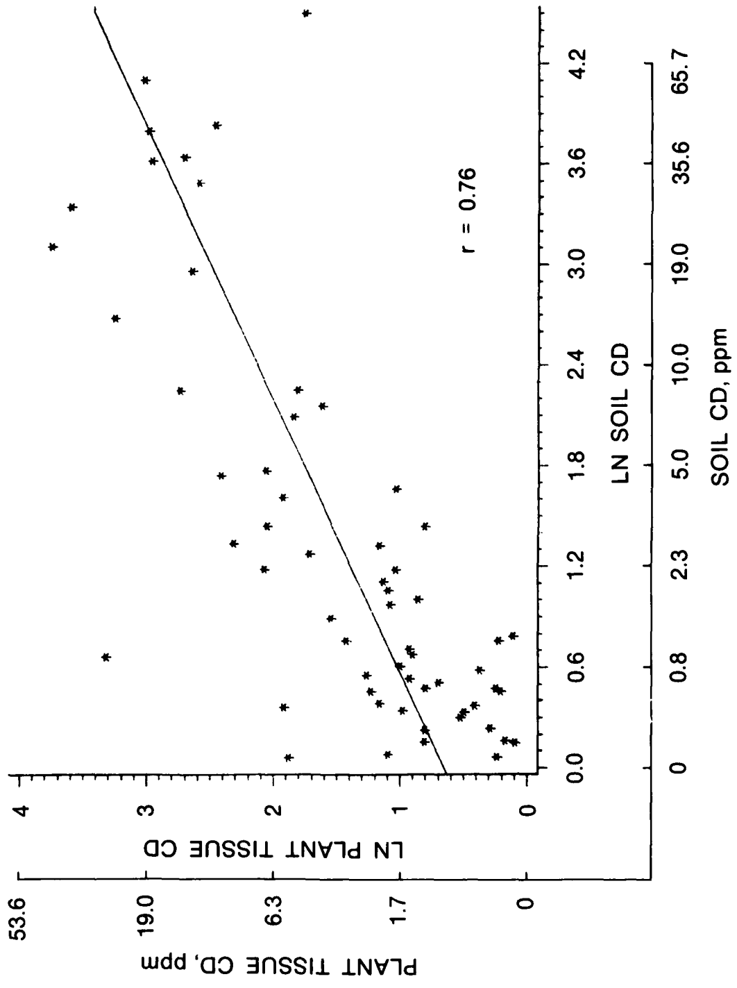
Figure 2-72. Regression of natural log (LN) plant tissue cadmium content on natural log (LN) soil cadmium content
