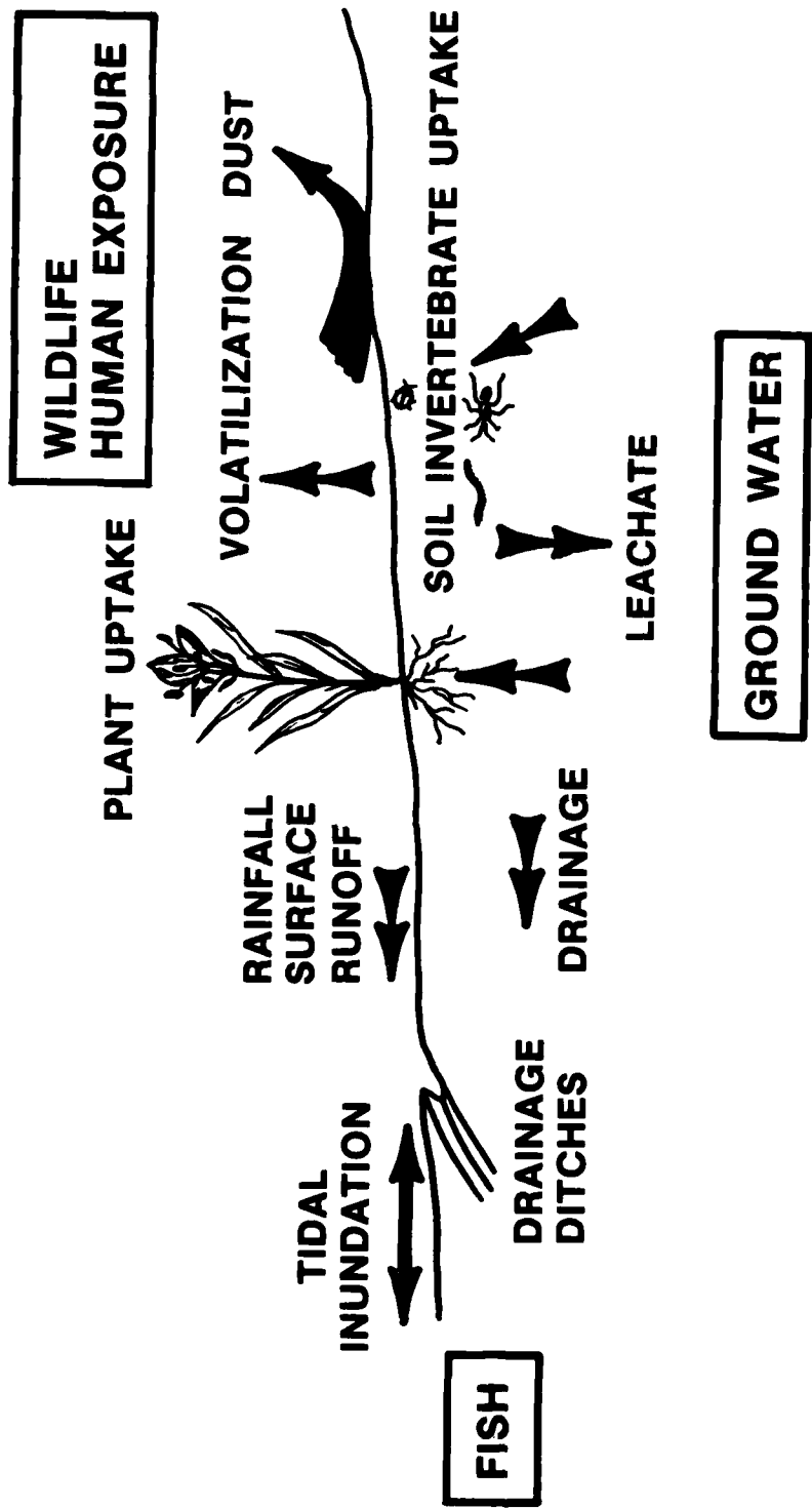
Figure 1-3. Pathways for contaminant mobility
