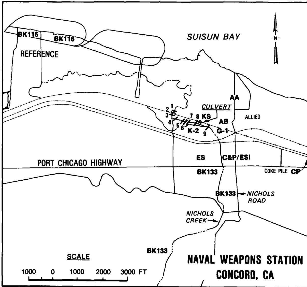
Figure 2-98. Cross-section locations used for HEC-2 analysis
