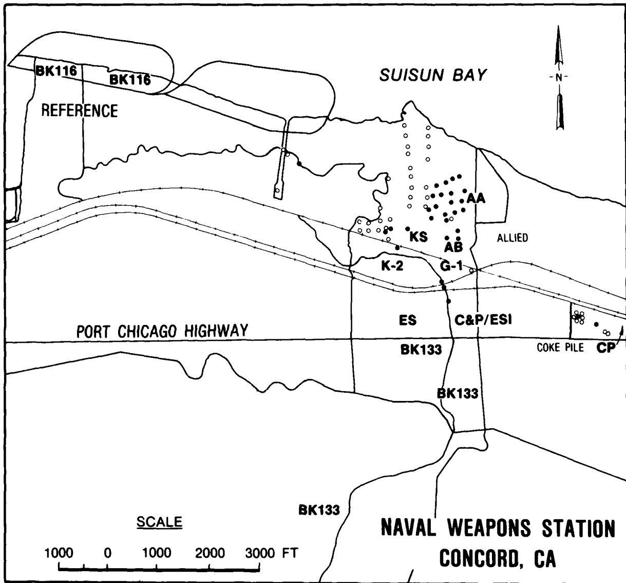
Figure 2-76. Distribution of earthworm arsenic content in excess of FDA level, 10 mg/kg. Soil circles were WES collected samples, open circles were Brown and Caldwell collected samples
