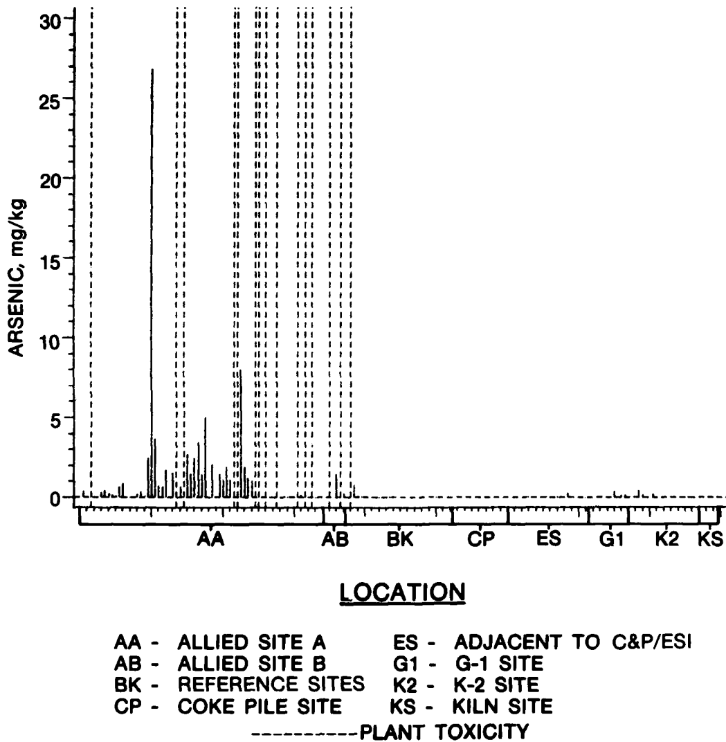
Figure 2-34. Flooded plant bioassay tissue arsenic content and plant toxicity
