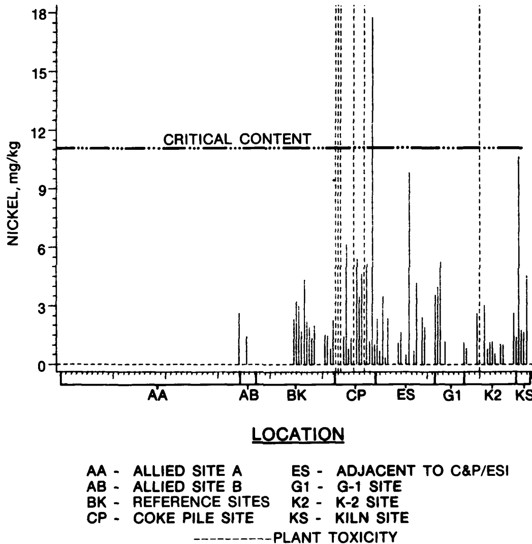
Figure 2-49. Upland plant bioassay tissue nickel content and plant toxicity
