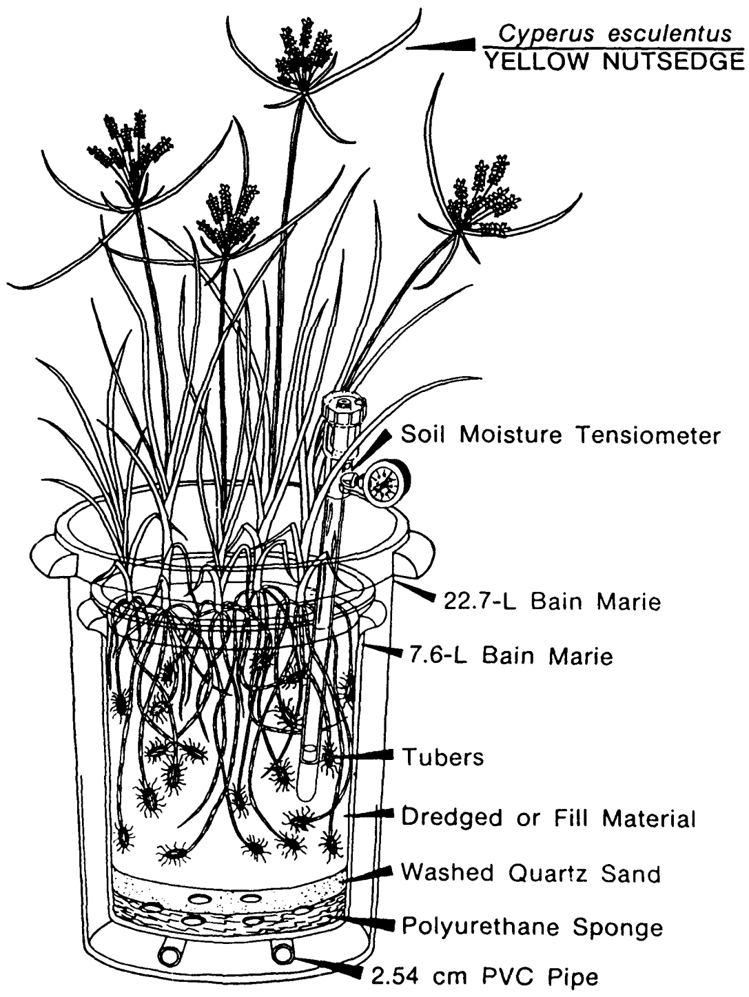
Figure 2-32. Plant bioassay apparatus
