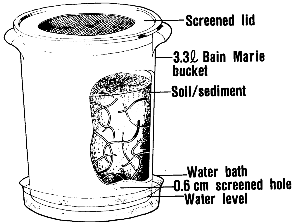
Figure 2-50. Earthworm bioassay apparatus
