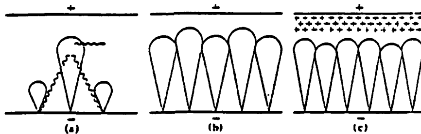
(c.) Townsend Mechanism-breakdown by Series of Avalanches.
