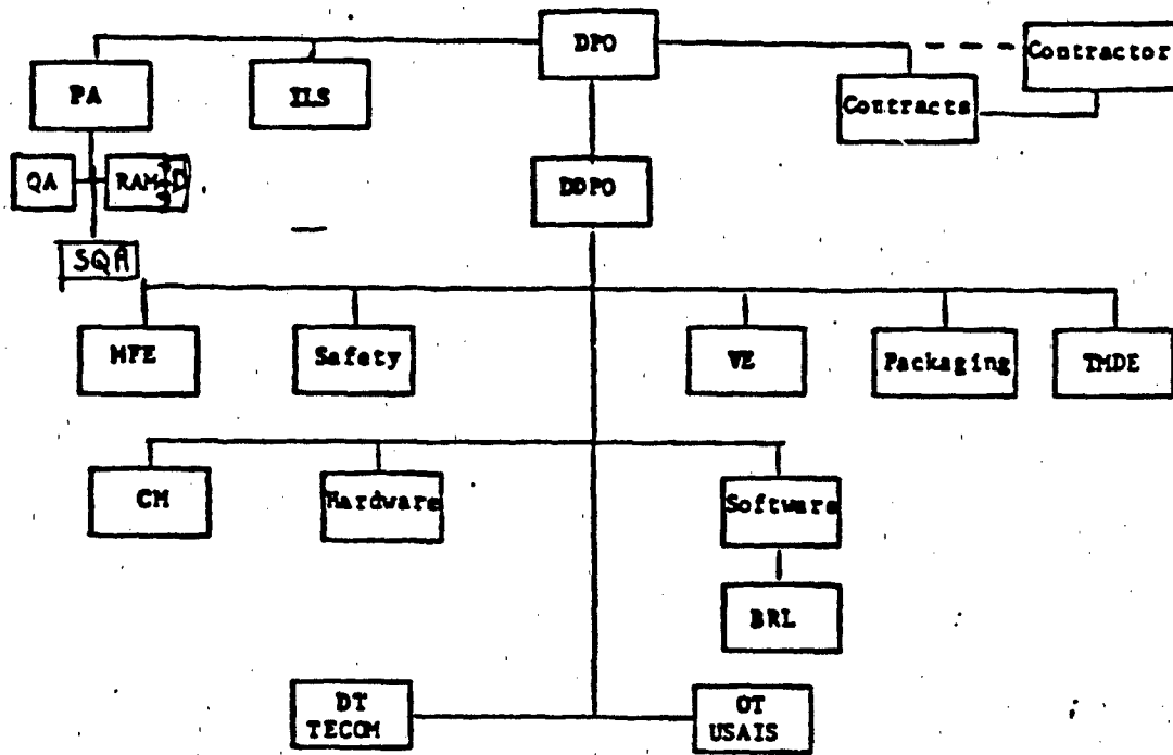
Figure 4.1a Program Management
