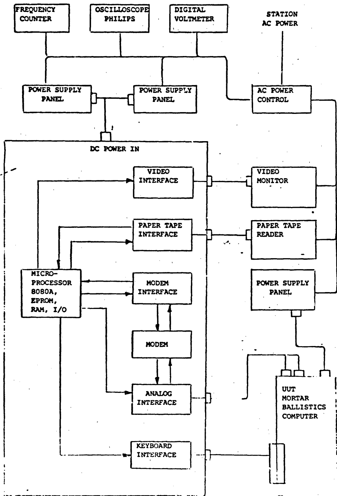
BLOCK DIAGRAM - MRC SYSTEM TEST CONSOLE
