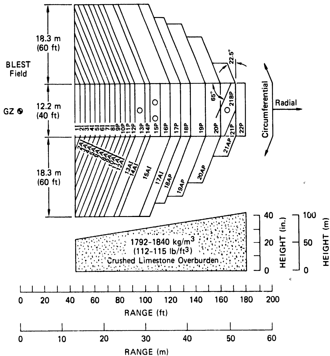
Figure 40. Layout of striptest and STP 3.5A HEST experiments.
