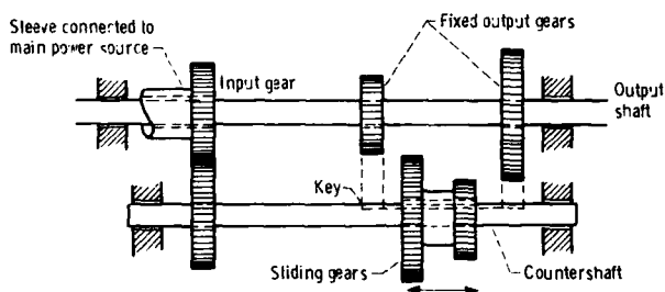
Figure 49.—Sliding gears.
