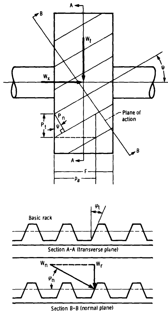
Figure 7.—Helical gear geometry. (Not to scale.).
