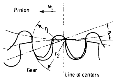
Figure 9.—Conformal tooth geometry.
