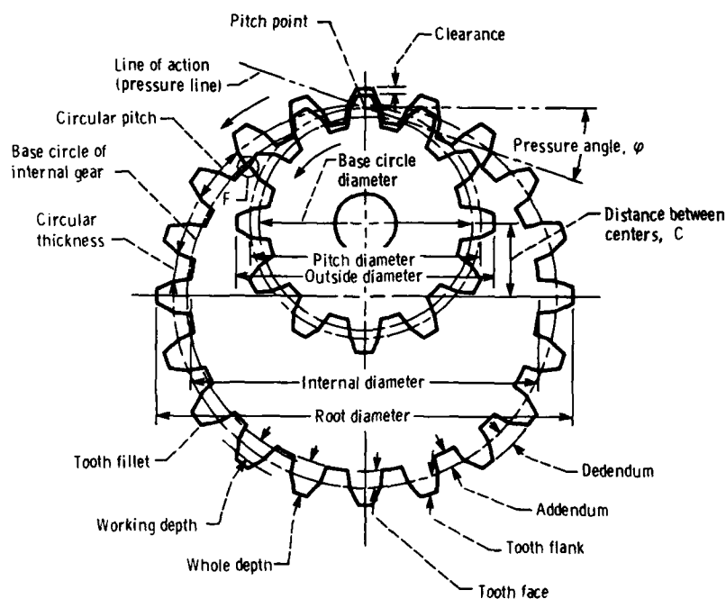
Figure 4.—Internal spur gear geometry.
