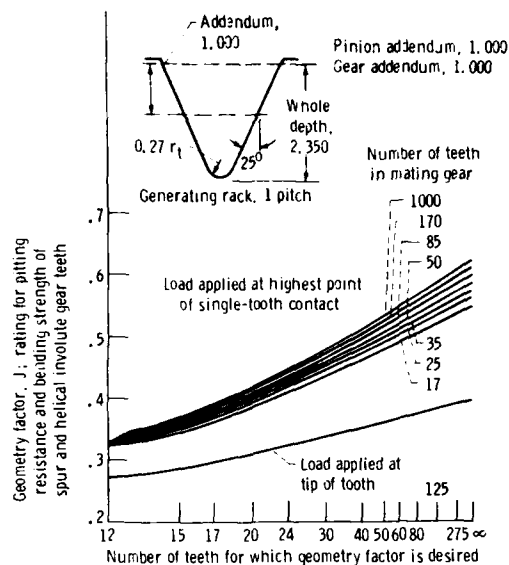
Figure 28.—Geometry factor for 25° spur gear. Standard addendum.
