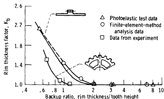
Figure 33.—Rim thickness factor.
