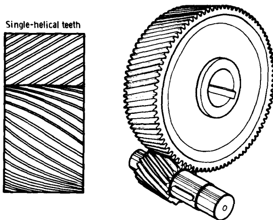
Figure 5.—Single-helical gear pair.
