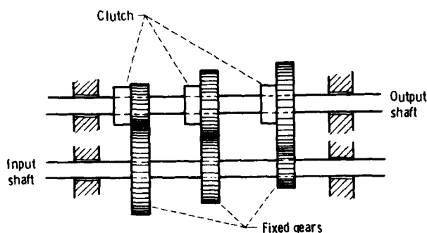
Figure 50.—Constant-mesh gears.
