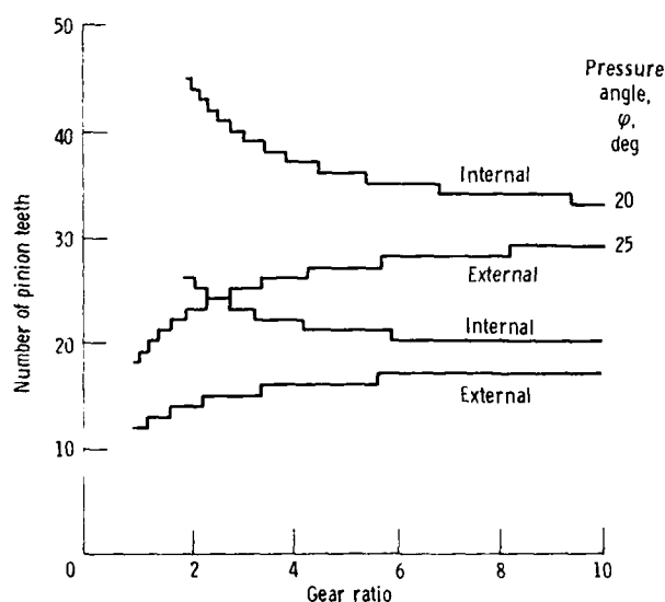
(a) Pressure angle, 20. (b) Pressure angle, 25.
