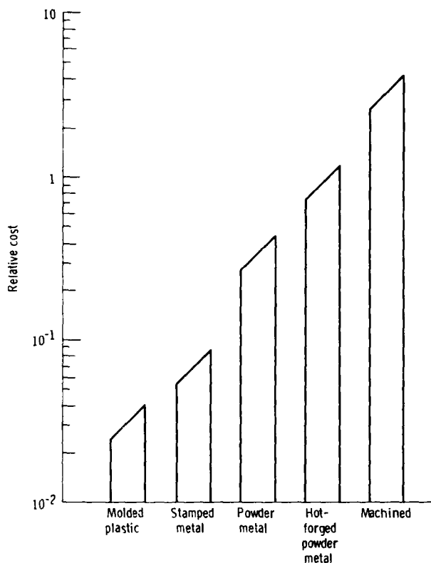
Figure 21.—Relative costs of gear materials.
