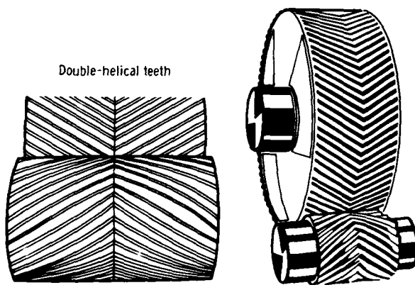
Figure 6.—Double-helical, or herringbone, gear pair.
