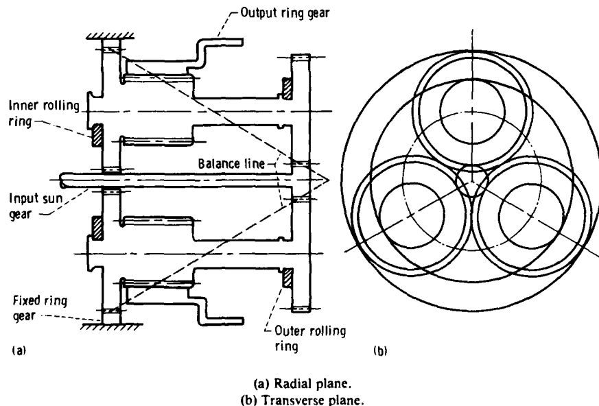
Figure 55.—373-kW (500-hp) bearingless planetary transmission.
