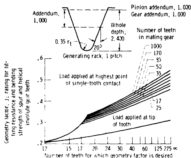
Figure 27.—Geometry factor for 20° spur gear. Standard addendum.
