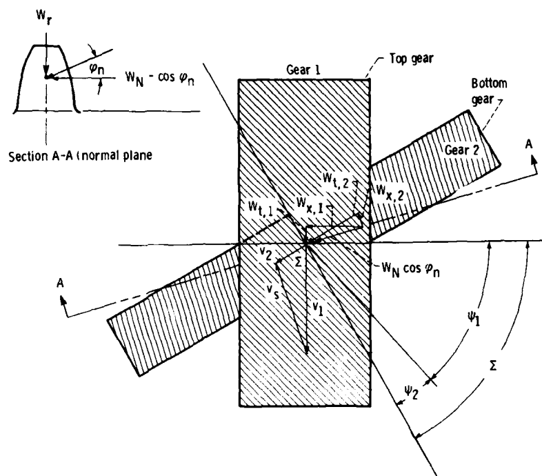
Figure 16.—Meshing crossed-helical gears showing relationship between helix angles, shaft angle, and load and velocity vectors.
