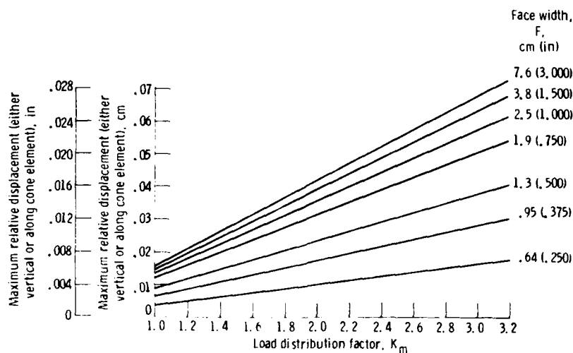
Figure 24.—Load distribution factor for bevel gears.
