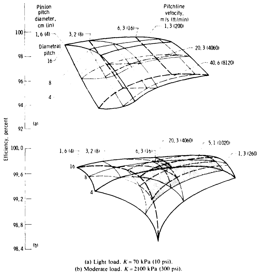
Figure 45.—Parametric study for light and moderate gear loads. Gearset parameters include gear ratio, 1; ratio of pinion face width to diameter 0.5; lubricant viscosity, 30 cP.
