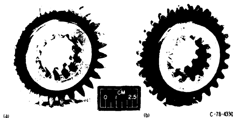
(a) High-contact-ratio gear with modified tooth profile. Contact ratio, 2.25. (b) Conventional involute gear. Contact ratio, 1.3.
