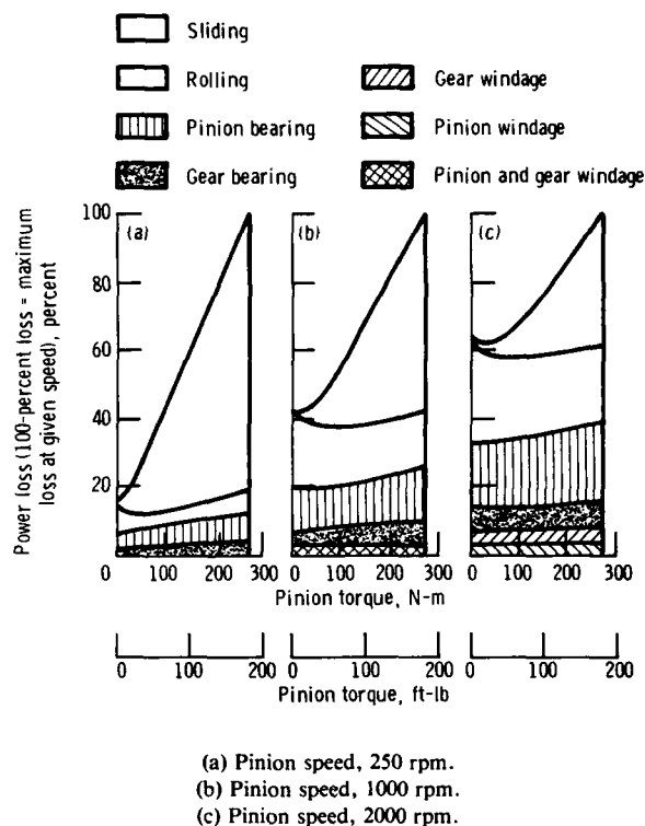
Figure 44.—Typical power loss breakdown for a gear system. Gearset parameters include pitch diameter, 15.2 cm; gear ratio, 1.66; diametral pitch, 8; ratio of pinion face width to diameter, 0.5; lubricant viscosity, 30 cP.
