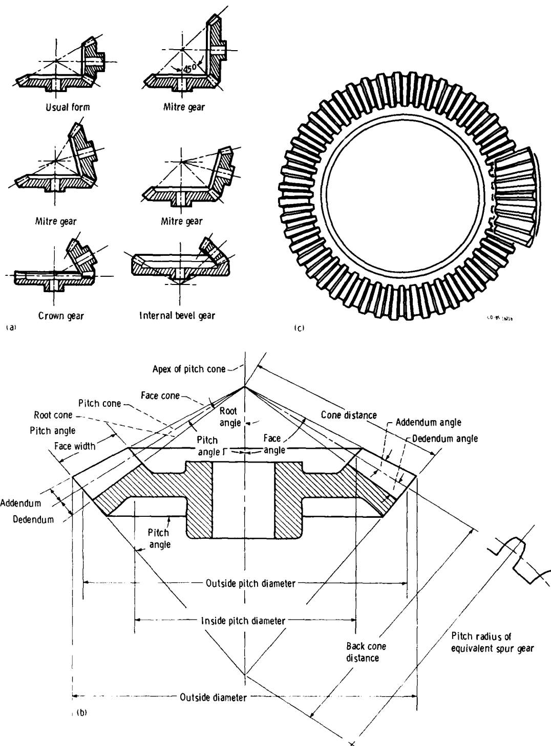
(a) Gear arrangements. (b) Gear terminology. (c) Gear pair.
