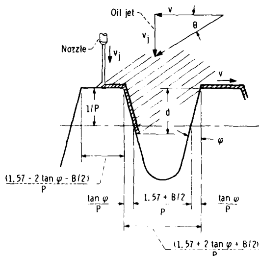
Figure 40.—Vectorial model for penetration depth.
