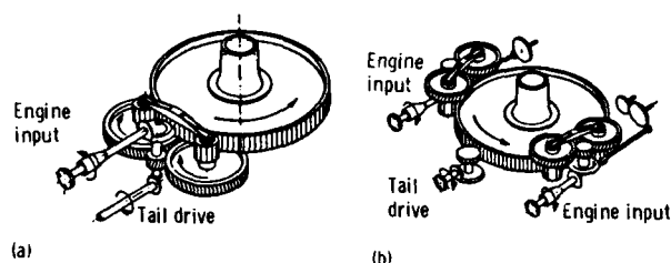
(a) Bevel gears. (b) Spur gears.
