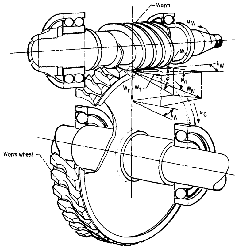
Figure 19.—Worm gearset showing load vectors.
