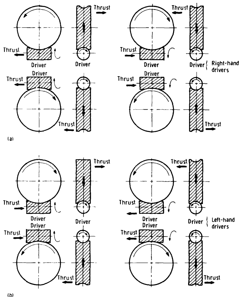
(a) Right-hand drivers. (b) Left-hand drivers.
