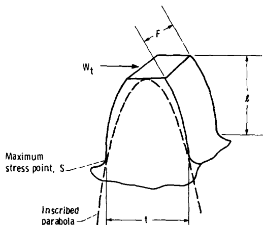
Figure 23.—Gear tooth load.
