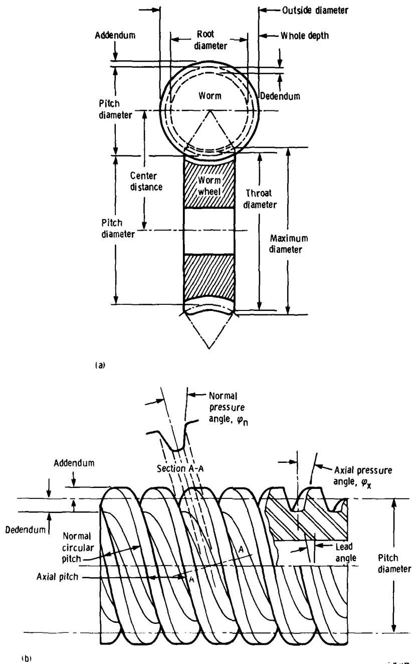
(a) Worm and wheel. (b) Worm.
