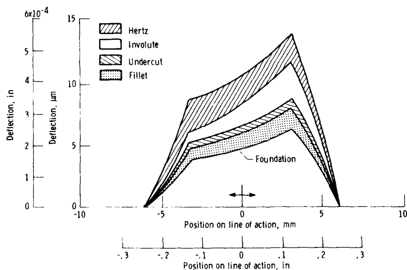
Figure 36.—Tooth deflection calculated by method of Cornell.
