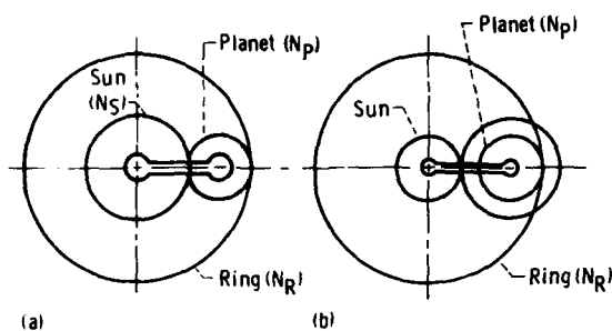
(a) Simple train. (b) Compound train, planet gears keyed to same shaft. Figure 54.—Epicyclic gear trains.
