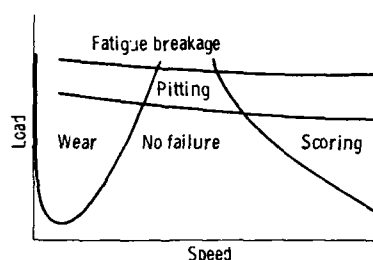
Figure 46.—Various failure regimes encountered by gear teeth.
