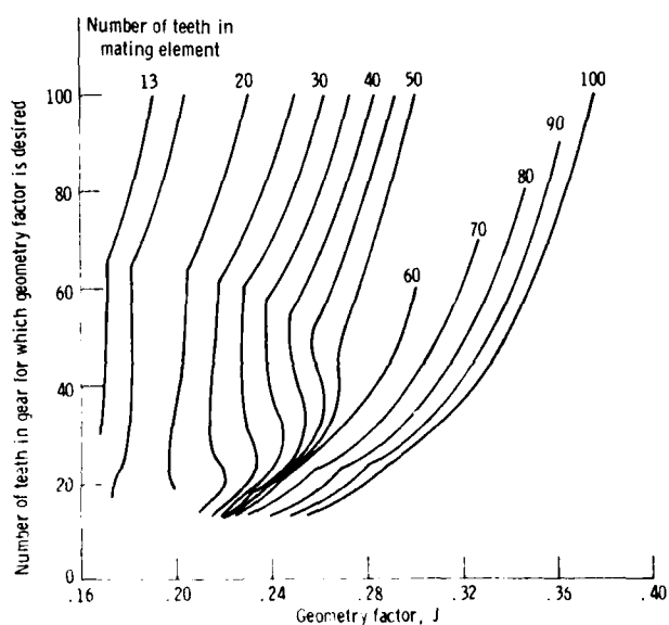
Figure 32.—Geometry factor for straight bevel gears with 20° pressure angle and 90° shaft angle.
