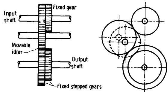
Figure 51.—Idler gear.
