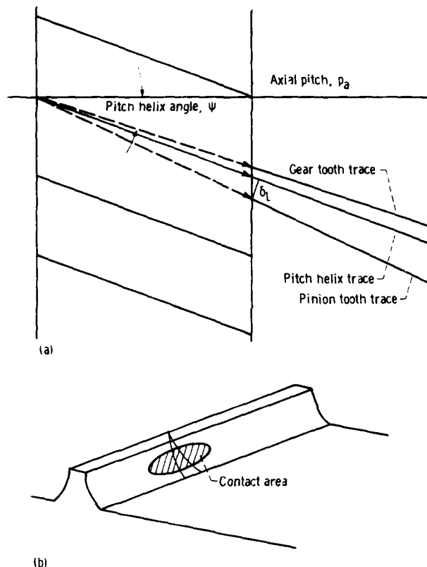
(a) Sliding components in rolling direction. (b) Relative sliding velocities in contact area.
