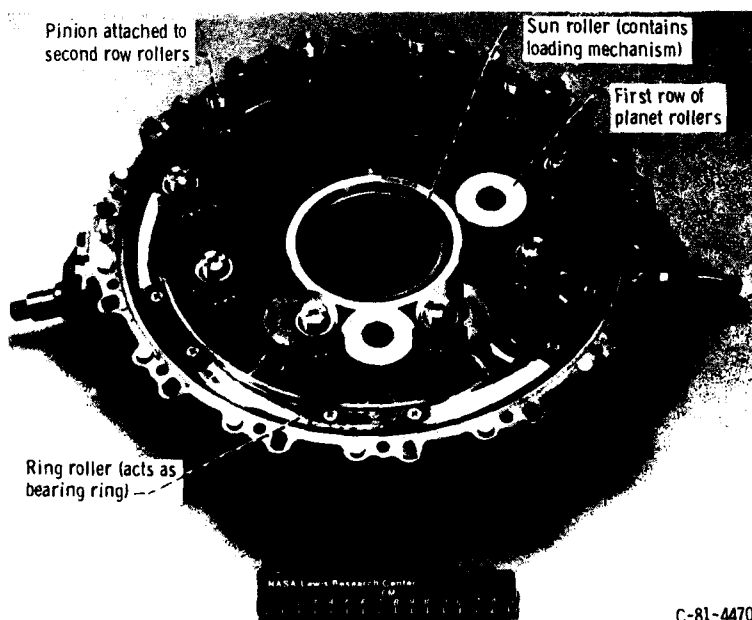
Figure 56.—373-kW (500-hp) hybrid transmission.
