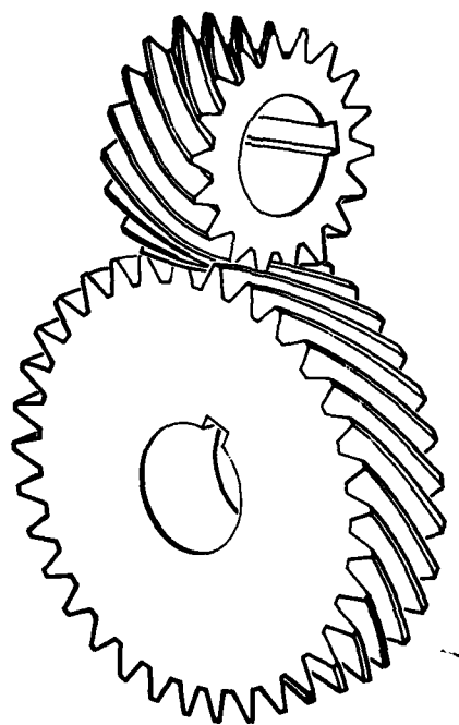
Figure 15.—Crossed-helical gear.
