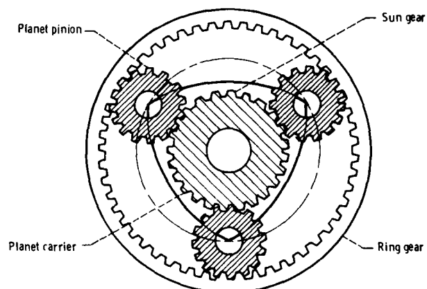
Figure 52.—Planetary gears. Epicyclic gears.
